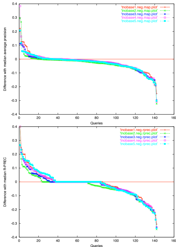
Figure 2: Difference of TNO produced MAP and R-PREC values with the TREC reference values for negative queries (queries sorted by descending performance).
