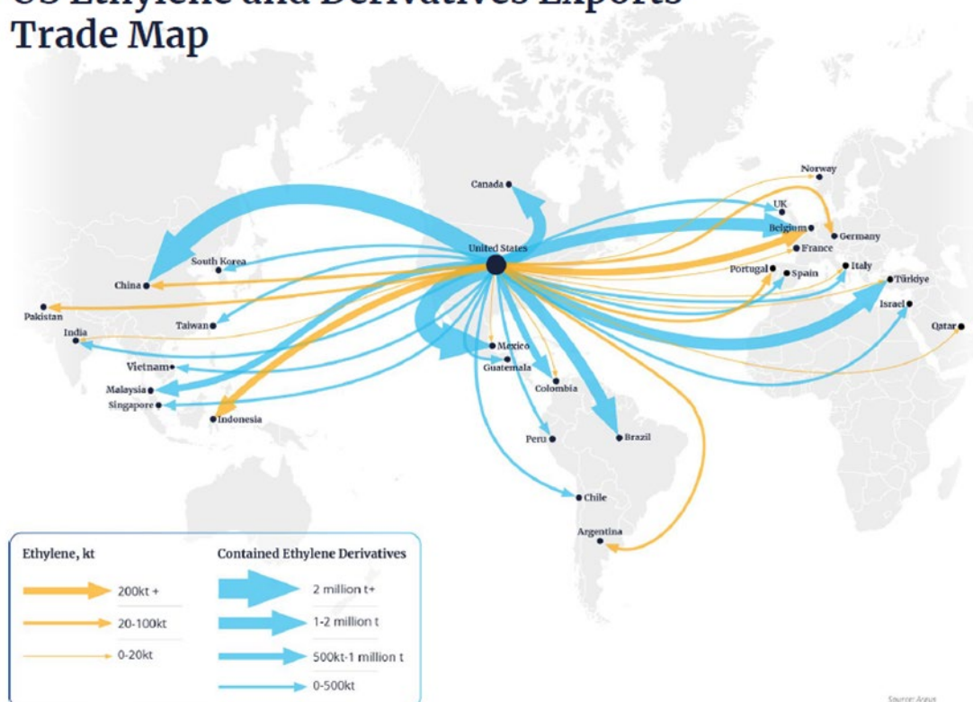
Figure 2.1: US ethylene and ethylene derivatives exports trade map, Argus, March 2026. (For reference: the production of ethylene by the countries of the Trilateral Chemical Region in 2019 was around 10 million tonnes).
