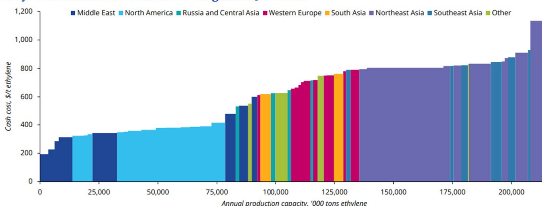
Figure 2.7: Argus-modelled 2025 forecast cost curve as of May 2025, Argus insight paper May 2025, https://www.argusmedia.com/en/news-and-insights/market-insight-papers/global-ethylene-market-costs-tariffs-volatility .
