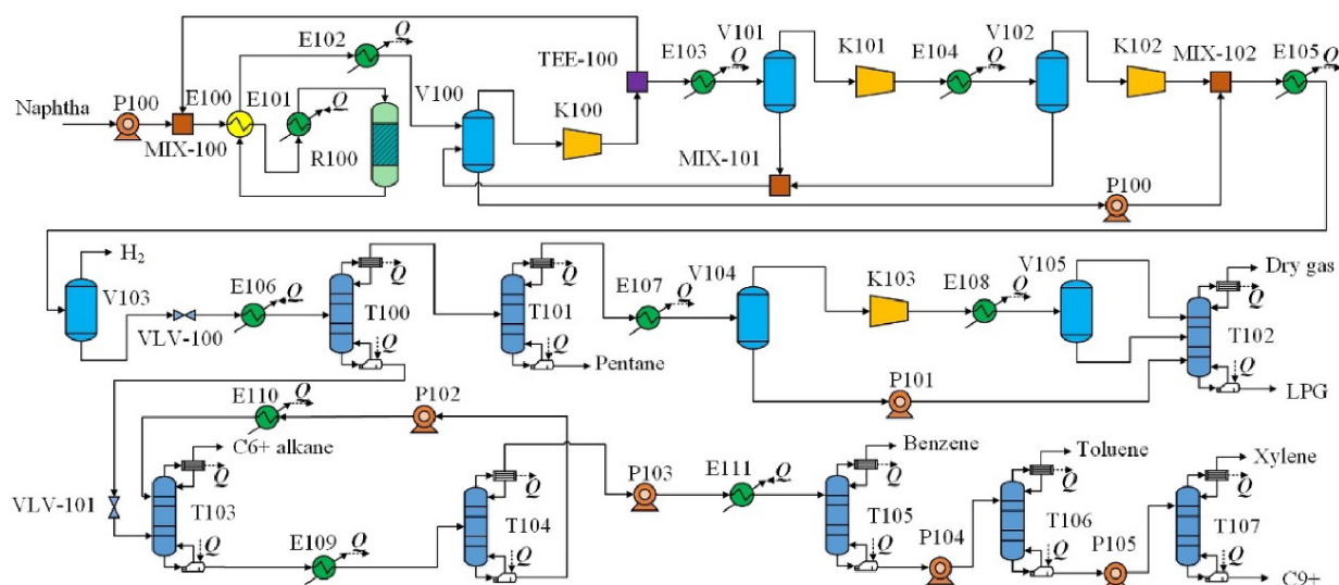
Figure D.4: Process flow diagram of naphtha catalytic reformer process 5
