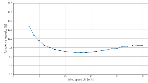
Figure 4.5: Turbulence intensity at 91 m
