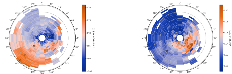
Figure A.68: Wind shear and veer as function of wind speed and direction for 2023
