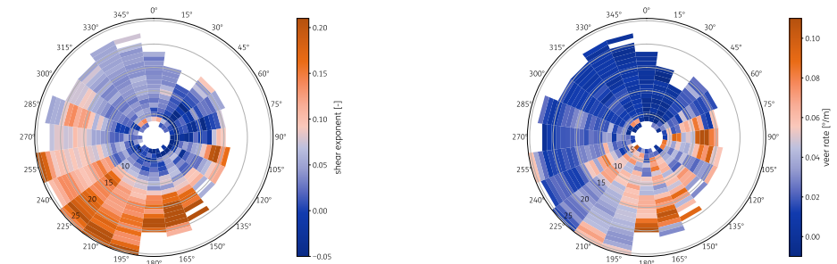
Figure A.64: Wind shear and veer as function of wind speed and direction for 2019
