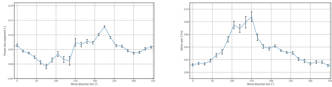
Figure A.56: Wind shear and veer as function of wind direction for 2021
