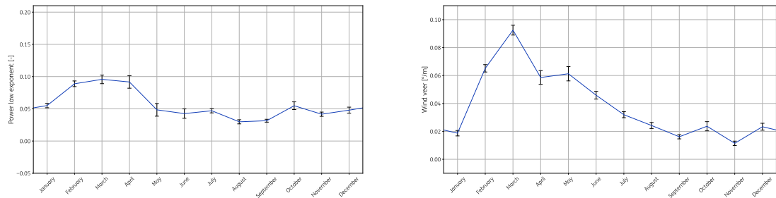
Figure A.22: Wind shear and veer as function of the month-of-year for 2017
