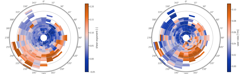
Figure A.62: Wind shear and veer as function of wind speed and direction for 2017
