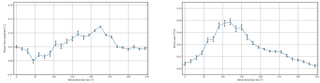
Figure A.59: Wind shear and veer as function of wind direction for 2024
