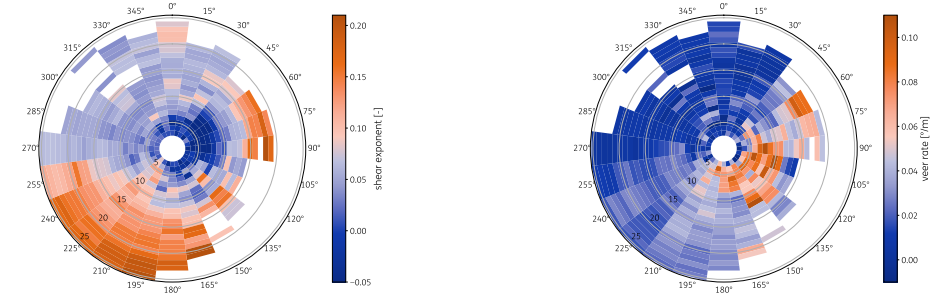
Figure A.65: Wind shear and veer as function of wind speed and direction for 2020
