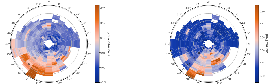
Figure A.63: Wind shear and veer as function of wind speed and direction for 2018
