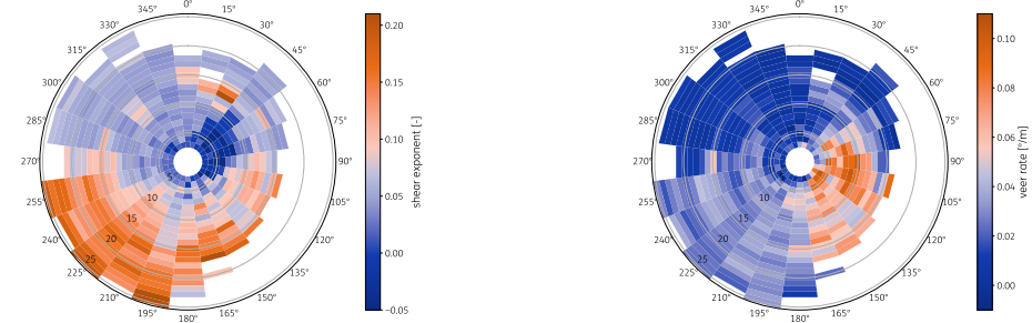
Figure A.69: Wind shear and veer as function of wind speed and direction for 2024
