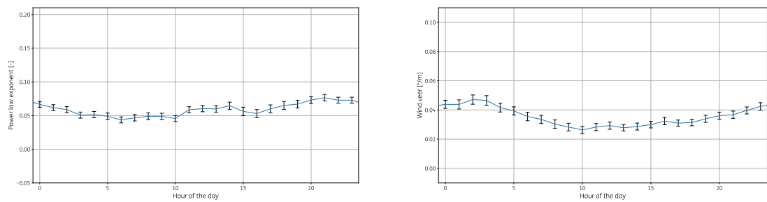
Figure A.40: Wind shear and veer as function the hour-of-day for 2025
