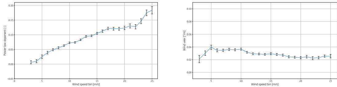
Figure A.49: Wind shear and veer as function of wind speed for 2024
