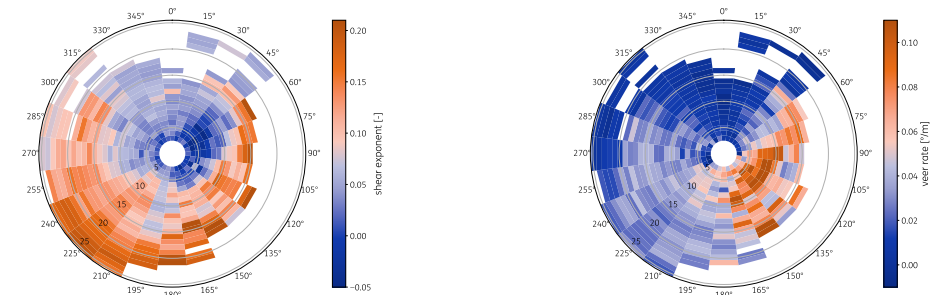
Figure A.67: Wind shear and veer as function of wind speed and direction for 2022
