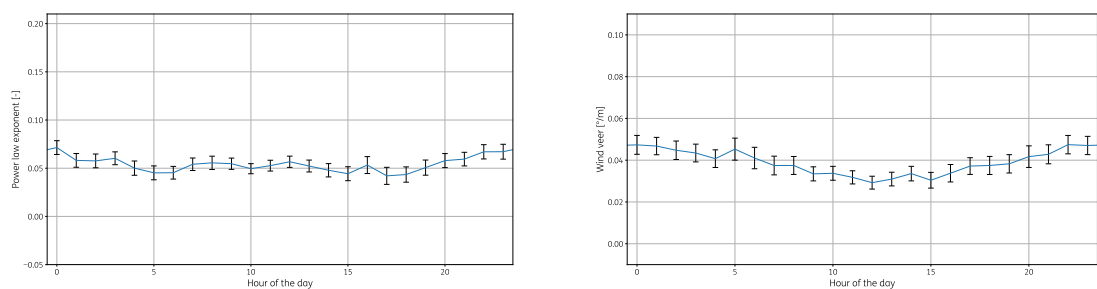
Figure A.32: Wind shear and veer as function the hour-of-day for 2017
