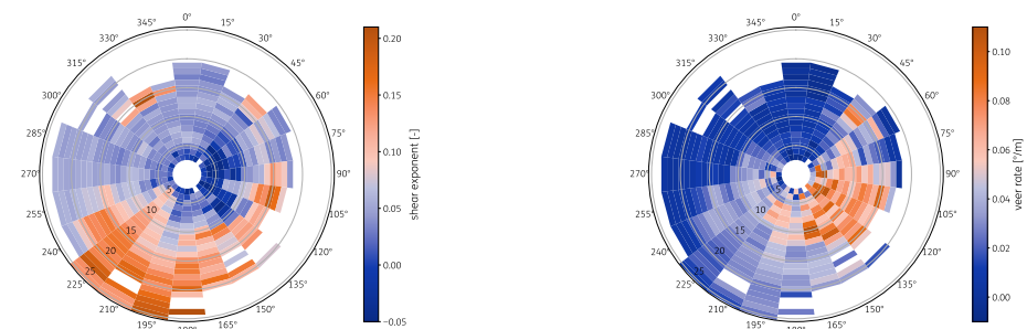
Figure A.70: Wind shear and veer as function of wind speed and direction for 2025
