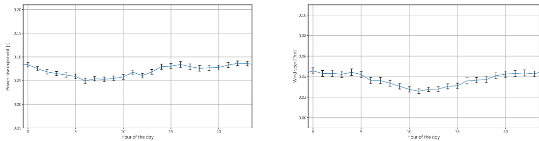
Figure A.37: Wind shear and veer as function the hour-of-day for 2022
