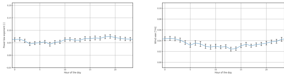
Figure A.34: Wind shear and veer as function the hour-of-day for 2019
