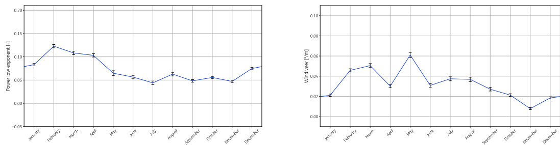
Figure A.29: Wind shear and veer as function of the month-of-year for 2024
