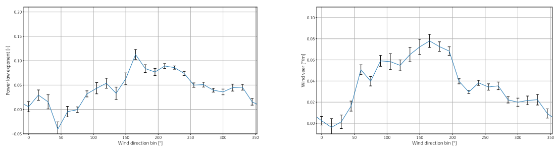
Figure A.52: Wind shear and veer as function of wind direction for 2017
