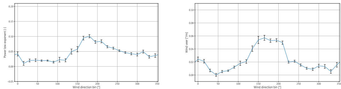
Figure A.53: Wind shear and veer as function of wind direction for 2018
