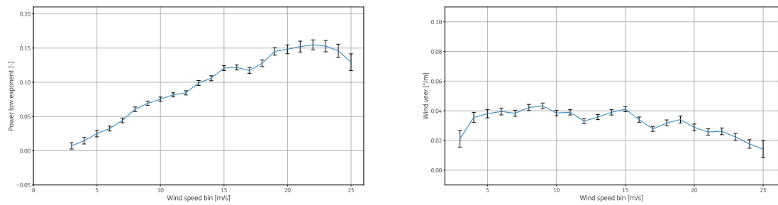
Figure A.47: Wind shear and veer as function of wind speed for 2022
