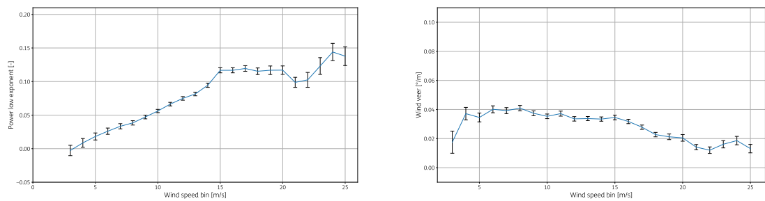
Figure A.50: Wind shear and veer as function of wind speed for 2025
