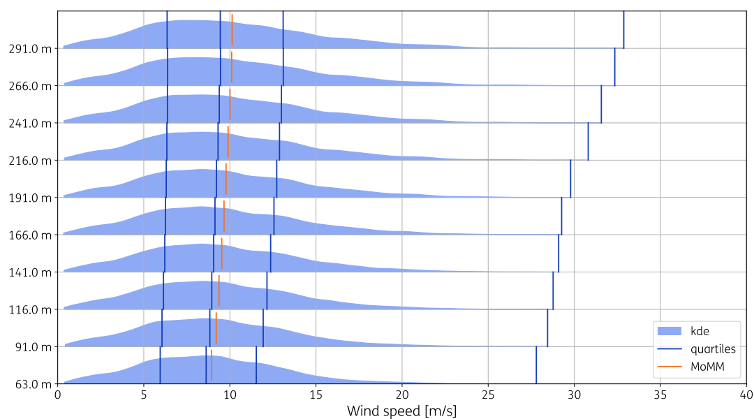
Figure A.20: Wind speed distributions for 2025
