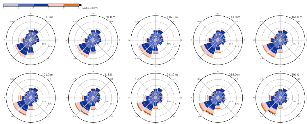
Figure A.10: Wind roses for 2025
