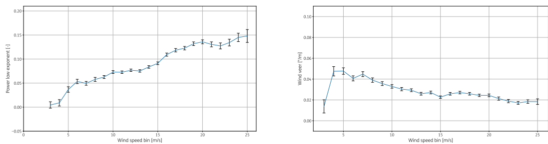
Figure A.48: Wind shear and veer as function of wind speed for 2023
