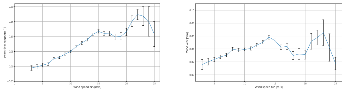
Figure A.42: Wind shear and veer as function of wind speed for 2017
