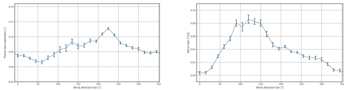
Figure A.57: Wind shear and veer as function of wind direction for 2022
