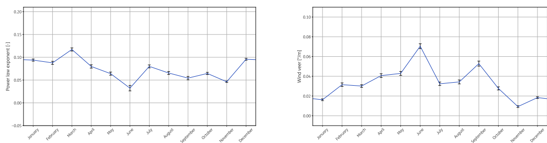
Figure A.28: Wind shear and veer as function of the month-of-year for 2023
