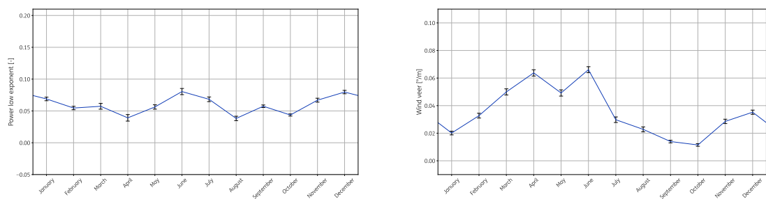
Figure A.30: Wind shear and veer as function of the month-of-year for 2025
