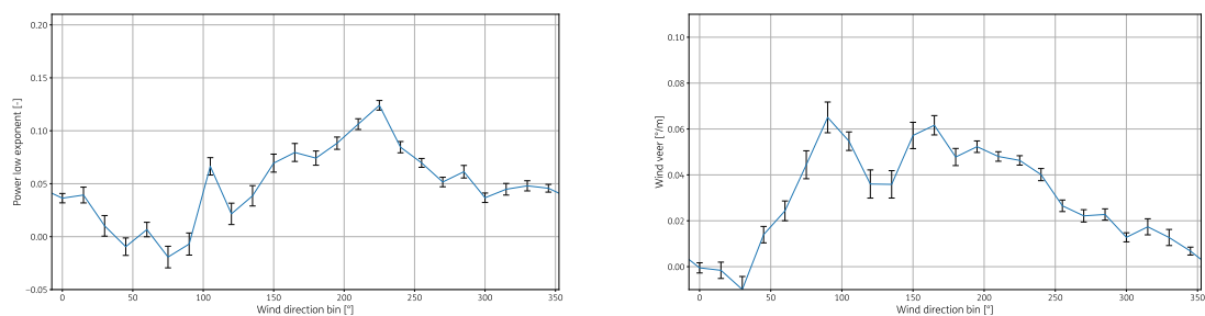
Figure A.54: Wind shear and veer as function of wind direction for 2019
