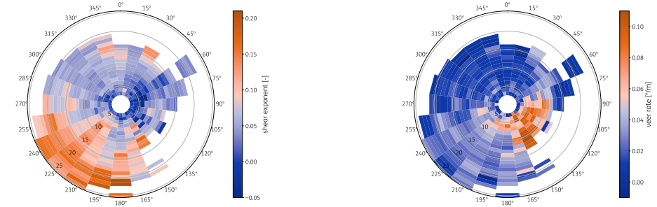
Figure A.66: Wind shear and veer as function of wind speed and direction for 2021
