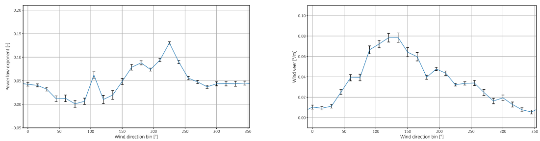
Figure A.60: Wind shear and veer as function of wind direction for 2025
