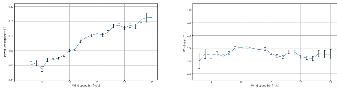
Figure A.44: Wind shear and veer as function of wind speed for 2019
