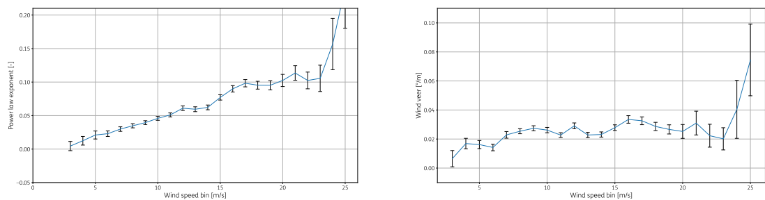
Figure A.43: Wind shear and veer as function of wind speed for 2018
