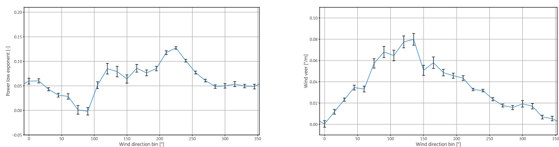
Figure A.58: Wind shear and veer as function of wind direction for 2023
