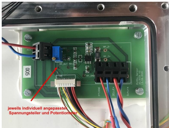
Figure 132: Picture of signal amplification board
