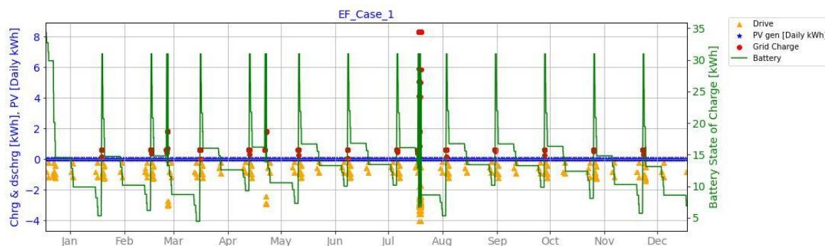
Figure 121: Energy flow for LP10 passenger car without PV using charging strategy A
