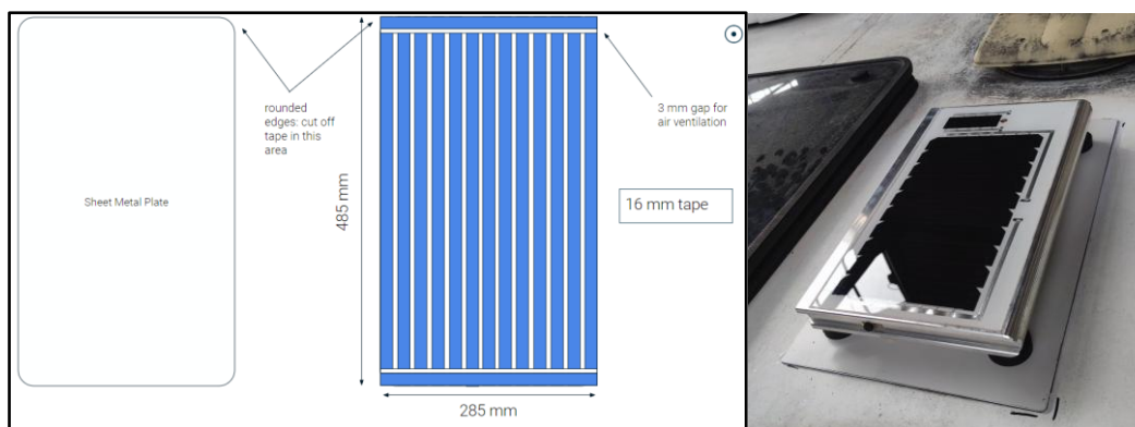
Figure 99: Non-ferromagnetic roof installation method for sensors
