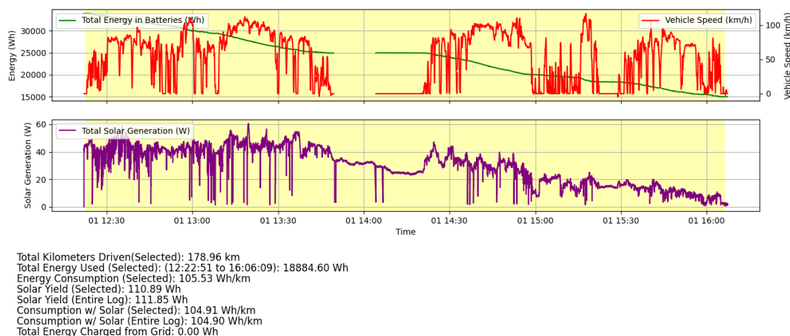
Figure 79: Energy profile of 180 km drive with 45-minute break, fully clouded day, Driver + 1 passenger (07 November 2024)
