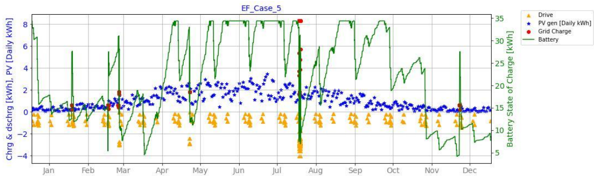
Figure 125: Energy flow for LP10 passenger car with PV on top and sides using charging strategy .
