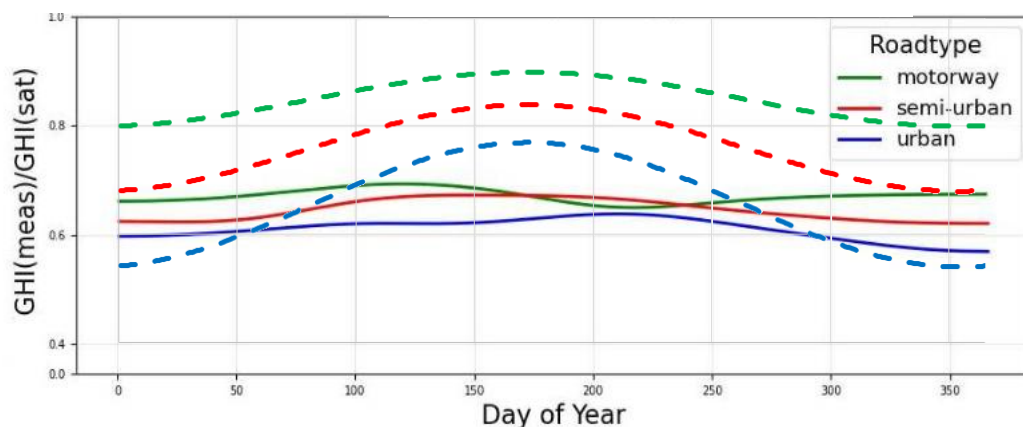
Figure 58: Total measured seasonal irradiance factor for the road types. Solid lines measurements, dashed lines model
