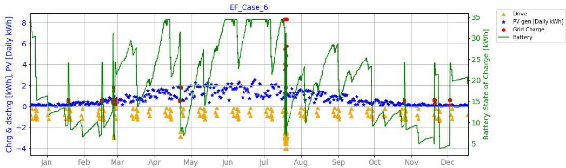
Figure 126: Energy flow for LP10 passenger car with PV on top using charging strategy C
