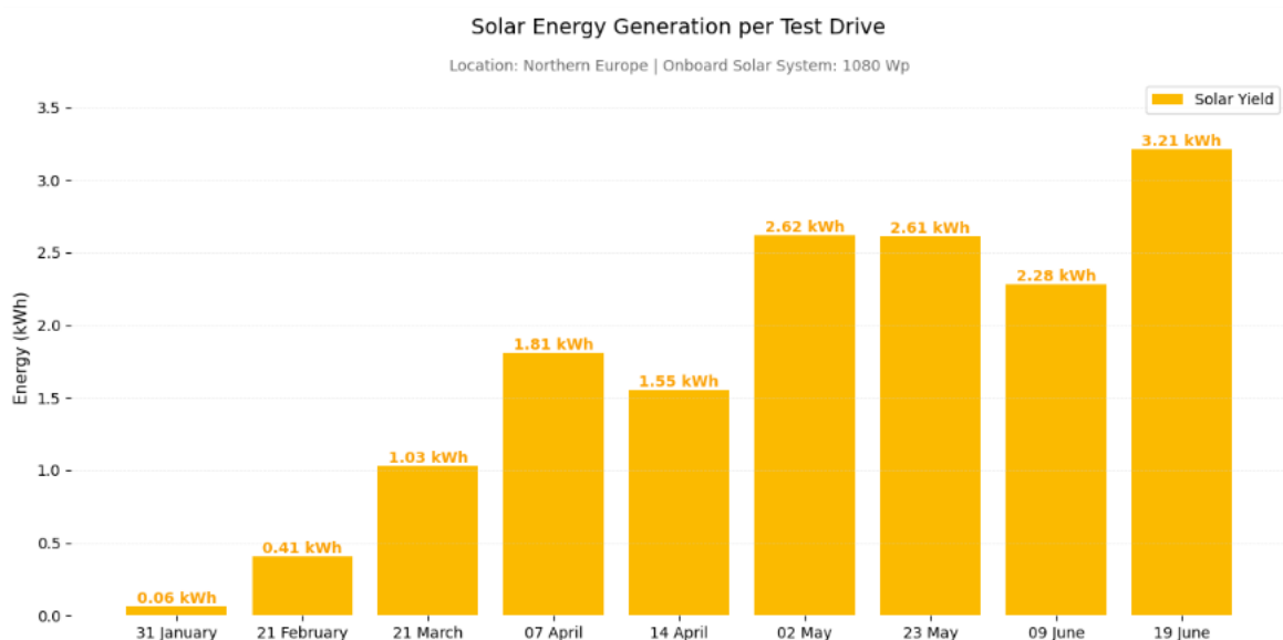
Figure 103: Solar Yield during test drives
