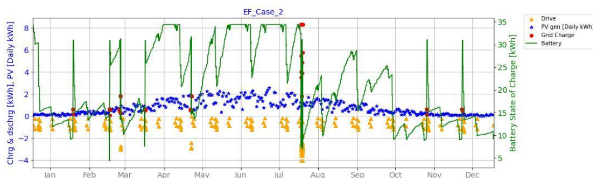
Figure 122: Energy flow for LP10 passenger car with PV on top using charging strategy A
