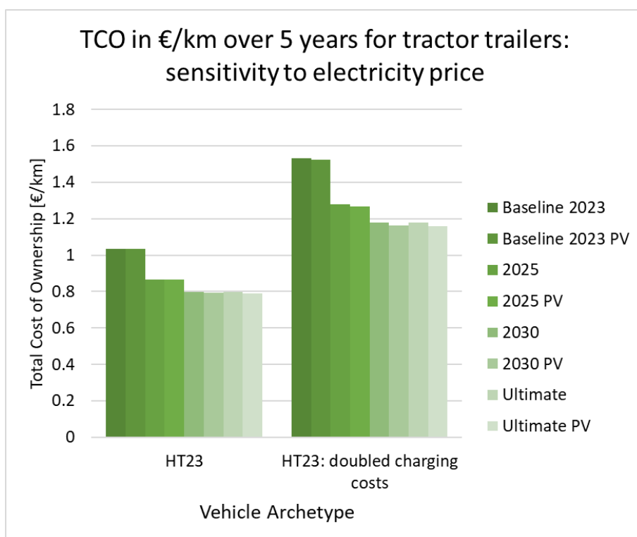
Figure 131: Total cost of ownership in euros per kilometre for long-haul tractor trailer for default and doubled charging costs, for an ownership of 5 years
