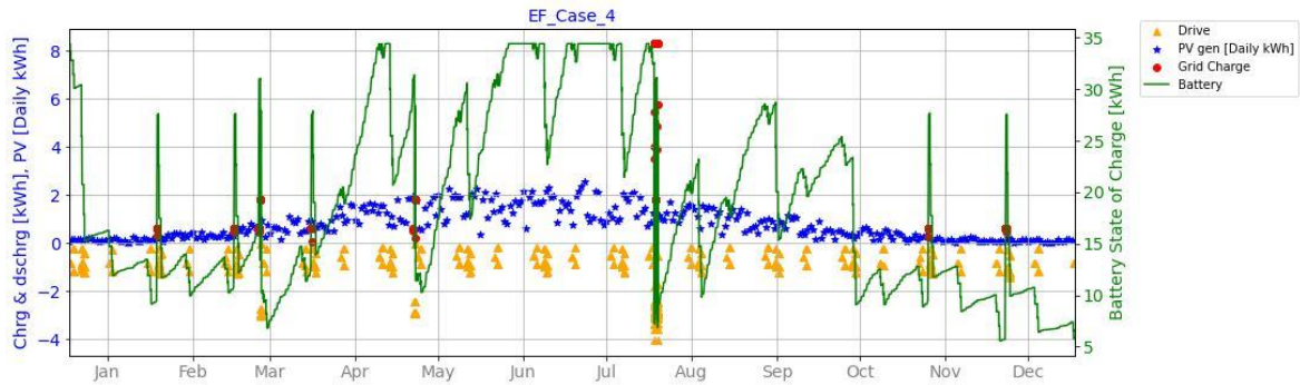
Figure 124: Energy flow for LP10 passenger car with PV on top using charging strategy .
