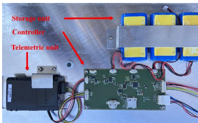
Figure 35: Picture of sensor unit electronics with battery packs
