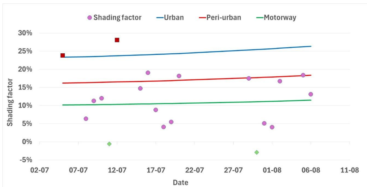
Figure 54: Truck shading loss comparison. Red squares indicate the outliers resulting from the tilt of the sensor and the green diamonds indicate the 2 outliers due to the low irradiance conditions in combination with reflection of the diffused light.
