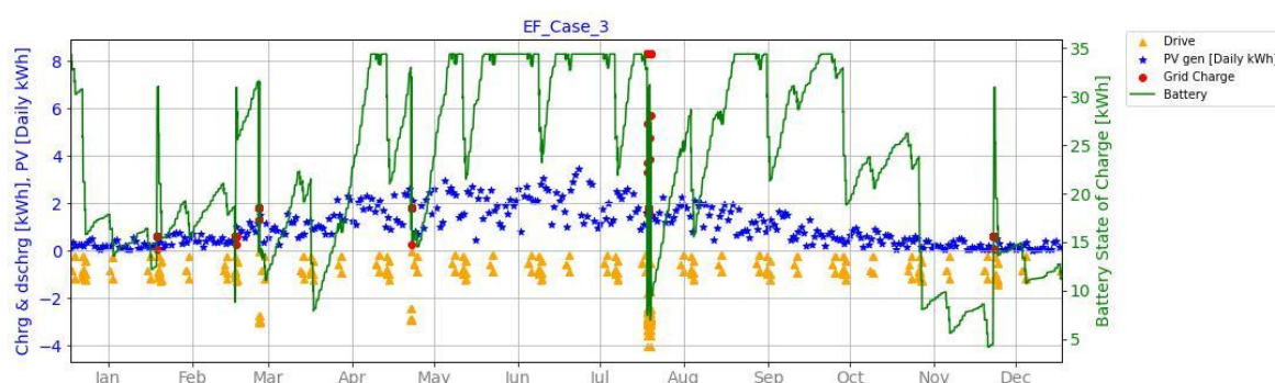
Figure 123: Energy flow for LP10 passenger car with PV on top and sides using charging strategy A
