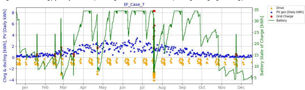
Figure 127: Energy flow for LP10 passenger car with PV on top and sides using charging strategy C
