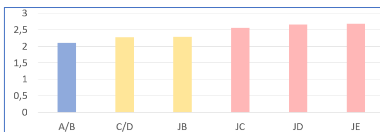
Figure 114: Frontal area (m 2 ) of the different categories compared
