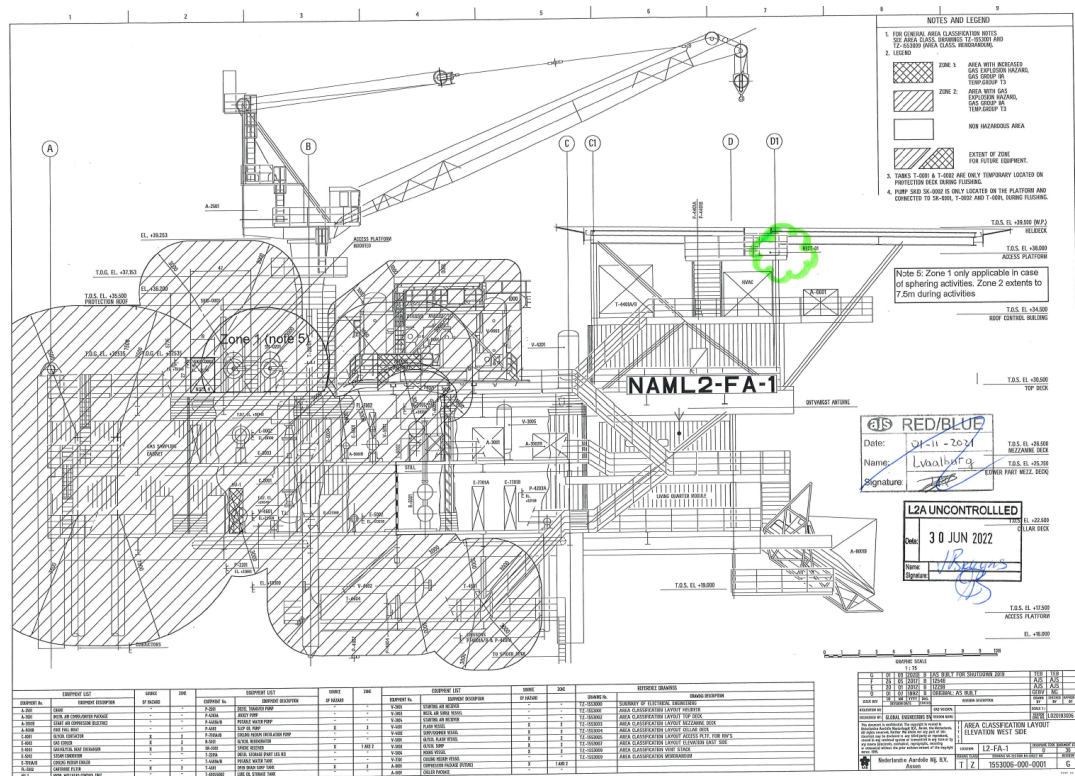
Figure 2.3: Side view of the L2-FA-1 platform with the position of the lidar marked in green.
