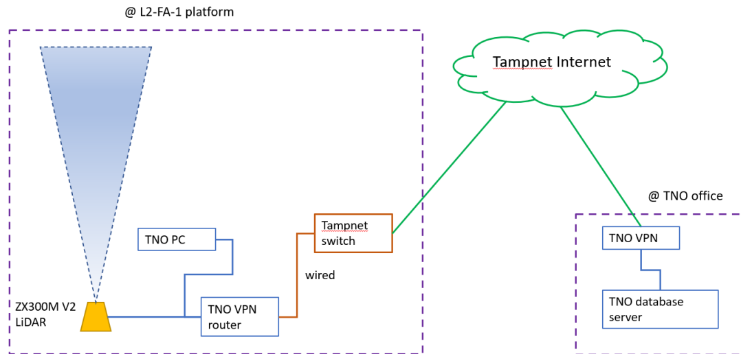
Figure 4.2: L2-FA-1 lidar campaign network layout.
