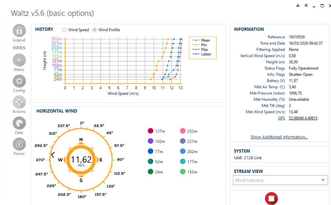
Figure 6.1: Screenshot of ZX Lidars software Waltz.
