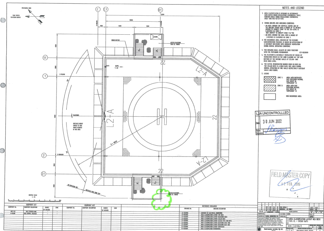
Figure 2.2: Top view the L2-FA-1 helideck with the position of the lidar marked in green.
