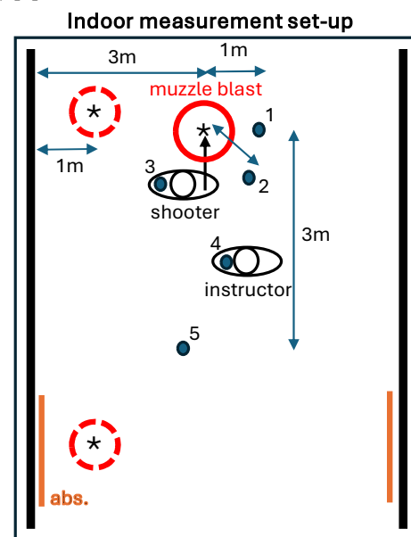
Figure 1. Measurement set-up using 5 microphones (blue markers) near the muzzle blast using 3 different firing positions (red circles).
