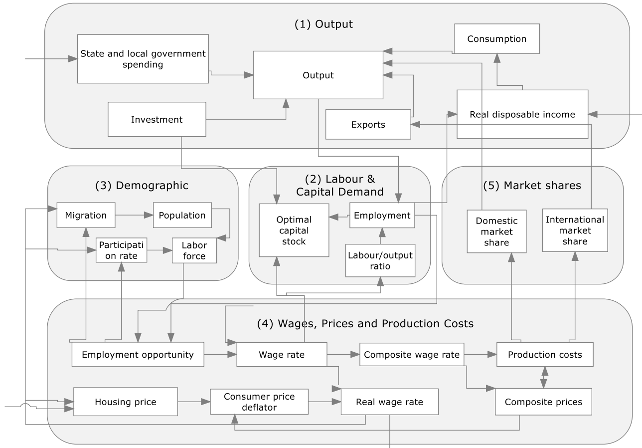
Fig. 6. Links between different part of the model
