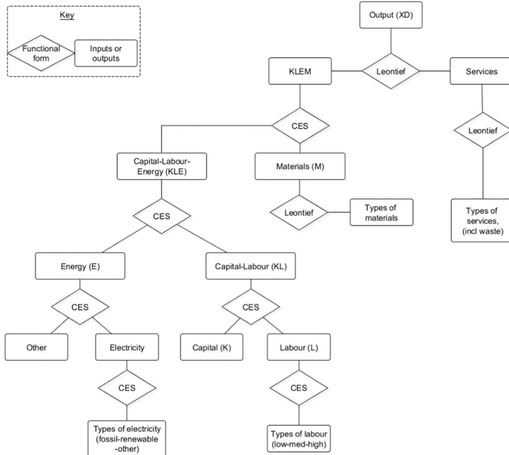
Fig. 7. Structure of KLEM production functions in the model
