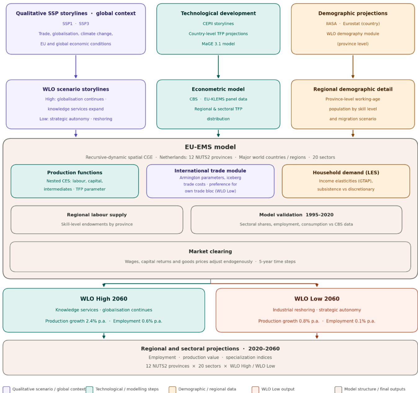
Fig. 1. Data flow and modeling framework for the quantification of WLO scenarios at the regional and sectoral level.
