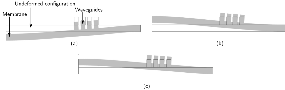
Fig. 8. (a) Displacement profiles of the MZI-based IPUT for different frequencies and internal stresses: (a) 1 \text{ Hz} and 0 \text{ Pa} (static deflection) (b) 1.03 \text{ MHz} and 0 \text{ Pa} at the first (fundamental) resonant mode, which is similar to the static deflection (with a \pi phase shift due to the resonance), and (c) 1 \text{ Hz} and -250 \text{ MPa} : the static case with internal stress that is again similar to the previous two cases.
