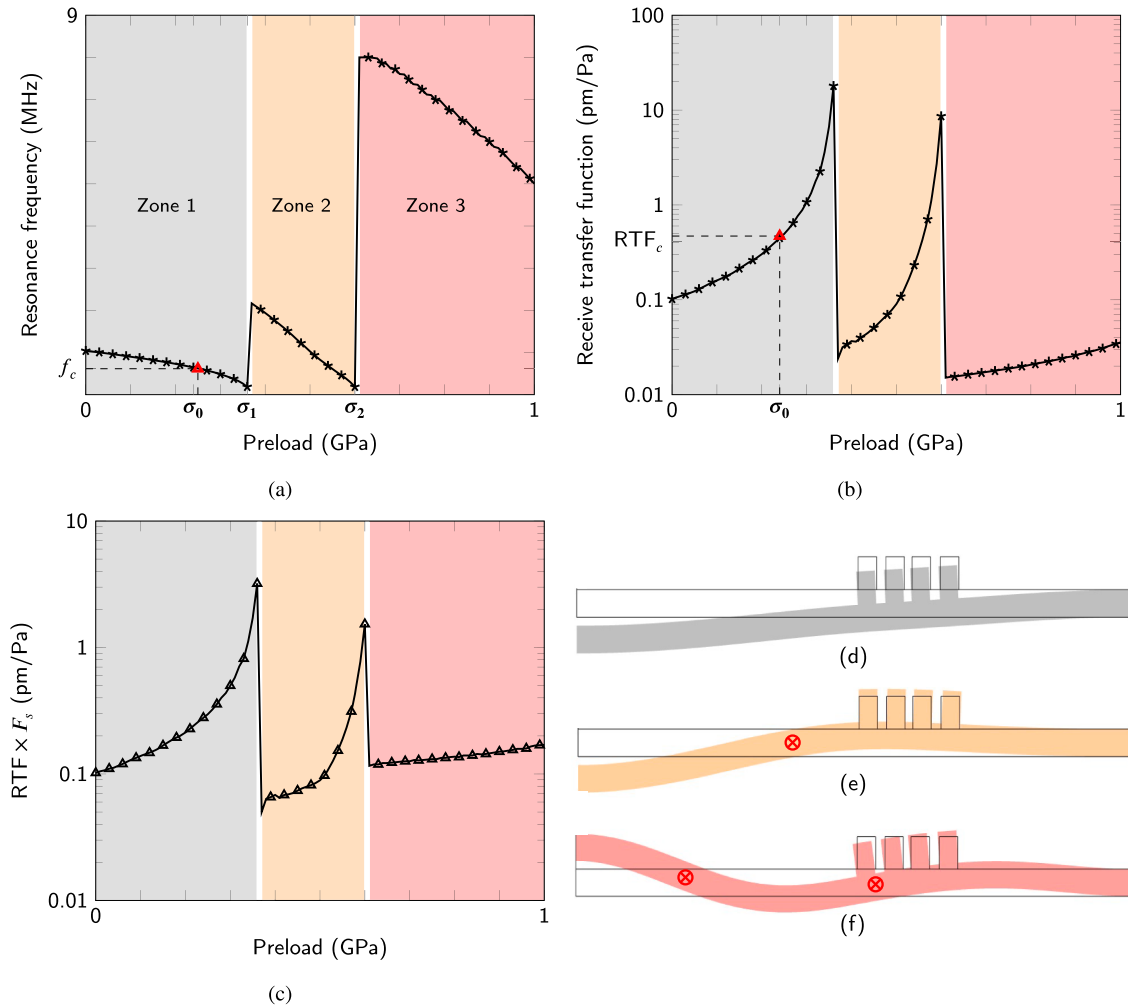
Fig. 9. Parametric response of the MZI-based IPUT: (a) Resonance frequency variation with internal stress from 0 to -1 GPa where the first two buckling loads \sigma_1 = -360 MPa and \sigma_2 = -600 MPa are marked. The plot is separated into three zones based on the mode shapes of the IPUT. There are sharp discontinuities between each zone, evidence of a mode change. The internal stress experienced by the IPUT ( \sigma_i = -250 MPa) and the corresponding resonance frequency ( f_c = 0.61 MHz) obtained experimentally are also marked here. (b) The variation of RTF with the internal stress, where sudden increases in RTF values close to critical loads are visible. The internal stress \sigma_i and corresponding RTF ( RTF_c = 0.47 pm/Pa) also attained experimentally are marked in the plot. (c) The variation of the product of RTF with the frequency ratio ( F_s ) is plotted for the same range of internal stress. (d), (e) and (f), respectively are displacement profiles of the MZI-based IPUT for different frequencies and internal stresses: (d) 0.62 MHz and -250 MPa, i.e., the actual operating condition of the IPUT, which is similar to the resonant mode without internal stress (in Zone 1). (e) 1.93 MHz and -400 MPa, which is the IPUT's behavior after crossing the first critical load (in Zone 2), where its deformation pattern is similar to a second vibration mode with the presence of a node (red cross). (f) 6.86 MHz and -800 MPa operating in Zone 3 after crossing the second critical load, where the IPUT's displacement profile is equivalent to the third vibration mode with two nodes. (For interpretation of the references to colour in this figure legend, the reader is referred to the web version of this article.)
