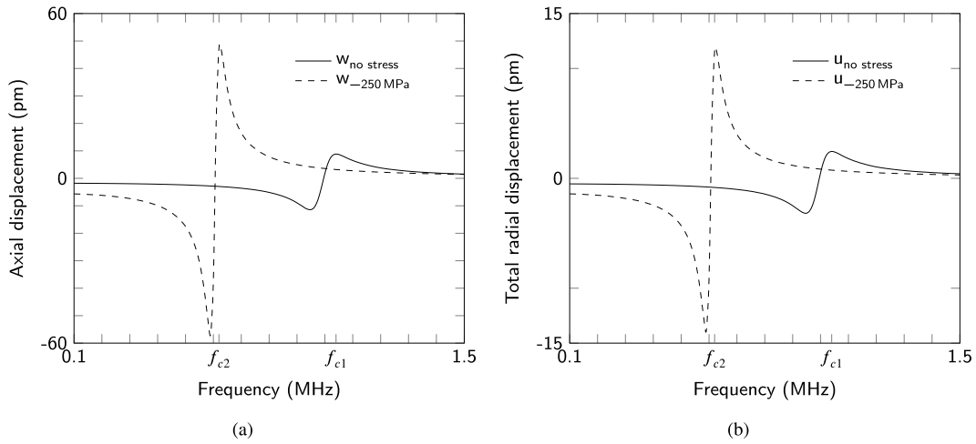
Fig. 7. Comparison of the MZI-based IPUT with and without internal stress ( -250 \text{ MPa} ): (a) axial displacement extracted at the center of the plate as a function of frequency where the resonance frequencies f_{c1} = 1.03 \text{ MHz} (without internal stress) and f_{c2} = 0.62 \text{ MHz} (with -250 \text{ MPa} internal stress), are marked. (b) total radial displacement of all four loops of the MZI as a function of the applied frequency, showing an enhanced radial displacement of the waveguide for -250 \text{ MPa} internal stress.
