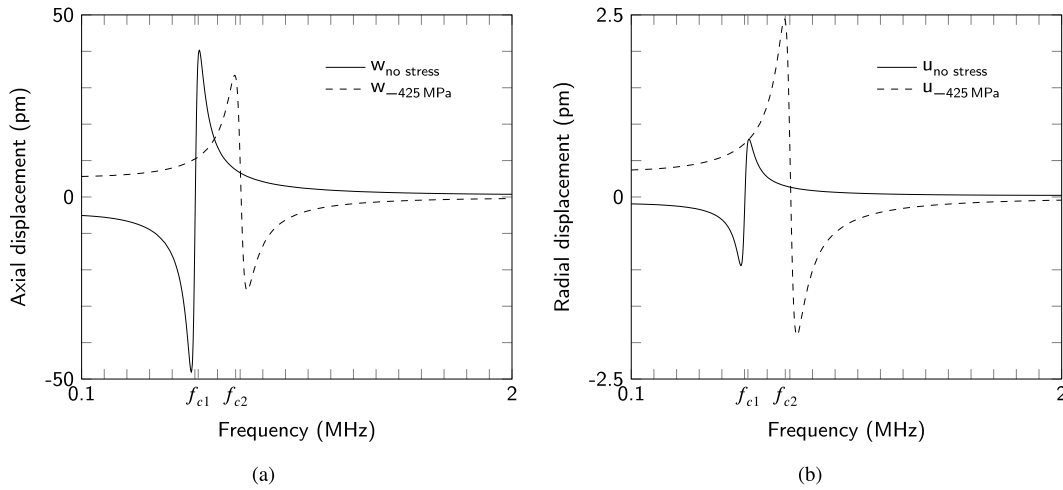
Fig. 11. Comparison of the RR-based IPUT with and without an internal stress ( -425 \text{ MPa} ): (a) axial displacement as a function of frequency where the resonance frequencies f_{c1} = 0.62 \text{ MHz} —without internal stress and f_{c2} = 0.78 \text{ MHz} —with -425 \text{ MPa} internal stress are marked. (b) radial displacement of the ring (of RR) as a function of the applied frequency, showing an enhanced radial displacement of the waveguide with the presence of -425 \text{ MPa} internal stress. Both axial and radial displacement show that the IPUT with internal stress experiences a \pi phase shift associated with vibration about a different equilibrium configuration.
