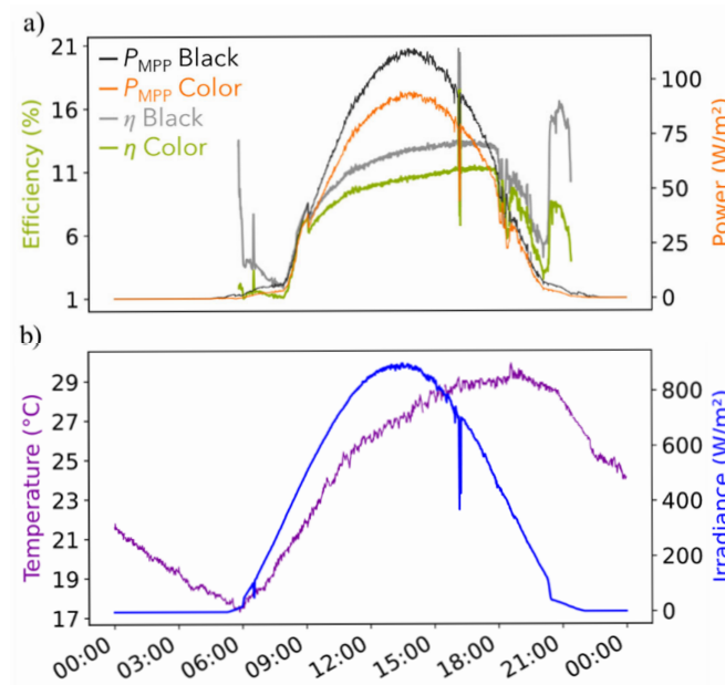
Figure 10. (a) Single-day measurements on the 25 June 2024 with a tilt angle of 30^{\circ} showing the P_{MPP}/m^2 (black) and efficiency (gray) of the non-colored solar panels and P_{MPP}/m^2 (orange) and efficiency (green) for the colored solar panels; (b) the irradiance (blue) and outdoor temperature (purple) over time. All data were filtered to irradiance \geq 15 W/m^2 to avoid outliers due to on/off switching of the inverter.
