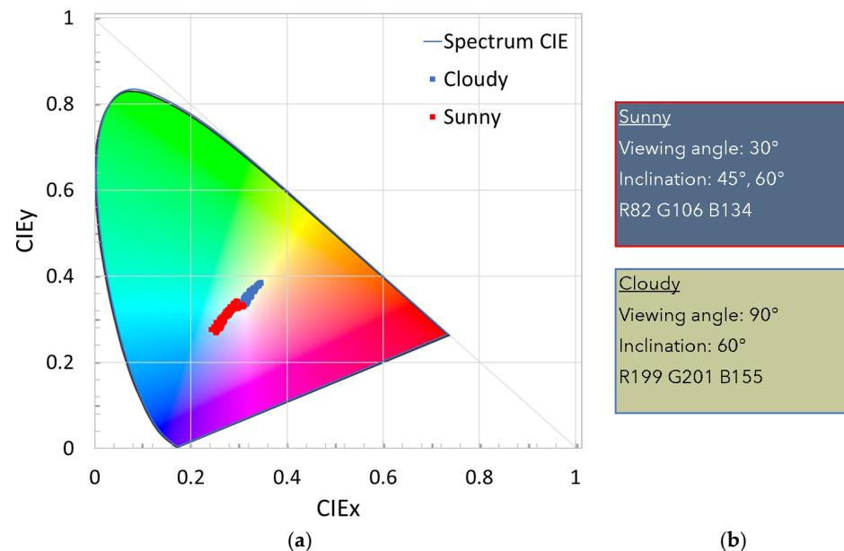
Figure 6. (a) CIE 1931 spectrum along with all measurement points on sunny days (red) and cloudy days (blue) with viewing angles ranging from 30° to 150° and tilt angles of the test setup of 60° and 45°; (b) a visualization of the extreme colors that have been measured.
