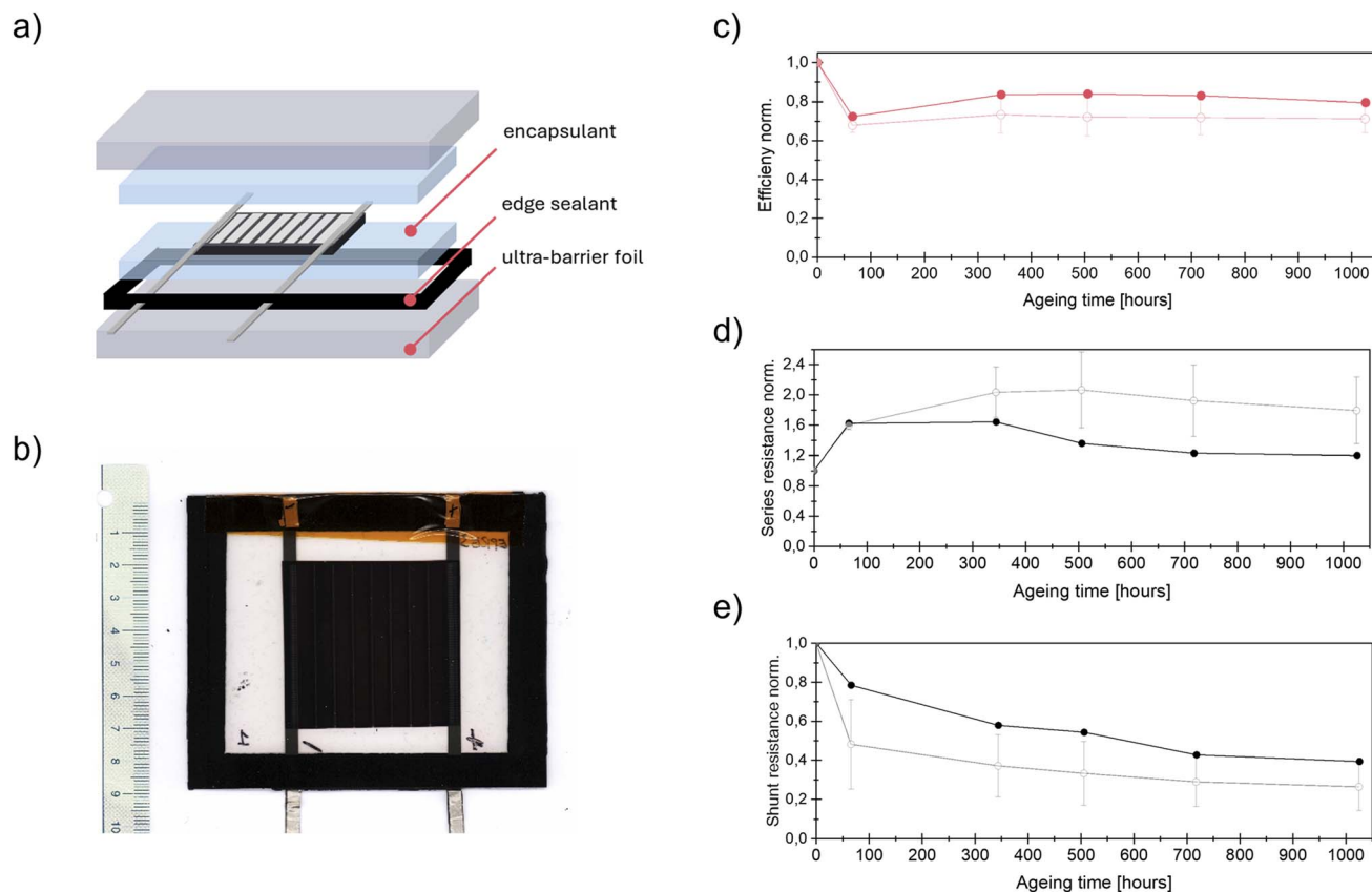
Fig. 3 (a) Schematic of the encapsulation layer stack, (b) picture of the encapsulated PSM, (c) normalized efficiency evolution upon the DH stability test, (d) normalized series resistance evolution upon the DH stability test, and (e) normalized shunt resistance evolution upon the DH stability test. On the graphs, the solid symbol represents the data for the most stable module, and open symbols represent the average and associated standard deviations across all five tested modules.
