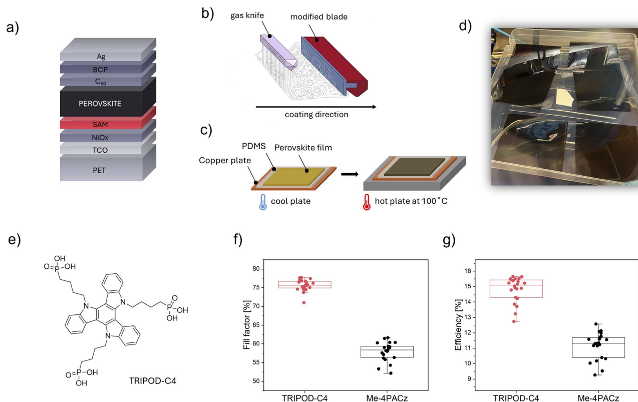
Fig. 1 (a) Scheme of the inverted WBG PSC layer stack, (b) scheme of the modified blade with a shielding element, (c) scheme of the gradual annealing step using a PDMS-covered copper plate, (d) picture of 90 \text{ cm}^2 -sized blade-coated samples up to perovskite from which individual solar cells were extracted, (e) structure of TRIPOD-C4, and (f and g) statistics of the fill factor and efficiency for blade-coated WBG PSCs employing TRIPOD-C4 and Me-4PACz as a SAM.
