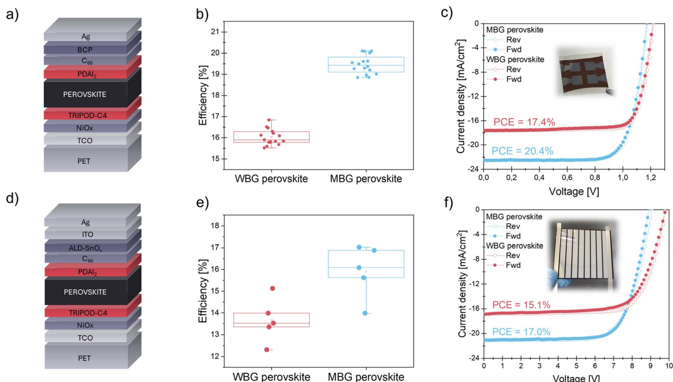
Fig. 2 (a) Scheme of the optimized inverted PSC stack, (b) statistics of efficiency for flexible, blade-coated solar cells employing WBG and MBG perovskite absorbers, (c) J - V curves (forward and reverse scan directions) of top-performing solar cells with the WBG and MBG absorbers, (d) scheme of the optimized inverted PSM stack, (e) statistics of efficiency for flexible, blade-coated solar modules employing WBG and MBG perovskite absorbers, and (f) J - V curves (forward and reverse scan directions) of the top-performing solar module with the WBG and MBG perovskite absorbers.
