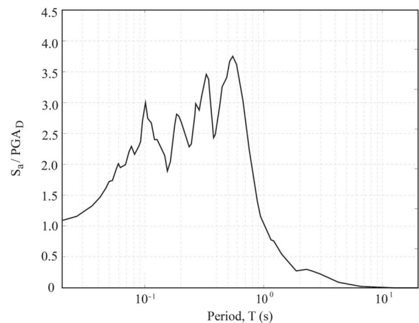
FIGURE 7 Response spectrum function of the deterministic solution ( \text{RSF}_D ).
