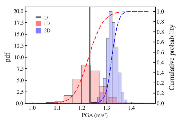
FIGURE 11 Pdf and cumulative probability of PGA values reached during the earthquake for 1D and 2D analyses, compared with the deterministic solution.
