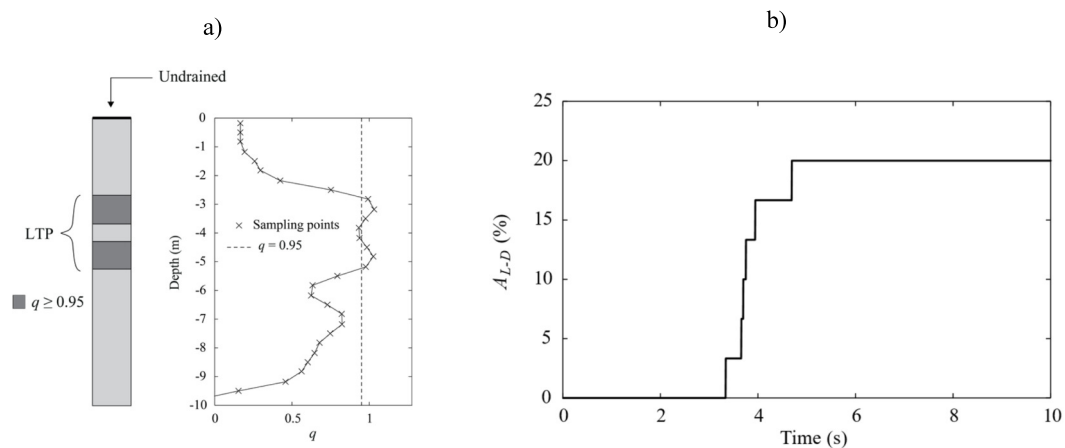
FIGURE 5 (a) Liquefied zones after the earthquake next to the variation of q with depth, and (b) deterministic liquefied area A_{L-D} as a function of time.
