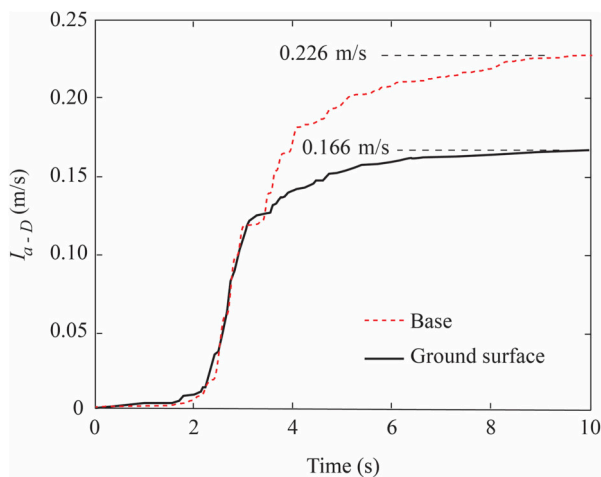
FIGURE 6 Arias intensity of deterministic solution I_{a-D} .
