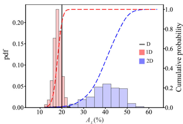
FIGURE 10 Pdf and cumulative probability of A_L reached at the end of the earthquake for 1D and 2D analyses, compared with the deterministic solution.
