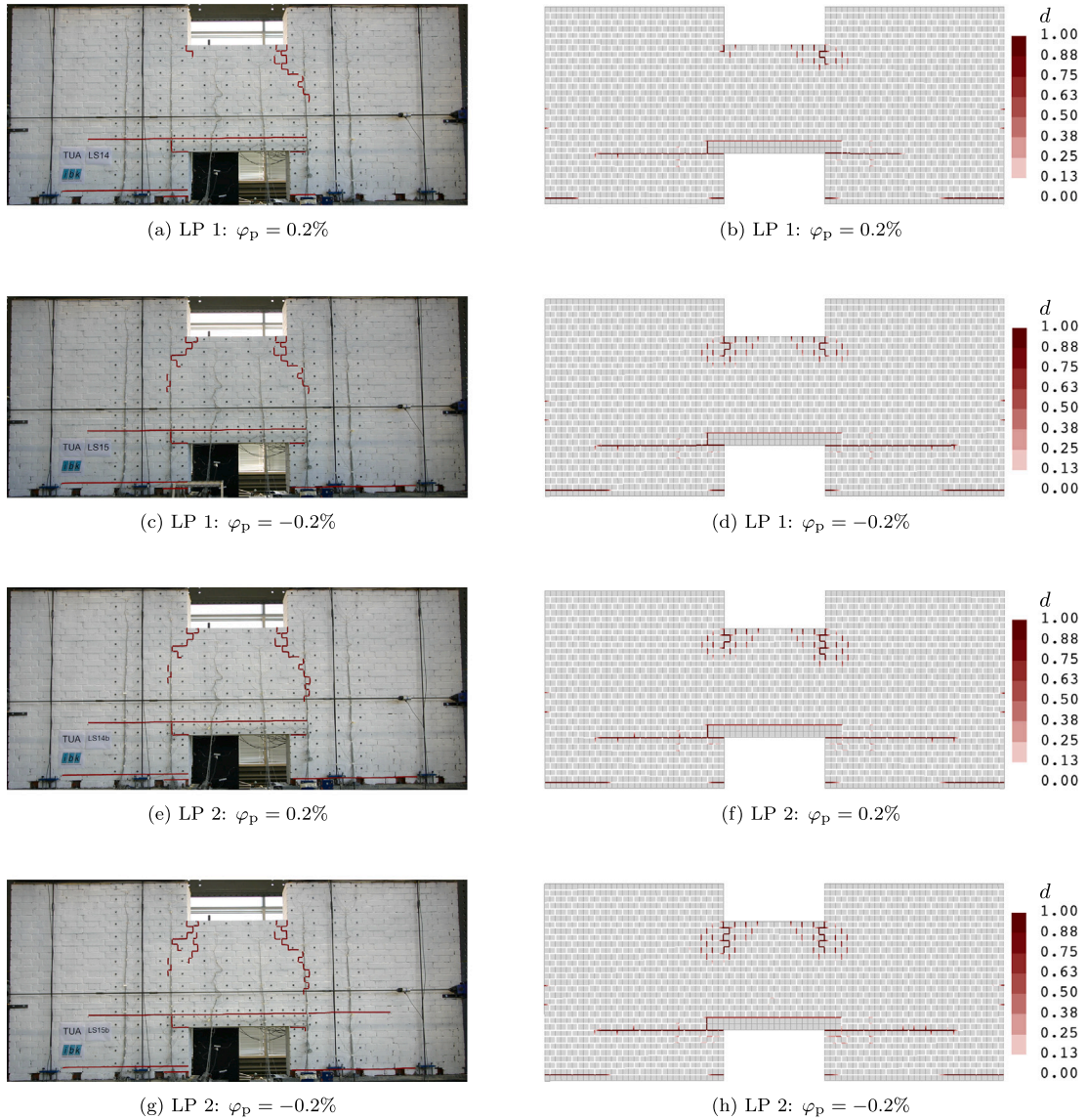
Fig. 21. Evolution of the damage for LP 1 and 2: experimental (left) versus numerical (right). The original pictures are provided by K. Beyer and modified by the authors to highlight the crack pattern.
