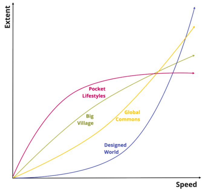
Fig. 8. Conceptual and purely-illustrative visualisation of speed vs extent of the SLIM scenario narratives.
