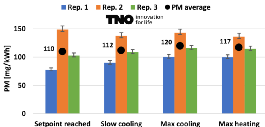
Figure 4-8: PM emissions per kWh of the TRU under four conditions (temperature setpoint reached, slow cooling, fast cooling and fast heating) with increasing engine load from left (around 3kW) to right (around 7kW). Each coloured bar represents a measurement repetition, the whiskers on each bar represent measurement uncertainty. The black dots are the average values for each condition.
