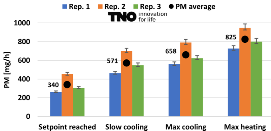
Figure 4-7: PM emissions per hour of the TRU under four conditions (temperature setpoint reached, slow cooling, fast cooling and fast heating) with increasing engine load from left (around 3kW) to right (around 7kW). Each coloured bar represents a measurement repetition, the whiskers on each bar represent measurement uncertainty. The black dots are the average values for each condition.
