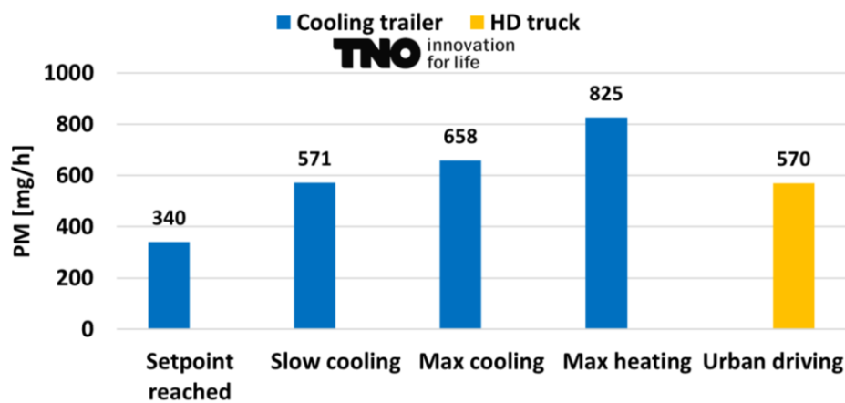
Figure 4-9: Average PM emissions per hour of the TRU under four conditions (temperature setpoint reached, slow cooling, fast cooling and fast heating) with increasing engine load from left (around 3kW) to right (around 7kW) displayed with the blue bars. The yellow bar represents the PM emissions per hour of a Euro 6 HD truck driving under urban conditions, based on the national emission factors.
