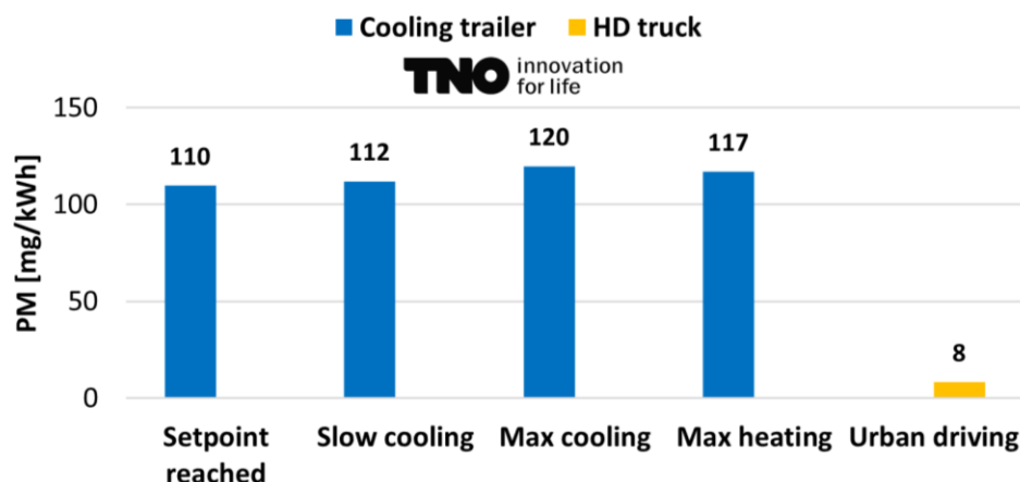
Figure 4-10: Average PM emissions per kWh of the TRU under four conditions (temperature setpoint reached, slow cooling, fast cooling and fast heating) with increasing engine load from left (around 3kW) to right (around 7kW) displayed with the blue bars. The yellow bar represents the PM emissions per kWh of a Euro 6 HD truck driving under urban conditions, based on the national emission factors.
