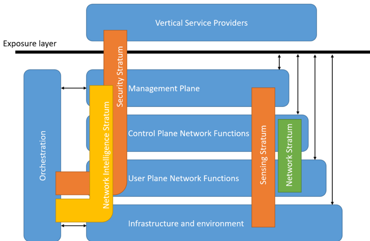
Figure 17: Functional view of the proposed 6G reference architecture [5G PPP]
