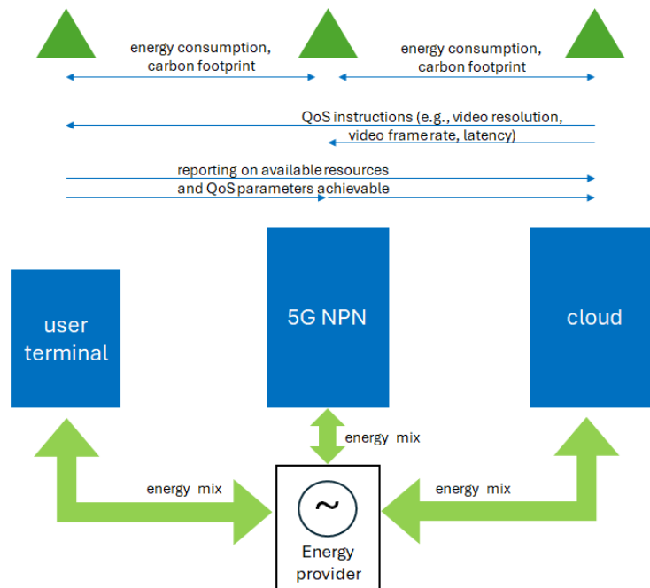
Figure 12: Functional Architecture instantiated for UC9
