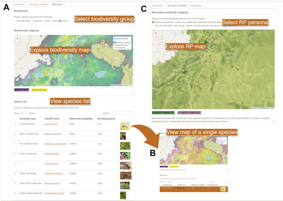
Figure 2. doi Screenshots from pDT user interface minimal viable product. The page has three tabs, the first (not illustrated) is an information tab with an overview of the pDT. The recreation potential tab (C) offers maps for different RP personas. The biodiversity tab has maps of species distributions available as groups of species or individual species (A) and species are listed, based on their probability of occurrence and the DECIDE recording priority (B). Further developments of the pDT will provide means to access the data and better integrate between the two components on the pDT.
