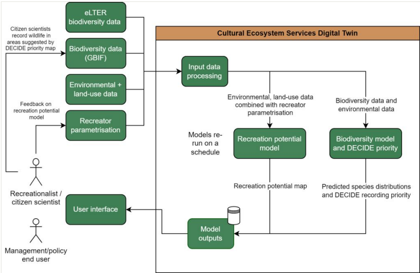
Figure 1. doi Conceptual schema of the Recreation and Biodiversity Cultural Ecosystem Services, Prototype Digital Twin.
