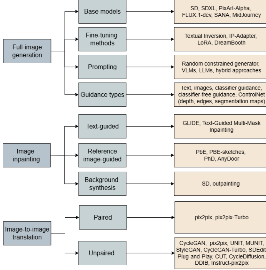
Figure 1: Overview of GenAI methods for synthesizing image data.
