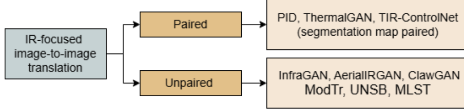
Figure 5: An overview of the models found in literature that focus specifically on RGB-IR domain translation tasks or data augmentation for enhanced performance in downstream AI-tasks on IR imagery.
