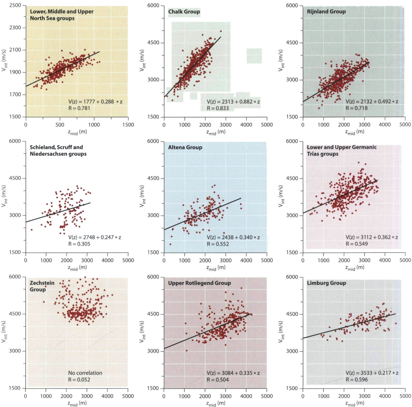
Fig. 5. Linear least squares relation between V_{int} and z_{mid} for the various lithostratigraphic layers.
