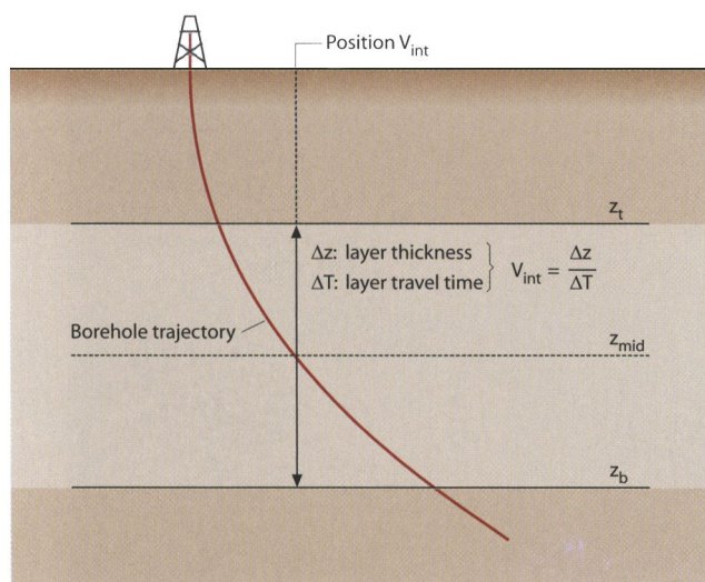
Fig. 3. V_{\text{int}} and its position in case of a layer perforated by a deviated borehole.
