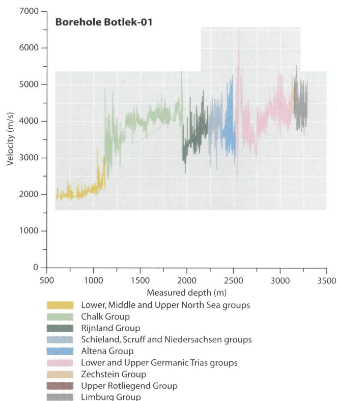
Fig. 4. Velocity representation of sonic log data in borehole Botlek-01 with lithostratigraphic interpretation (see Fig. 2 for location of this borehole).
