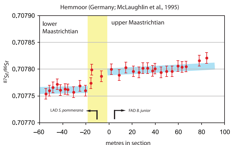
Fig. 4. Graph showing ^{87}\text{Sr}/^{86}\text{Sr} values of chalk from the Hemmoor section (northern Germany; McLaughlin et al., 1995). Although the top part of the upper Maastrichtian is not present in this section, data available suggest a distinct ^{87}\text{Sr}/^{86}\text{Sr} transition to occur between 0 m and -20 m from a lower to a higher ^{87}\text{Sr}/^{86}\text{Sr} plateau. The FAD of Belemnitella junior and the LAD of Stensioeina pommerana are indicated. See text for discussion of the biostratigraphical data; we correlate the ^{87}\text{Sr}/^{86}\text{Sr} step pattern, indicated by a yellow vertical bar, to the step in ^{87}\text{Sr}/^{86}\text{Sr} values visible in the Maastricht record (see Fig. 3).
