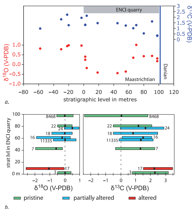
Fig. 7a. Graph showing \delta^{18}\text{O} values (in red) and \delta^{13}\text{C} values of the micromilled portions of belemnites from the Maastricht sequence. \delta^{13}\text{C} data define a stratigraphical trend towards lower values through the complete record; \delta^{18}\text{O} values show a more complex pattern with a rapid drop of \sim 1.5 permille around 0 metre in the composite section, followed by an increase to higher values at \sim 60 metre in the section; b. Graphic representation of the total range of \delta^{18}\text{O} and \delta^{13}\text{C} values within sclerochronologically sampled belemnites at different stratigraphical levels of the ENCI-HeidelbergCement Group quarry. Colour coding of the range bars indicates the preservational state of the belemnite as reconstructed from the trace element composition of all belemnite subsamples. Average stable isotope values are indicated by a black vertical marker in the range bars. The bulk isotope values in Fig. 7a compare relatively well to the average values of the sclerochronologically sampled belemnites in Fig. 7b. This suggests that stable isotope data of selectively sampled portions of the belemnites depicted in Fig. 7a are stratigraphically representative.
