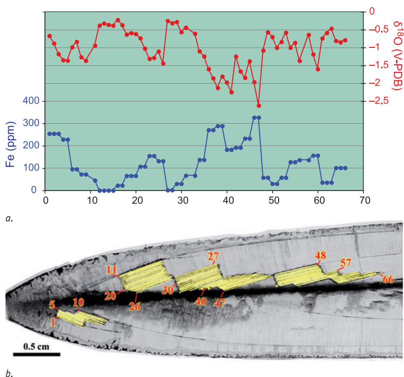
Fig. 2a. Graph illustrating a sclerochronologic record of oxygen isotope and Fe concentration data of belemnite sample HVENCI-17 (see Fig. 1b). Conspicuous antiphasic behaviour of Fe concentration and \delta^{18}\text{O} values of belemnite calcite indicates diagenetic alteration to have controlled \delta^{18}\text{O} variation; b. photomicrograph of a thin section of belemnite sample HVENCI-17, showing the microsample traces made to produce the record in Fig. 2a. A closer inspection of Fig. 2a and b reveals that high Fe concentrations (and low \delta^{18}\text{O} values) consistently occur in samples close to the apical line (dark horizontal line along the central axis of the belemnite in Fig. 2b) where diagenetic fluids were able to penetrate the rostrum.
