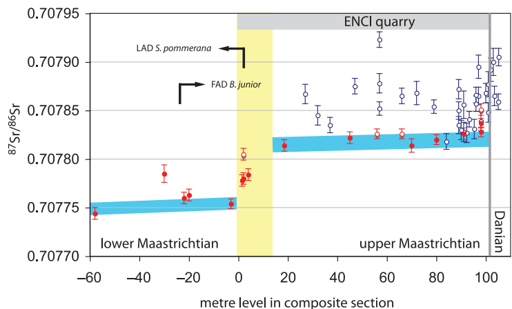
Fig. 3. Graph showing all Sr isotope data of belemnites analysed for this study (in red) compared to previously published Sr isotope analyses of other fossils from the ENCI-HeidelbergCement Group and Ankerpoort-Curfs quarries, Geulhem (in blue; see Vonhof & Smit, 1996). Data points from the Vonhof & Smit (1996) study show a significantly higher scatter and raised ^{87}\text{Sr}/^{86}\text{Sr} values than those of the belemnites, which we interpret as the result of diagenetic alteration in the former data set. Belemnite ^{87}\text{Sr}/^{86}\text{Sr} data define two periods of relatively stable ^{87}\text{Sr}/^{86}\text{Sr} values; these plateaus are connected by a relatively rapid transition, indicated by a yellow vertical bar. In the belemnite data, open circles represent the four samples that were prepared from discrete belemnite fragments, while closed circles represent micromilled belemnite rostra.
