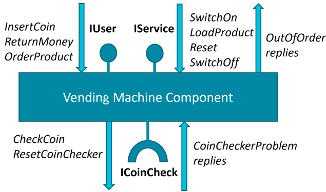
Figure 1 Vending machine example
