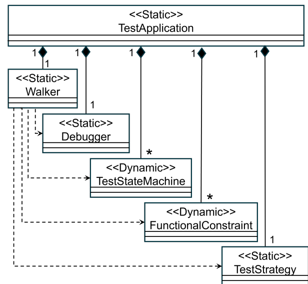
Figure 4 Class Diagram of the Test Application
