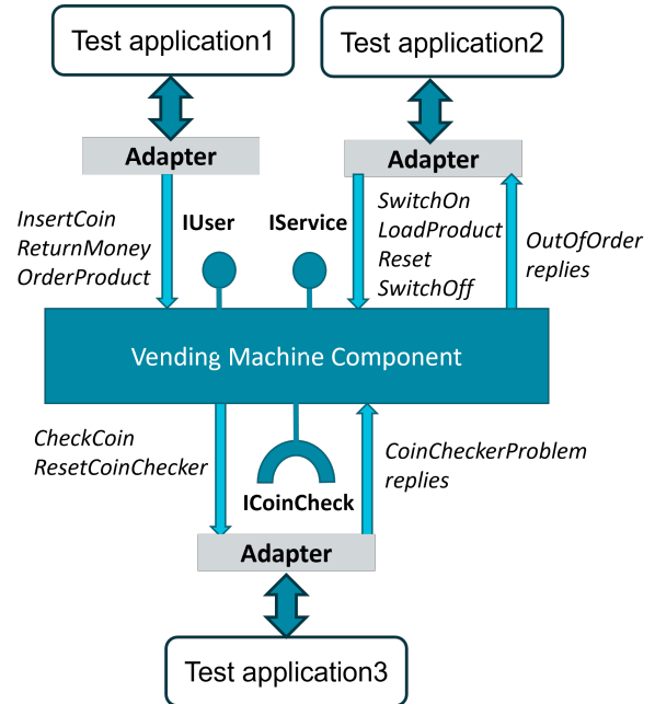
Figure 6 Multiple Test Applications
