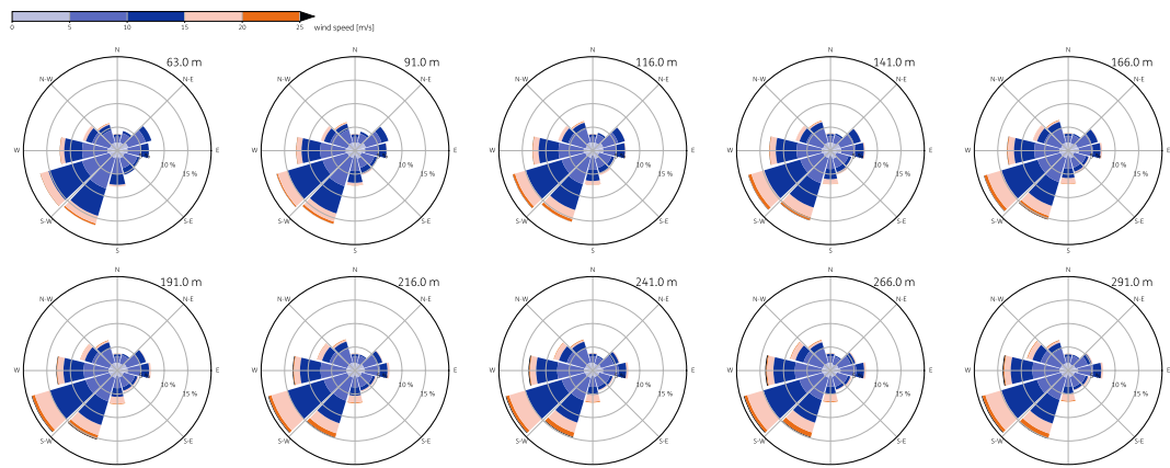
Figure A.2: Wind roses for 2017
