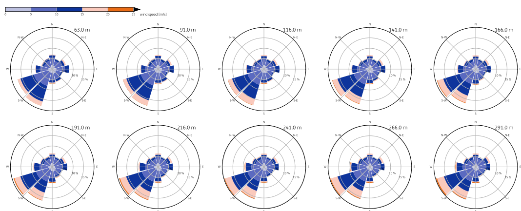
Figure A.1: Wind roses for 2016
