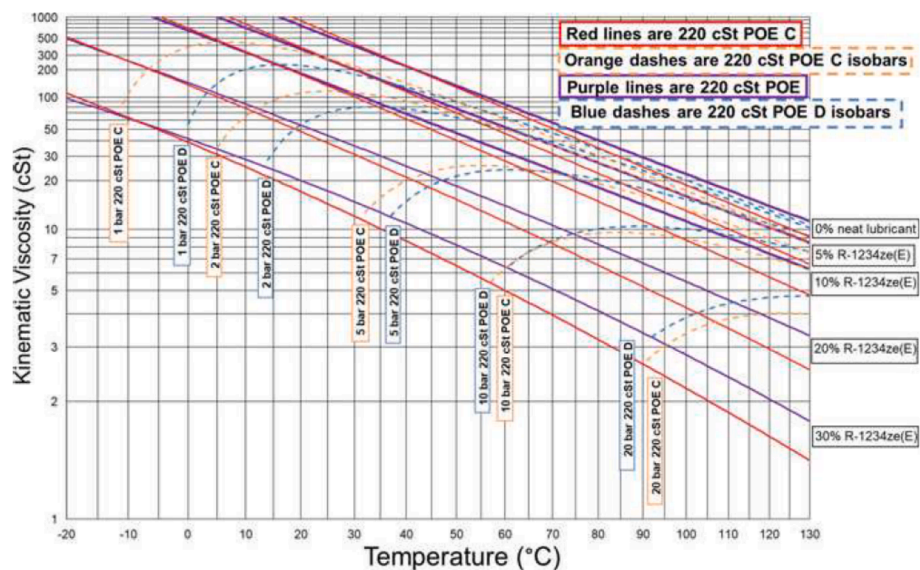
Fig. 17. Daniel plots for the two POE oils mixtures with R1234ze(E) [129].
