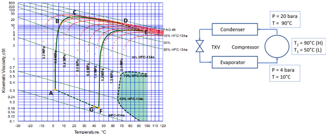
Fig. 13. Daniel plot for HFC-134a/PAG 46 mixture (left) and compression cycle (right) [79].
