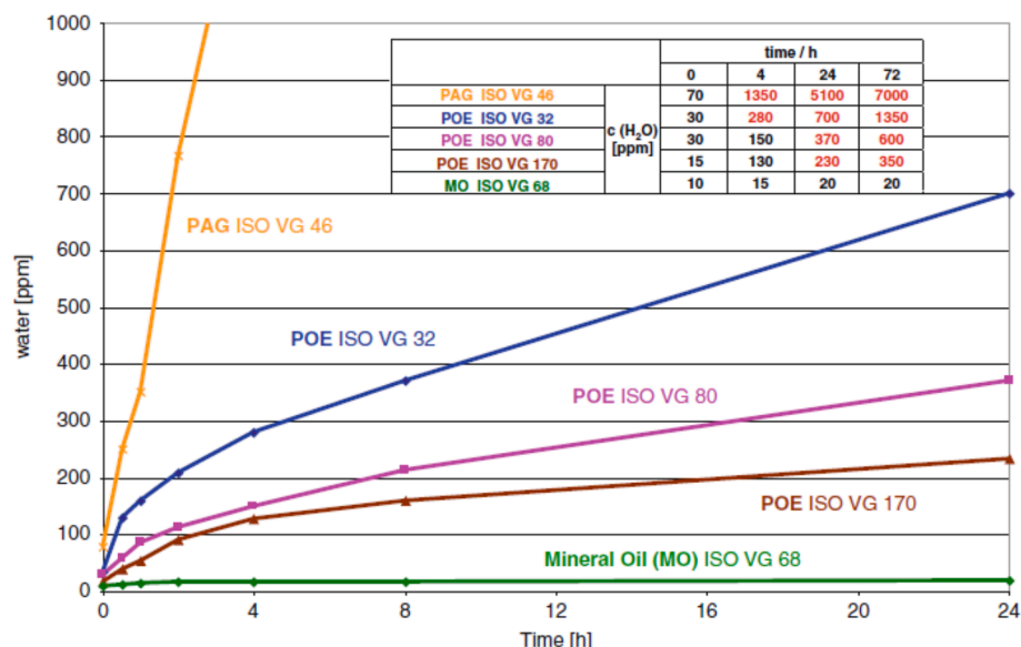
Fig. 10. Water absorption of different lubricant oils [20,78].
