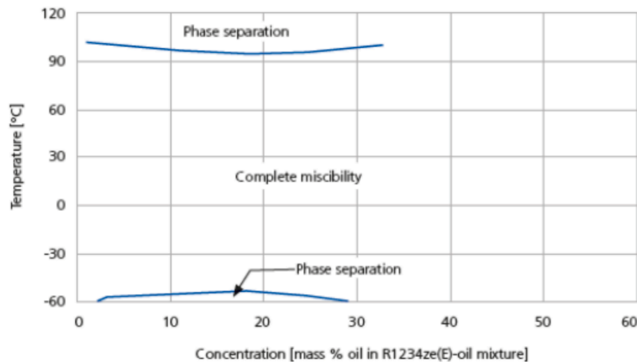
Fig. 19. Miscibility of RENISO TRITON SE 170 (POE) and R1234ze(E) [78].
