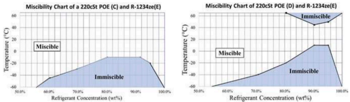
Fig. 16. Miscibility graphs for two different POE oils with R 454 [129].
