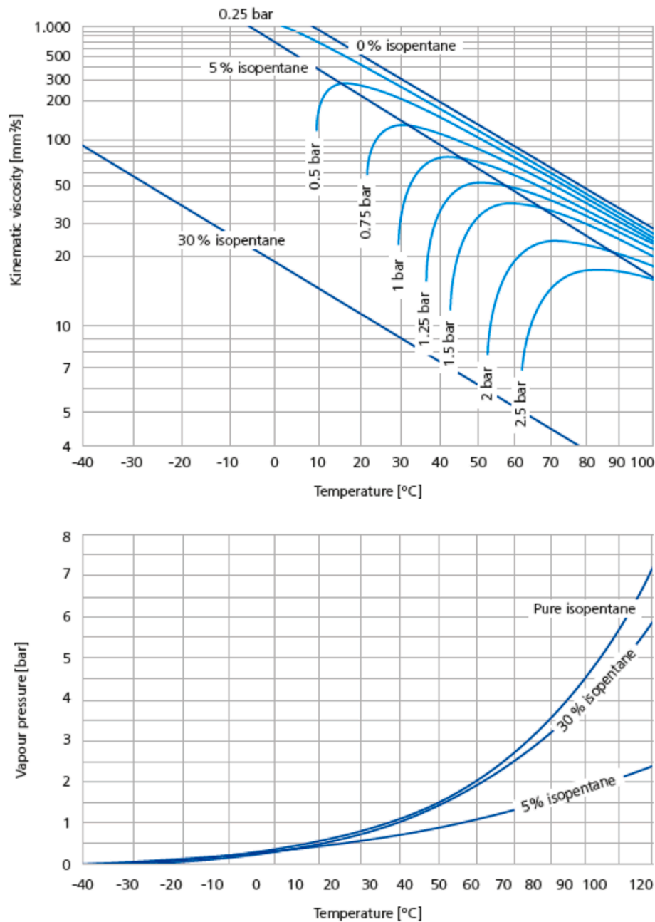
Fig. 24. Daniel plot for RENISO LPG 185 (PAG)- R601a (i-pentane) mixture [78].
