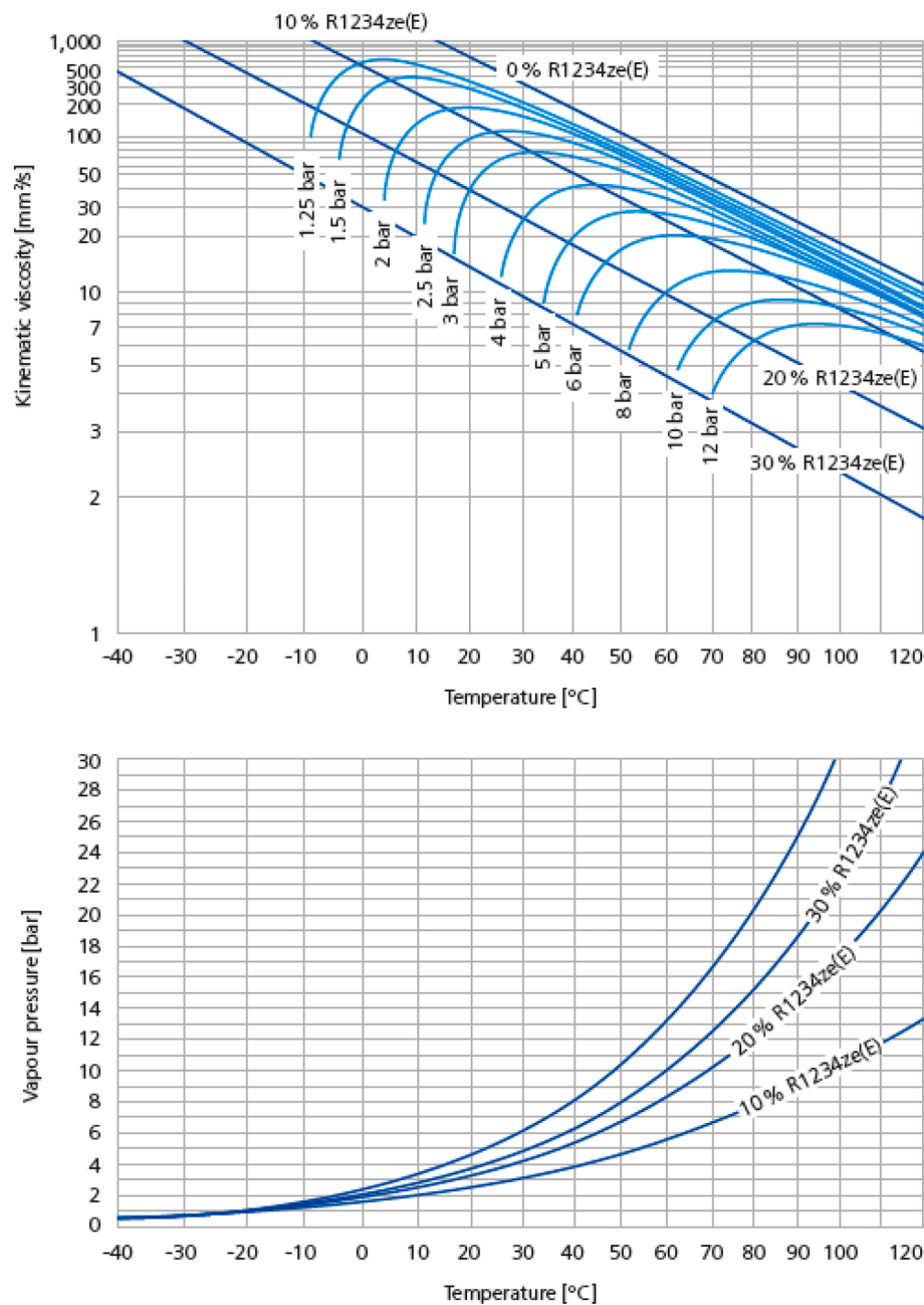
Fig. 20. Daniel plot of RENISO TRITON SE 170 (POE) with R1234ze(E) [78].
