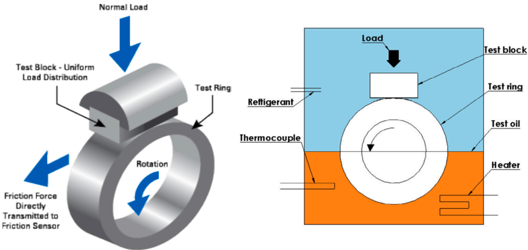
Fig. 5. A CAD-illustration of a block-on-ring wear tester (left) [101] and an illustration of the one used by Gorny et al. (right) [100].
