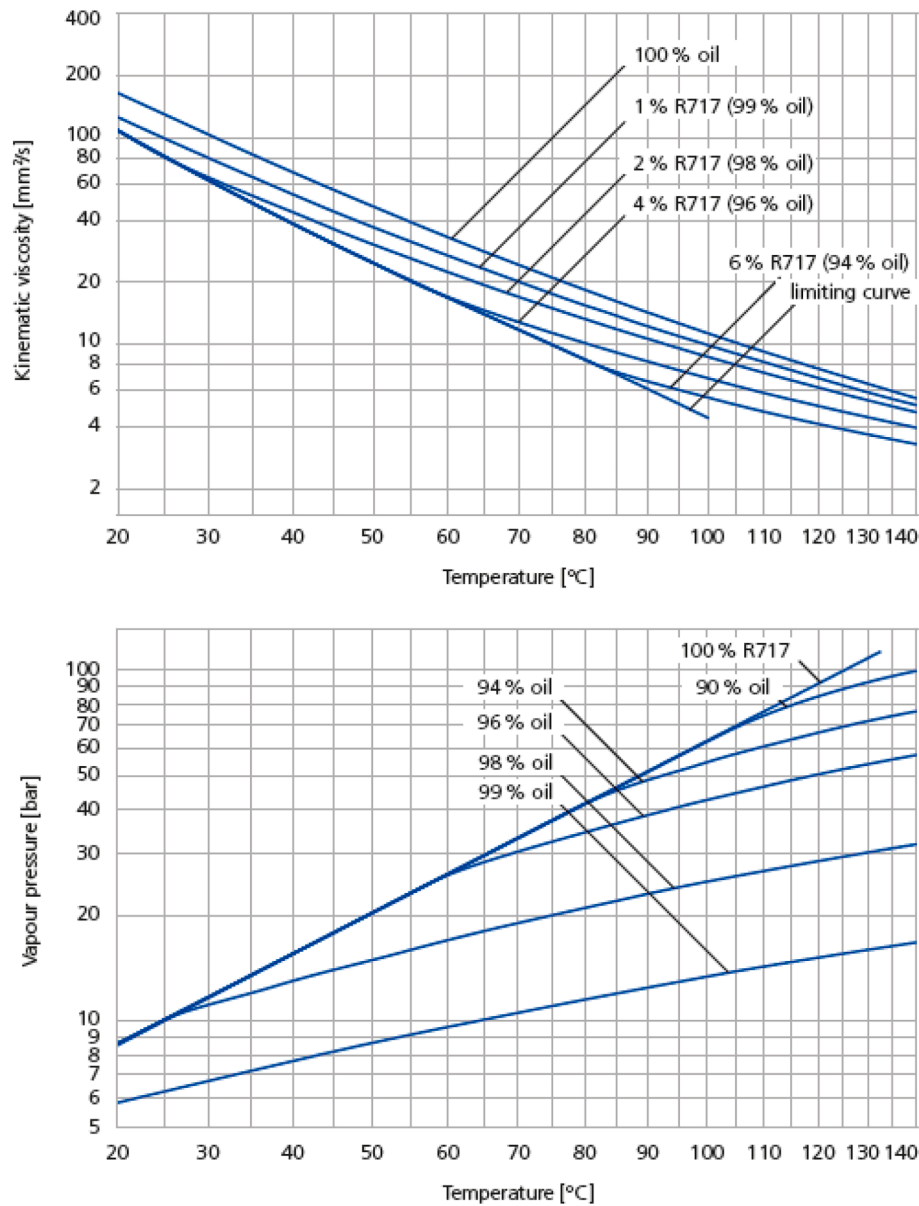
Fig. 23. Daniel plot for RENISO SYNTH 68 and R717 mixture [78].
