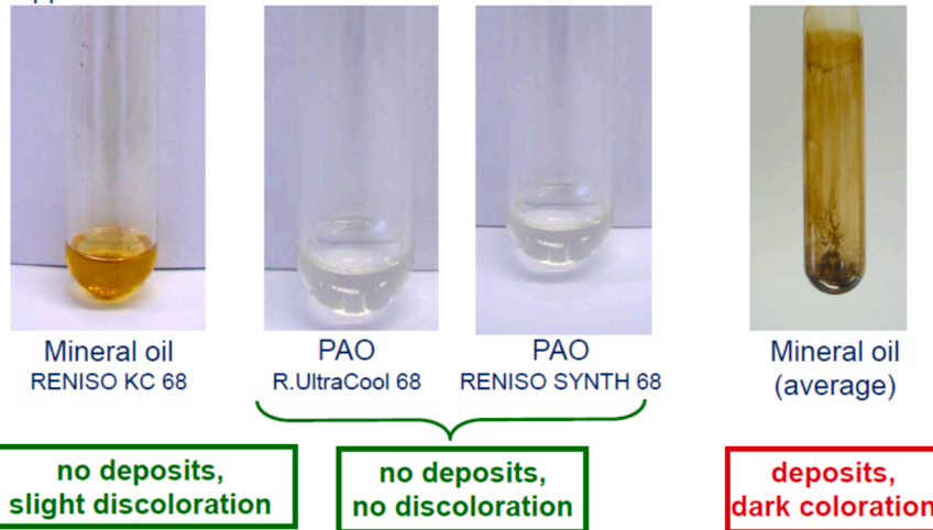
Fig. 21. Sealed tubes tests done at 120 °C for MO and PAO in combination with Ammonia [159].
