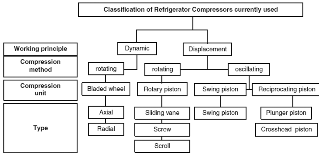
Fig. 2. Classification of refrigeration compressors according to their operation mode [20].
