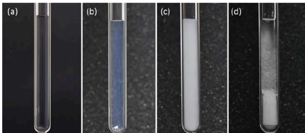
Fig. 8. Different miscibility behaviours of an oil/working medium mixtures in glass tubes [129].
