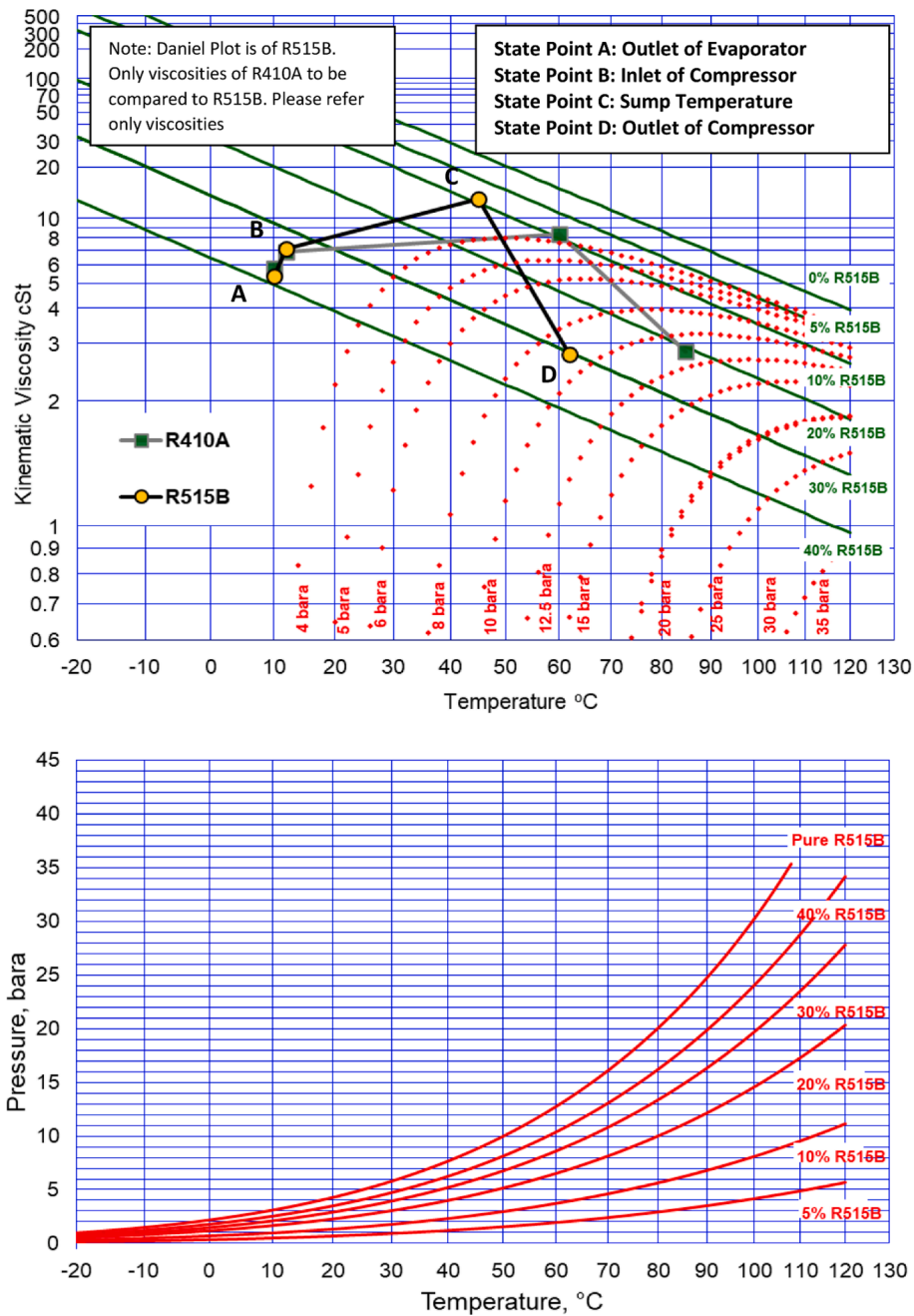
Fig. 18. Daniel plot for R515B with POE32 over the temperature range -20 – 120 °C [137].
