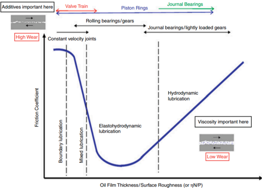
Fig. 4. Stribeck curve [79].
