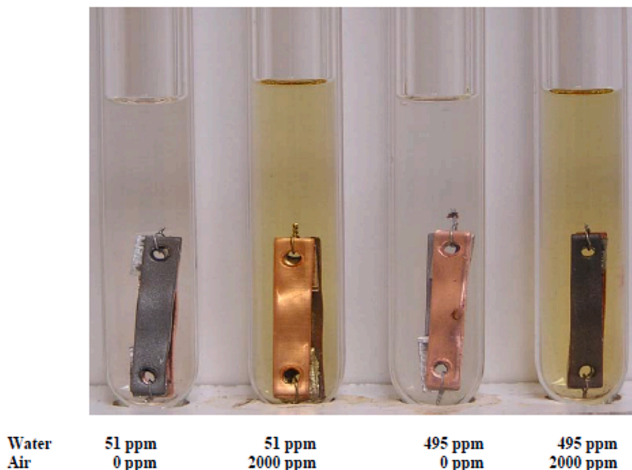
Fig. 11. Picture of sealed tubes containing HFO-1234yf/POE mixture with copper, steel, and aluminium strips [133].
