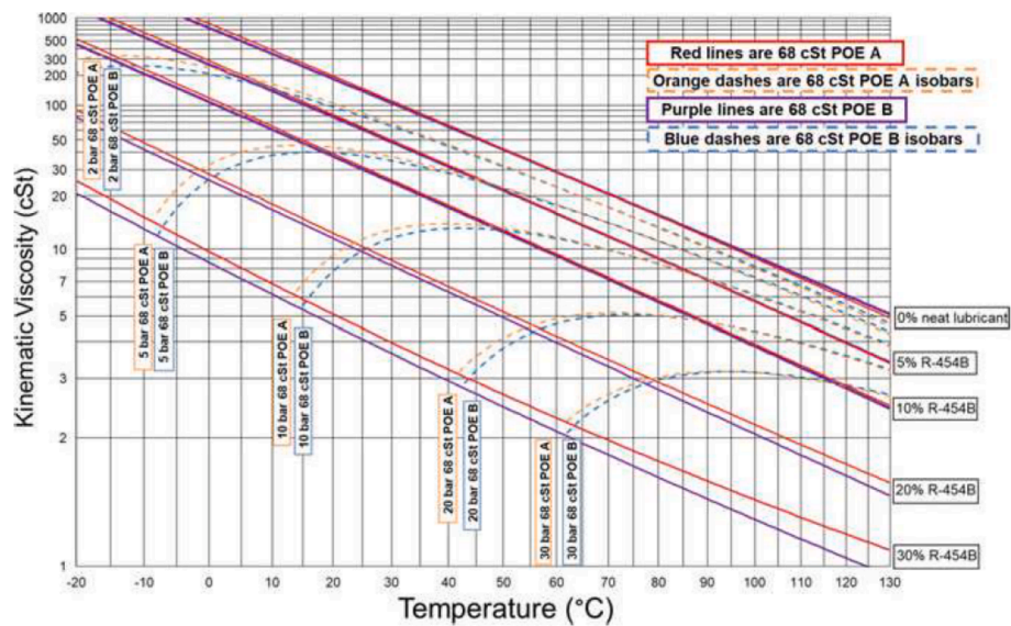
Fig. 15. Daniel plot for the two POE oils mixtures with R454B [129].
