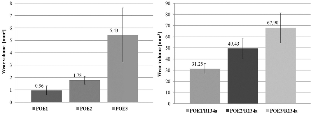
Fig. 6. Wear volume results after the tests with only POE oil and with POE/R134a mixtures [98].
