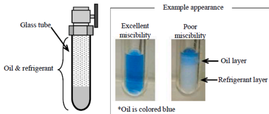
Fig. 9. Illustration (left) and picture (right) of the determination of the phase separation temperature [130].
