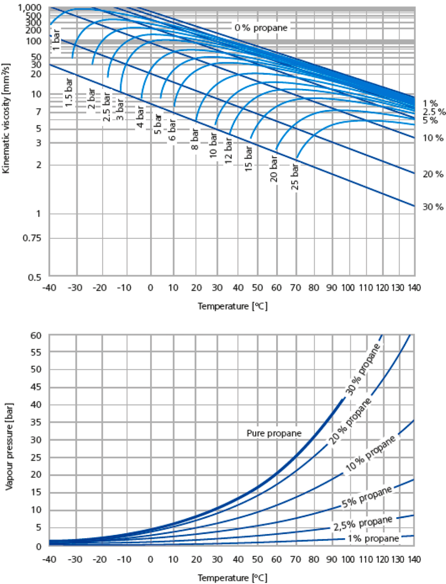
Fig. 12. Daniel plot for a PAG/R290 mixture [78].
