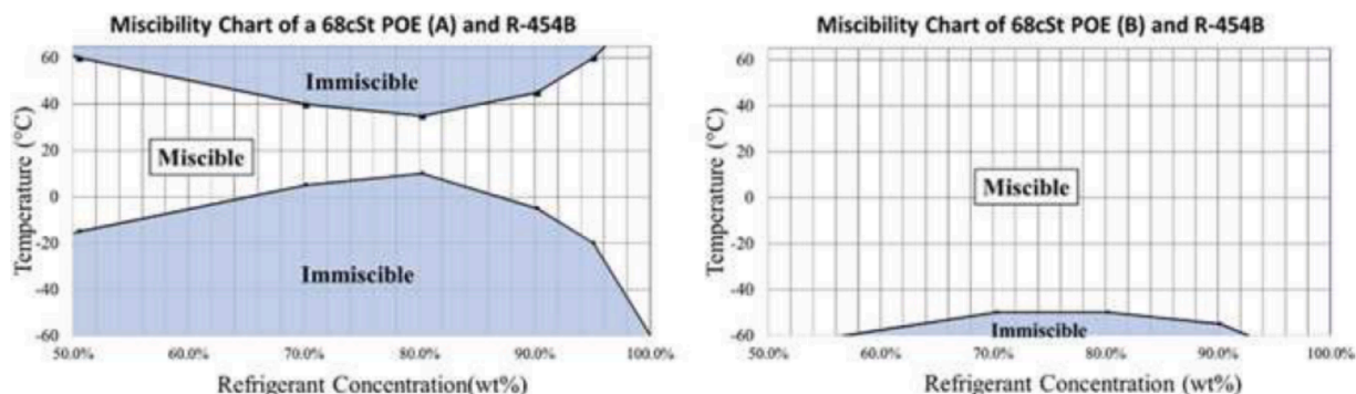
Fig. 14. Miscibility graphs for two different POE oils with R 454B [129].
