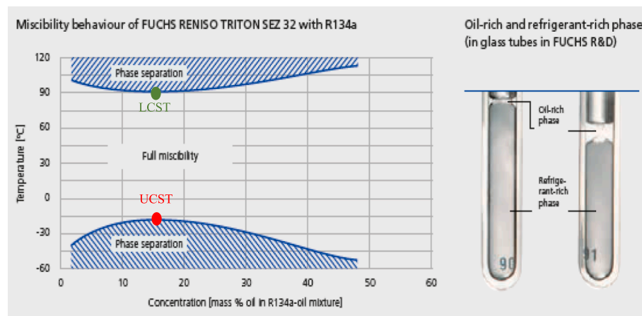
Fig. 7. Miscibility of R134a and POE oil [78].
