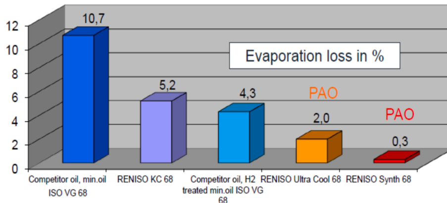
Fig. 22. Comparison of the evaporation losses for MO and PAO [159].
