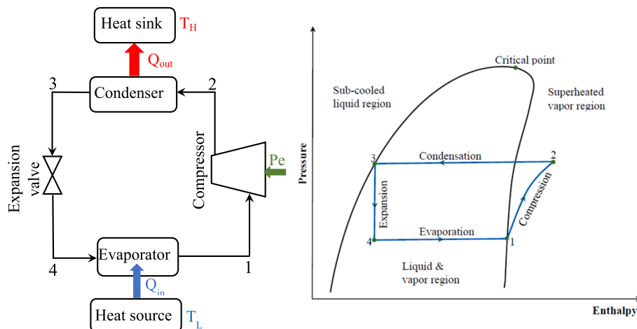
Fig. 1. Schematic of a compression heat pump (left), p-h diagram of the compression cycle (right).
