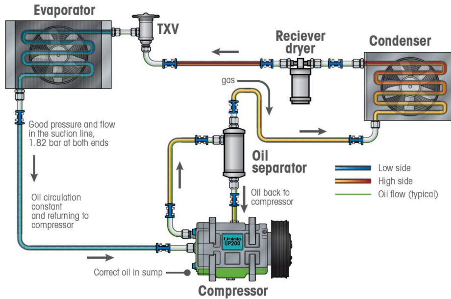
Fig. 3. Illustration of a heat pump system where an oil separation system is used[63].
