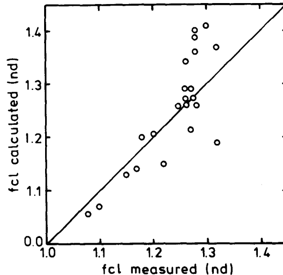
Fig. 5 Correlation between measured and calculated surface area factor using the cylinder model.
