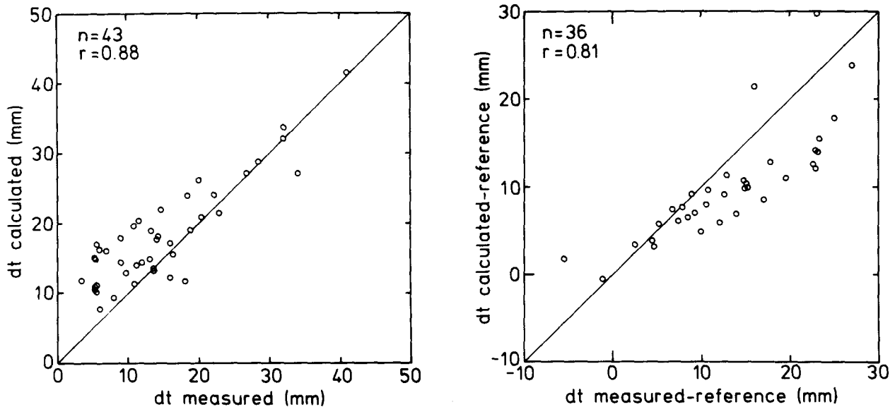
Fig. 9a Correlation between measured and calculated total water vapour resistance, using the regression equations on activity and wind.
