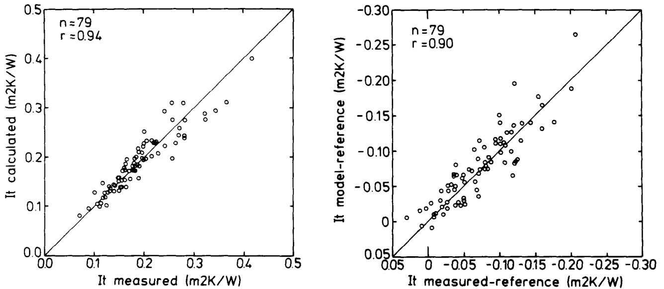
Fig. 7a Correlation between measured and calculated total insulation using the regression equations on activity and wind.
