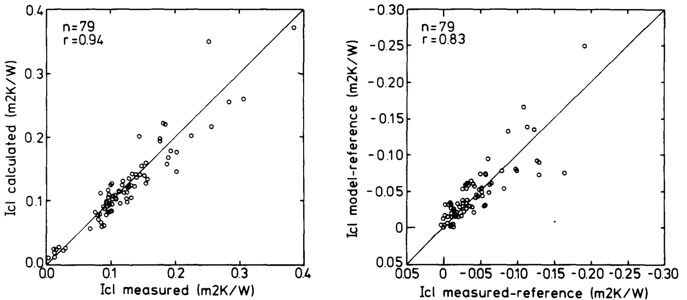
Fig. 8a Correlation between measured and calculated intrinsic insulation using the regression equations on activity and wind.
