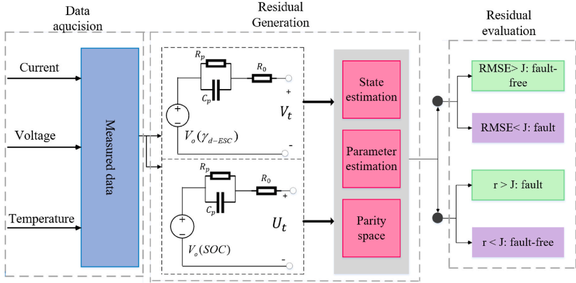
Fig. 19. Model-based fault detection procedure in LIBs [1].
