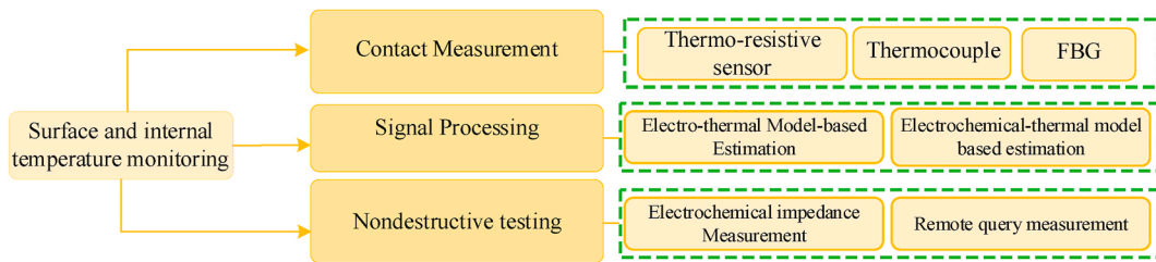
Fig. 17. Surface and internal temperature measurement methods applicable for the battery system.
