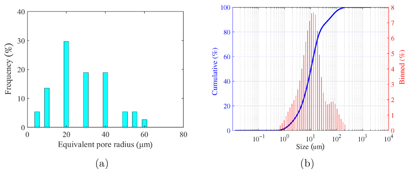
Figure 5. (a) The distribution of equivalent pore radius using SEM images; (b) Particle size distribution of calcite crystals.
