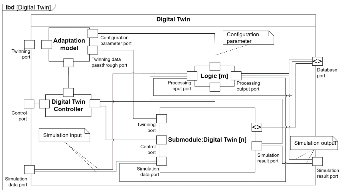
Figure 24 Logical components and communication of the DT
