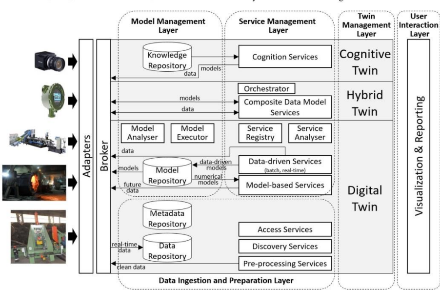
Figure 8 Architecture for a “Cognitive Twin” according to Aburru et al. [22].
