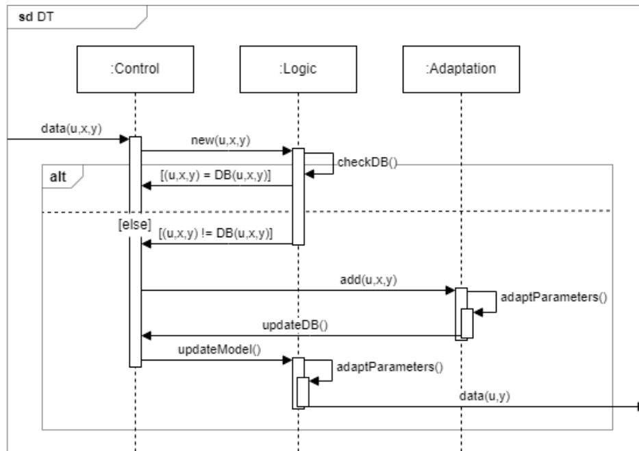
Figure 34 Sequence diagram of DT components.
