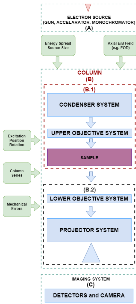
Figure 4 - Overview of Components Targeted for Sub Use Case 1
