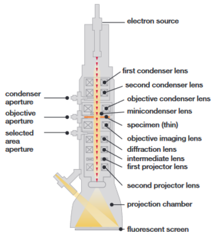
Figure 1: Structure of Transmission Electron Microscope
