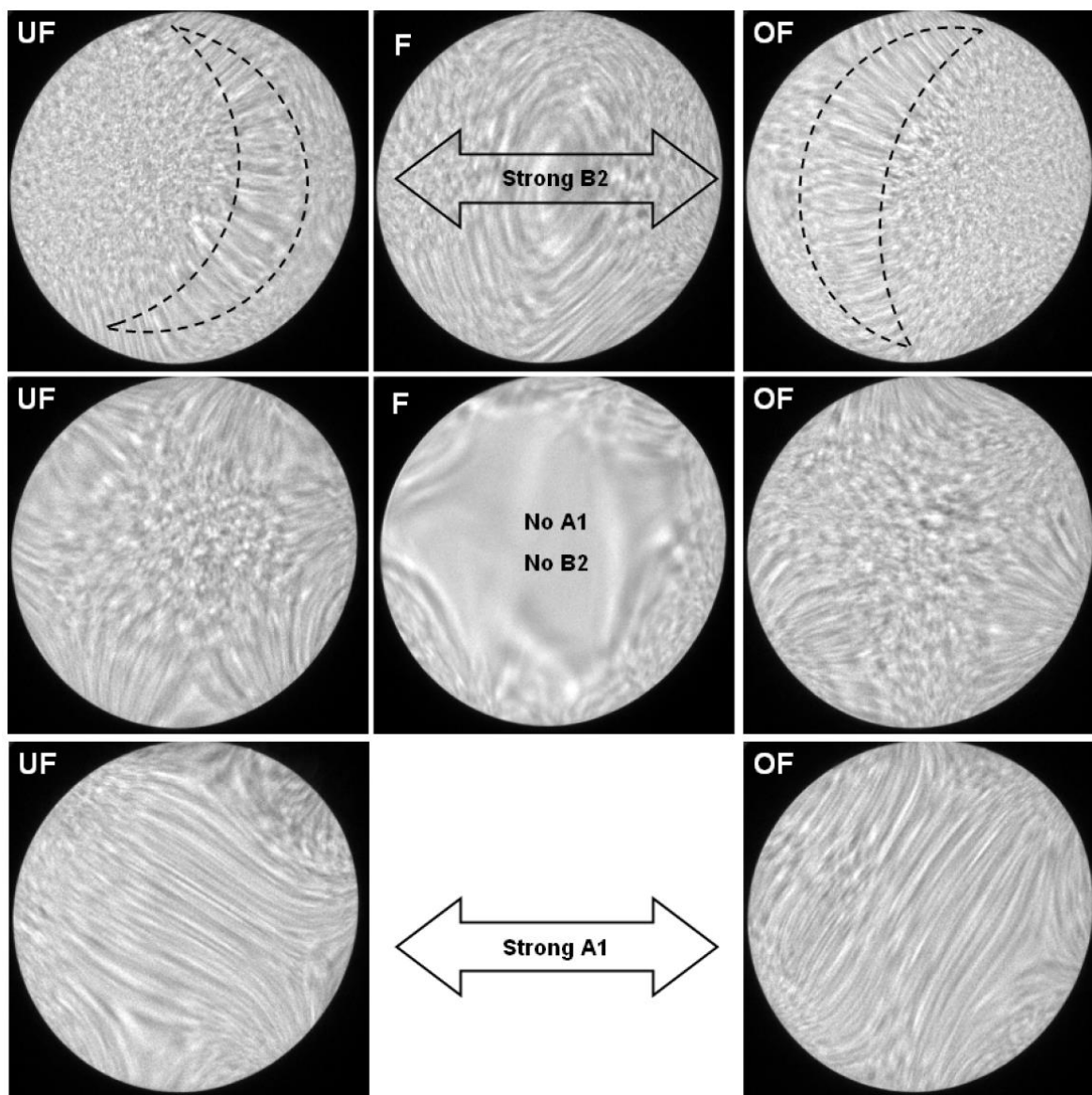
Figure 3: Illustration of Ronchigram features as a function of different aberrations. OF stands for over focus, UF for Under focus. [1]
