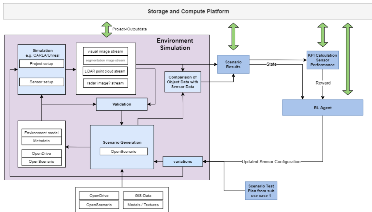
Figure 11 - Process Overview Sub Use Case 2
