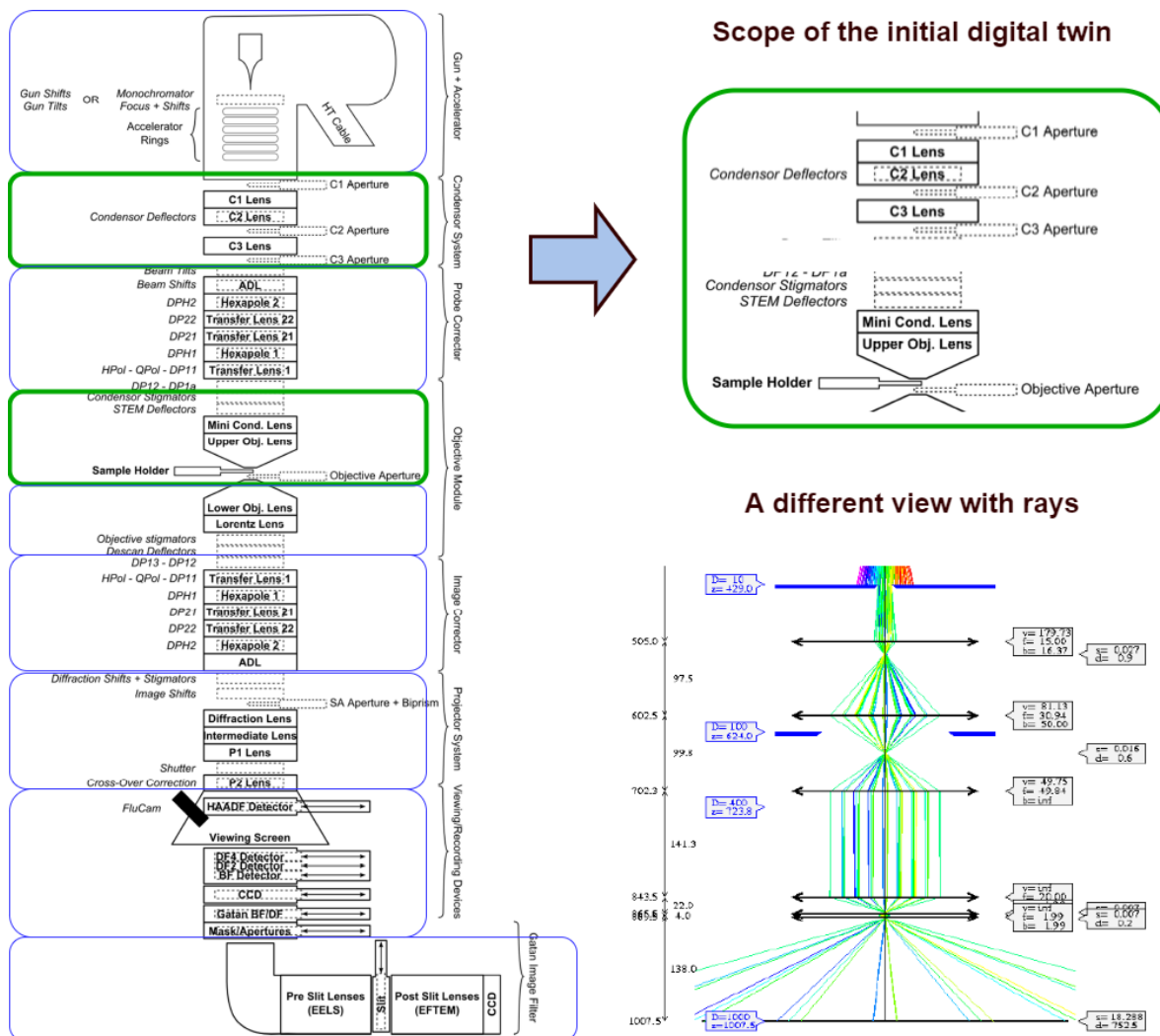
Figure 6 - Electron Microscope Components Included in the Digital Twin
