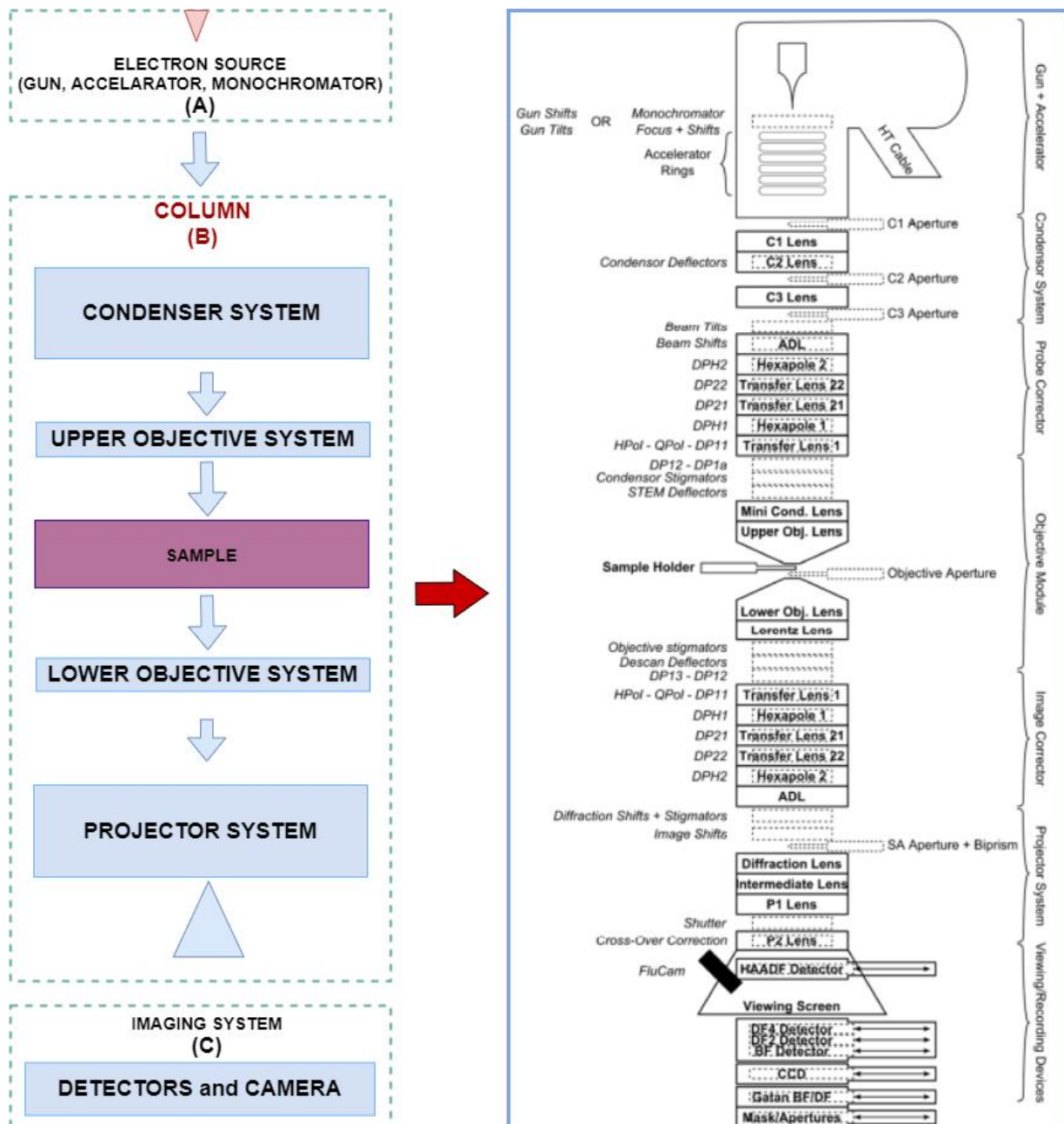
Figure 2: Schematic View of Electron Microscope Components
