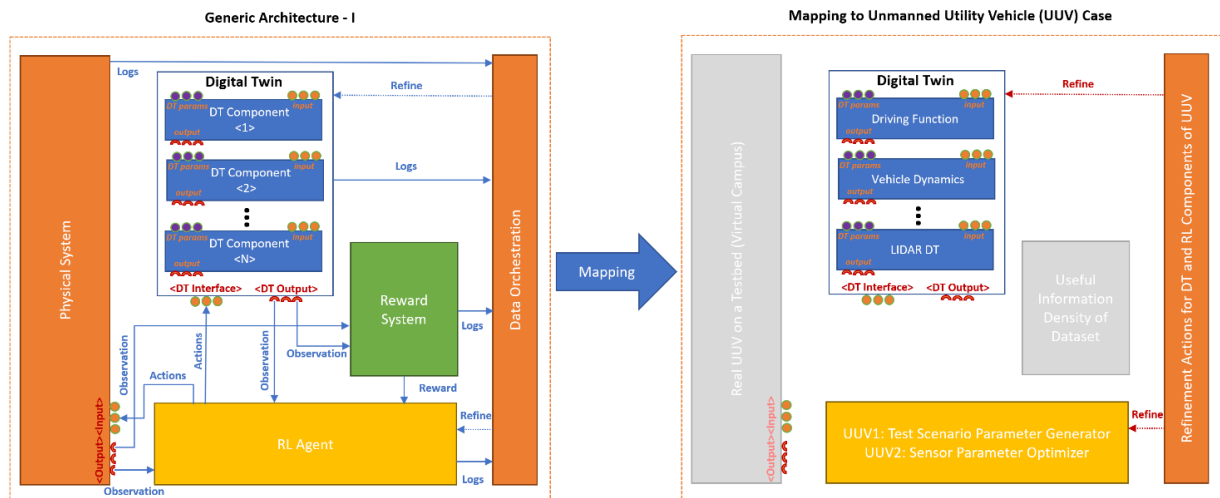
Figure 14 High-level architecture for the fine-tuning phase of the UAV use case.
