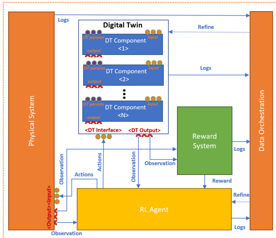
Figure 8 High-level architecture.
