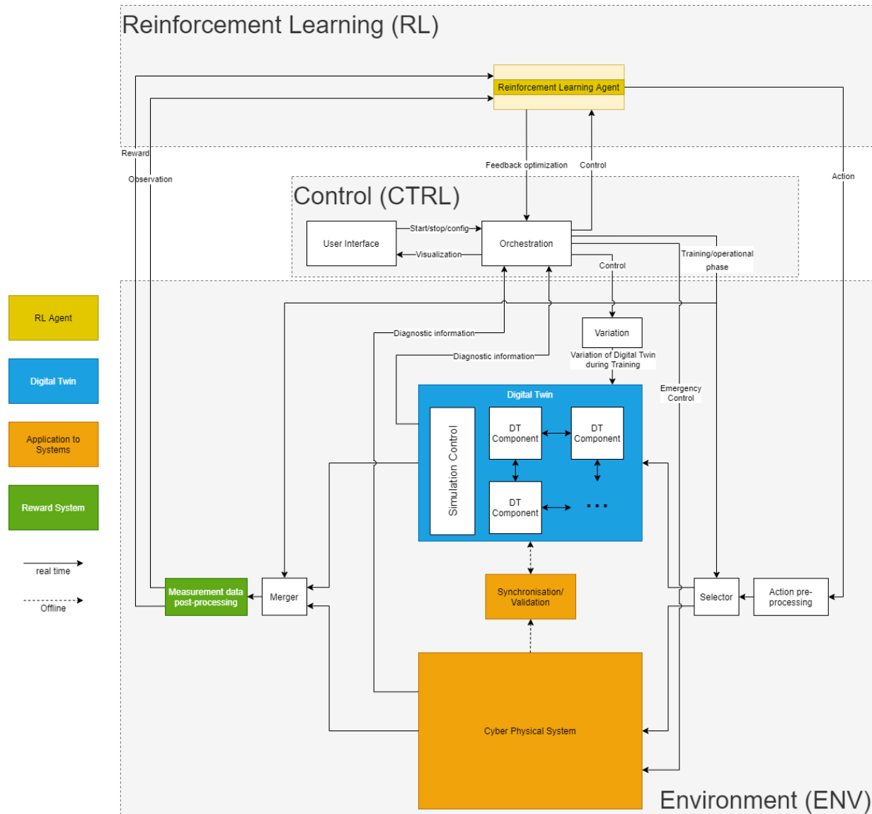
Figure 15 Detailed architecture.
