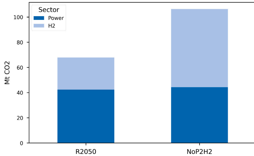
Fig. 16. EU CO 2 emissions for the electricity.
