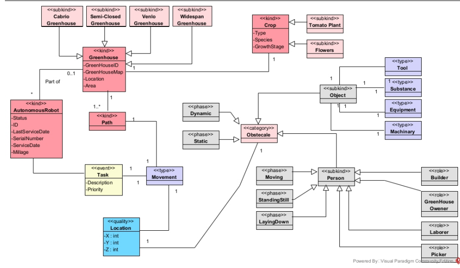
Figure 3. Greenhouse environment focused view.
