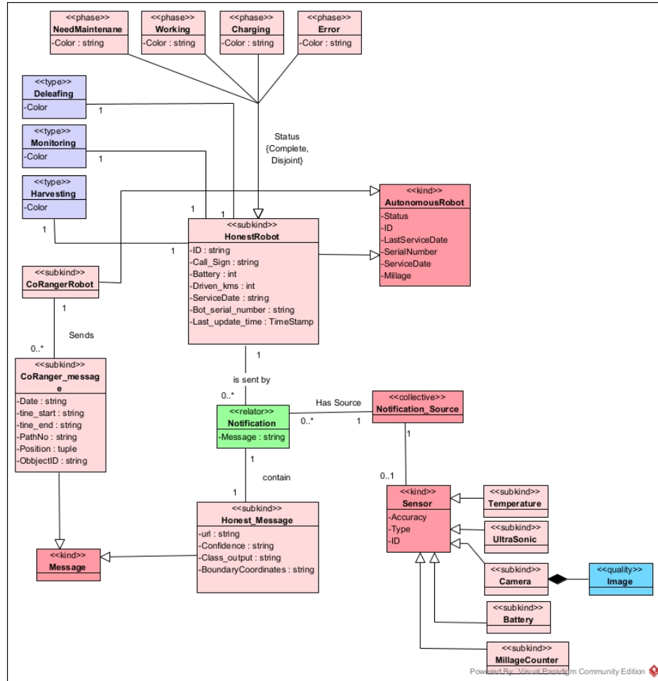
Figure 2. Autonomous system focused view.
