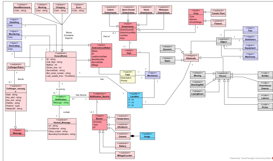
Figure 1. CGO-Robot reference ontology in OntoUML.
