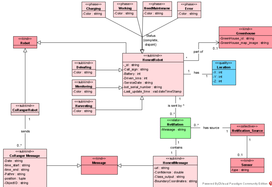
Figure 4. OntoUML test data.
