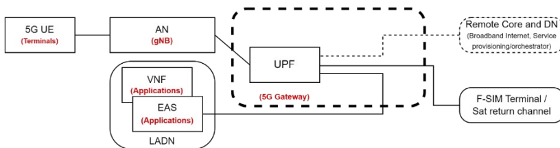
Figure 5: 5G gateway for the DTE use case.
