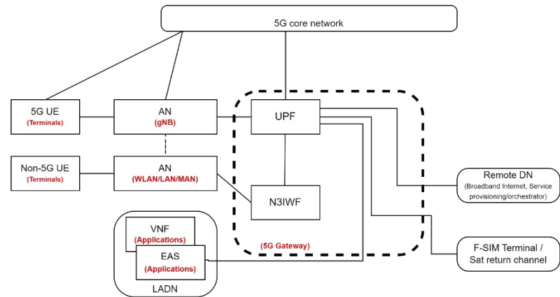
Figure 6: 5G gateway for the DTV maritime use case.
