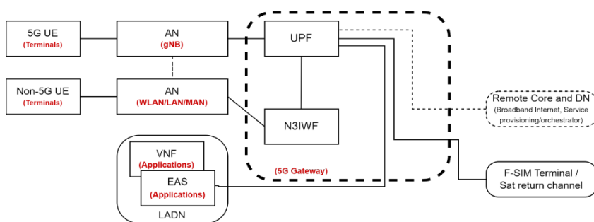
Figure 4: 5G gateway for the DTH use case.
