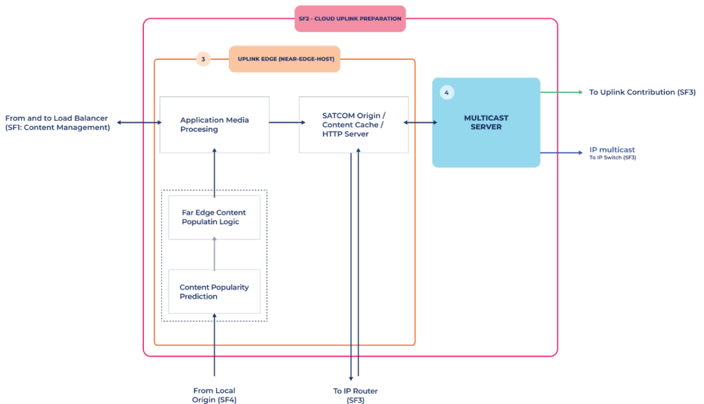
Figure 2: Architectural elements of system function 2, covering the Cloud Uplink Preparation. The numbers 3 and 4 refer to Figure 1.
