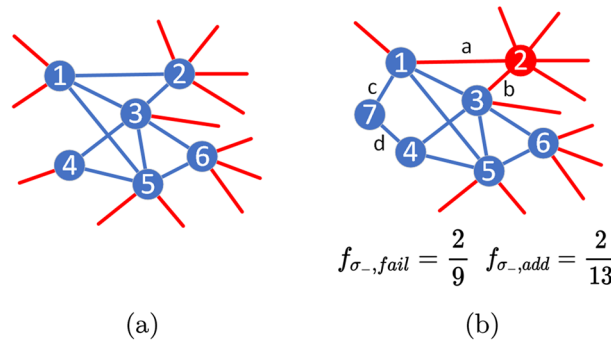
Fig. 5 Schematic representation of the neighbor opinion changing process of the G_{\sigma_-} subgraph. The colors of the links shows whether the link is connecting to a \sigma_- node (blue) or a \sigma_+ node (red). a State of the G_{\sigma_-} subgraph at time t . b State of the G_{\sigma_-} subgraph at time t + 1 . Node 2 changes its opinion and be removed from G_{\sigma_-} subgraph. Node 7 changes its opinion and be added to G_{\sigma_-} subgraph
