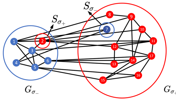
Fig. 4 State of a NCO system as in Fig. 3, but at time t = t + 1 . Node 2 changes its opinion from \sigma_- to \sigma_+ , and node 7 changes its opinion from \sigma_+ to \sigma_- . Sets S_{\sigma_+} and S_{\sigma_-} consist of node 2 and node 7, respectively
