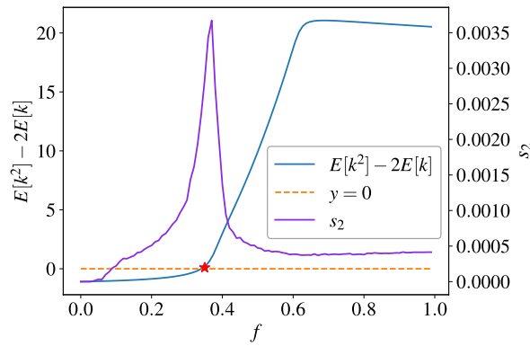
(c) Configuration model with N = 10000 and a random degree distribution.
