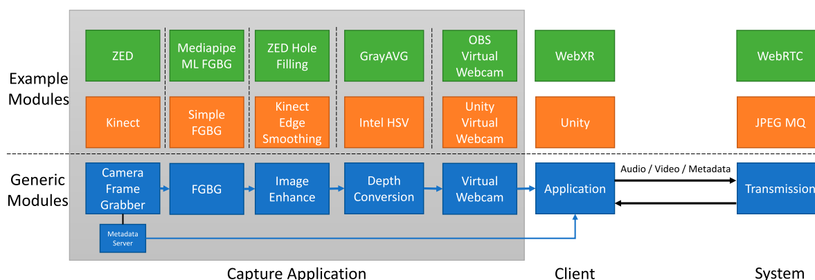
FIGURE 1 Modular capture architecture.
