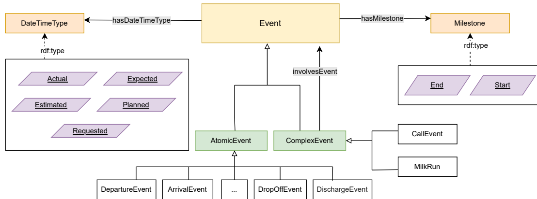
Figure 2: High level diagram of the Event module. For conciseness, the diagram leaves out the relation depicted in the modularisation and the full AtomicEvent taxonomy. Legend: Rectangles represent classes , with the main class in yellow, the first degree of the event taxonomy in green, the second degree of the event taxonomy in white, and other classes in orange; parallelograms (purple) represent enumerated individuals ; arrows with white tips represent rdfs:subclassOf relations; and other arrows represent the indicated relations.
