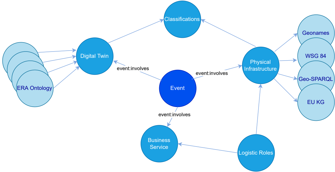
Figure 1: Modularisation of the FEDeRATED Semantic Model. The Event Module is dark blue, other modules are blue, and external ontologies are light blue.
