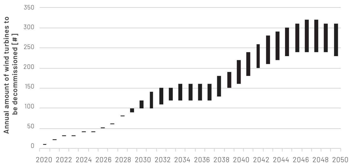
Figure 4 Projection of annual amount of wind turbines to be decommissioned [#] (distribution is based on lifetime variation from 20-25 years to 25-30 years)
