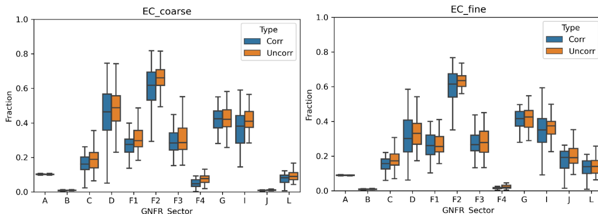
Figure 7. Boxplots (95% confidence interval) of the spread in the EC fraction in fine (PM 2.5 ) and coarse (PM 10 ) PM from the correlated (Corr) and uncorrelated (Uncorr) LIM ensemble (N=50).
