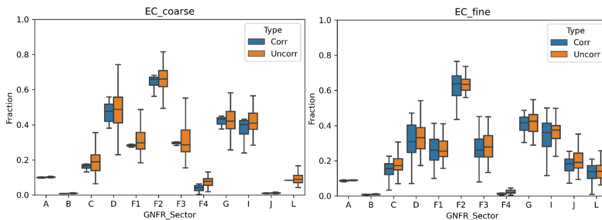
Figure 8. As Fig. 7, but for the MET ensemble.
