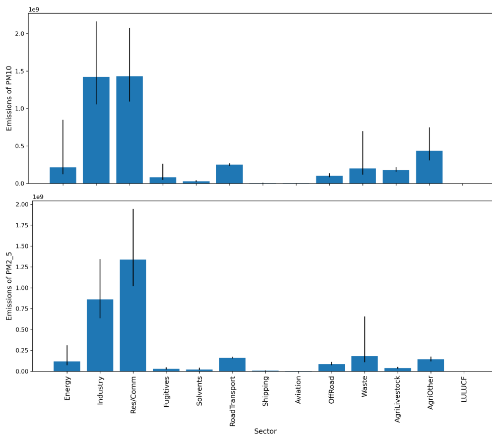
Figure 4. Emissions of PM10 and PM2.5 (kg/yr) per sector (for all countries combined) and error bars representing the standard deviations.
