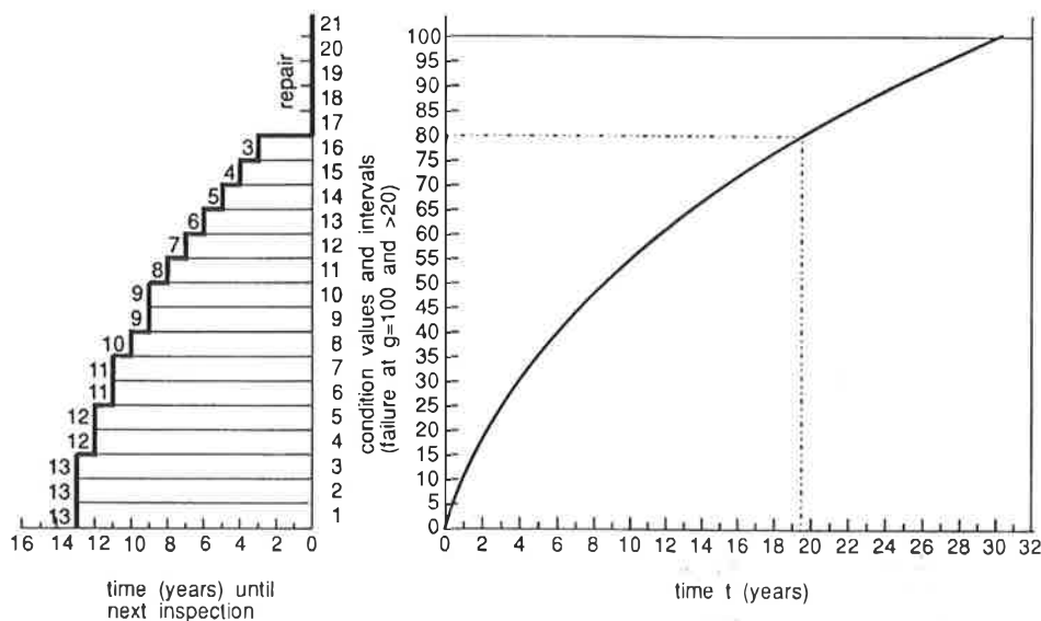
Fig. 3. Optimal condition-based inspection and repair strategy for a carbonation process (see table 1, part 1).
