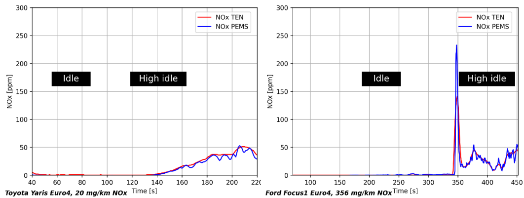
Figure 5.2: NO x concentration during PTI emissions test displayed for a vehicle with low emissions (left) as well as a more than 15 times higher NO x emitter (right). The height of the stabilized NO x concentration levels under low and high idle are indistinguishable between left and right.
