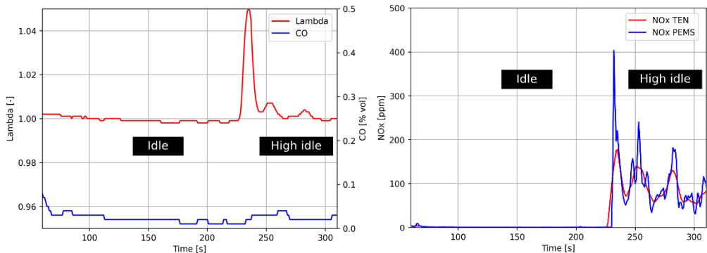
Figure 4.3: Raw data from the 5-gas analyser during a stationary PTI test of the Renault Twingo, on the left is CO in blue and Lambda in red, on the right is NO x measured with PEMS and a TEN 5-gas tester.
