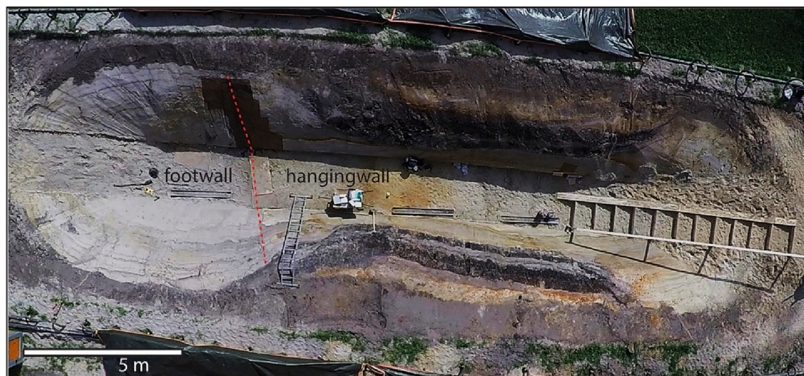
Fig. 4. Overview photo of the trench. The red dashed line indicates the fault. The prominent dark gray to black deposits on the hangingwall are the organic infill of the man-made paleo-channel. The length of the trench is about 25 m and the width 8 m. (For interpretation of the references to colour in this figure legend, the reader is referred to the web version of this article.)
