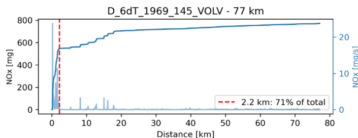
Figure 4.1: NO x emissions during a PEMS+ cold trip by a Euro 6d-Temp diesel vehicle with taxonomy code D_6dT_1969_145_VOLV as per [uCARE 2021]. The red dashed line indicates where the point after which the exhaust aftertreatment system is working well: the cumulative NO x emissions (dark blue line) plateau after this point.
