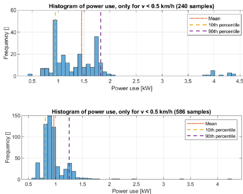
Figure 6.2: Example of power use while stationary of the VW ID.3 in a chassis dyno test of type 'WLTC, cold, def' (top) and the same vehicle in an on-road PEMS test of type 'PEMS, regular, cold' (bottom).
