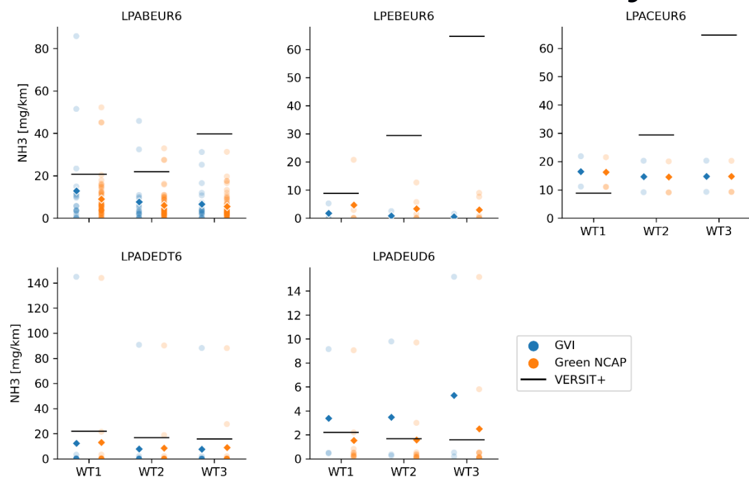
Figure A.3: Average NH 3 emissions calculated per urban (WT1), rural (WT2) and motorway (WT3) VERSIT+ road type, as calculated per vehicle (round points) and averaged per GVI or Green NCAP data set (diamond points). Each pane shows the relevant VERSIT+ classes separately.
