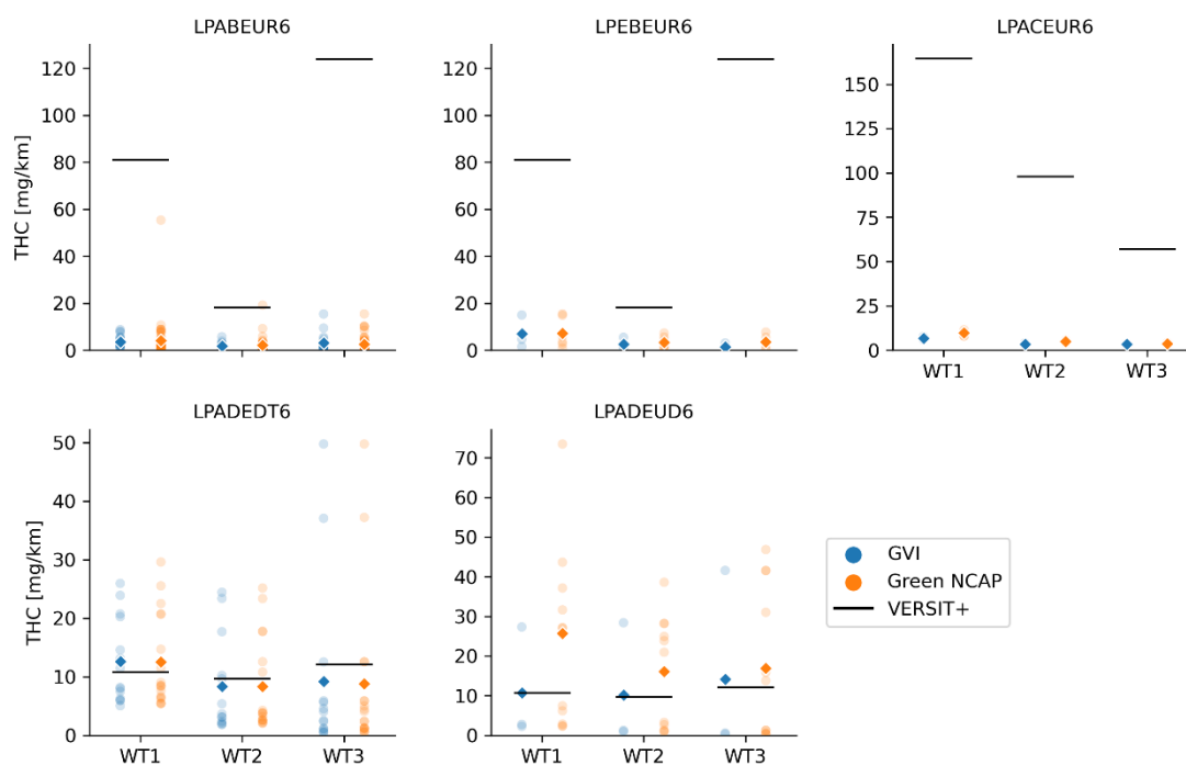
Figure A.4: Average THC emissions calculated per urban (WT1), rural (WT2) and motorway (WT3) VERSIT+ road type, as calculated per vehicle (round points) and averaged per GVI or Green NCAP data set (diamond points). Each pane shows the relevant VERSIT+ classes separately.
