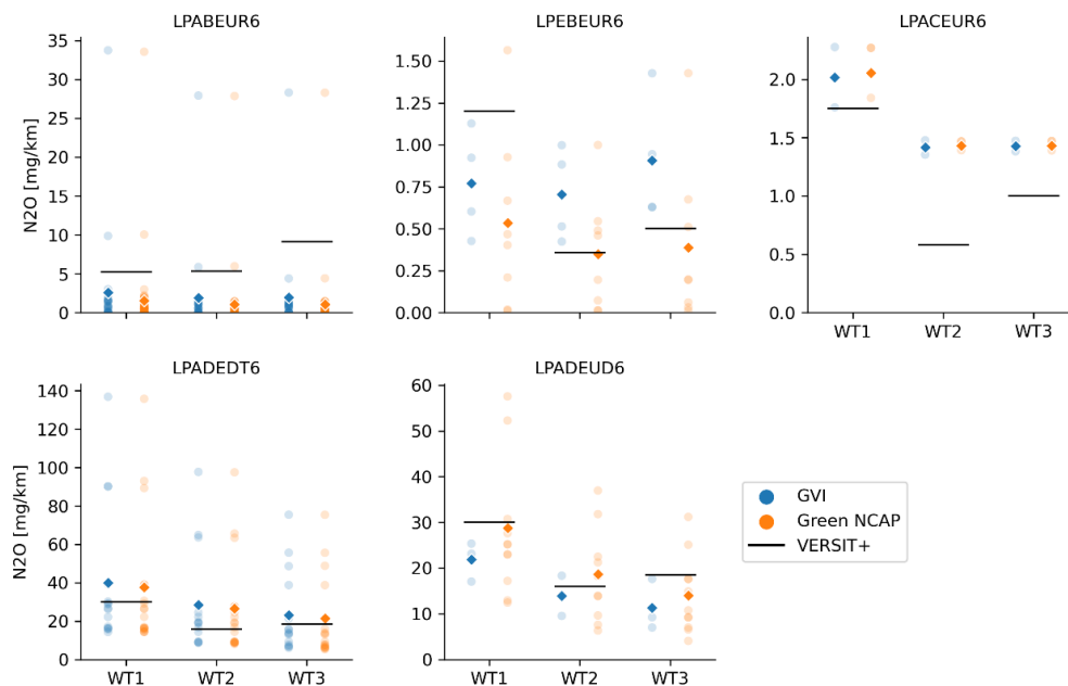
Figure 4.5: Average N 2 O emissions calculated per urban (WT1), rural (WT2) and motorway (WT3) VERSIT+ road type, as calculated per vehicle (round points) and averaged per GVI or Green NCAP data set (diamond points). Each pane shows the relevant VERSIT+ classes separately.
