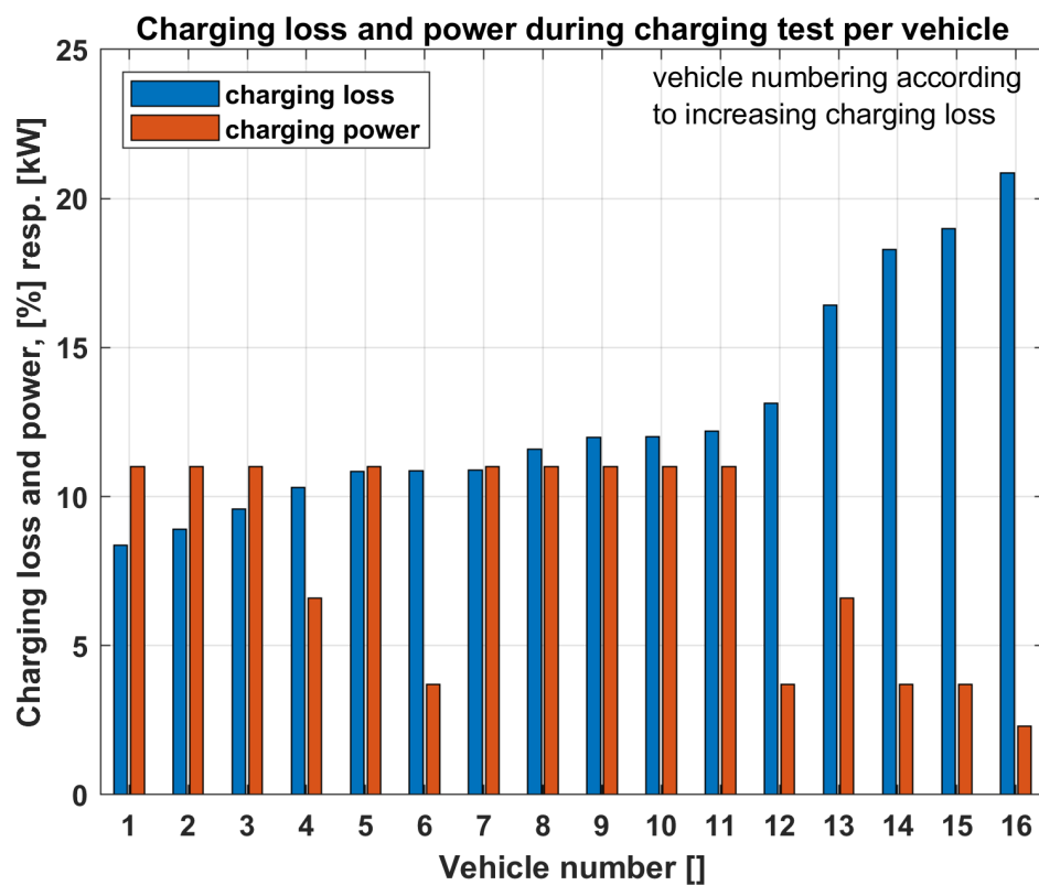
Figure 6.1: Charging losses (blue bars) as measured and power used (red bars) during charging of the 16 BEVs.
