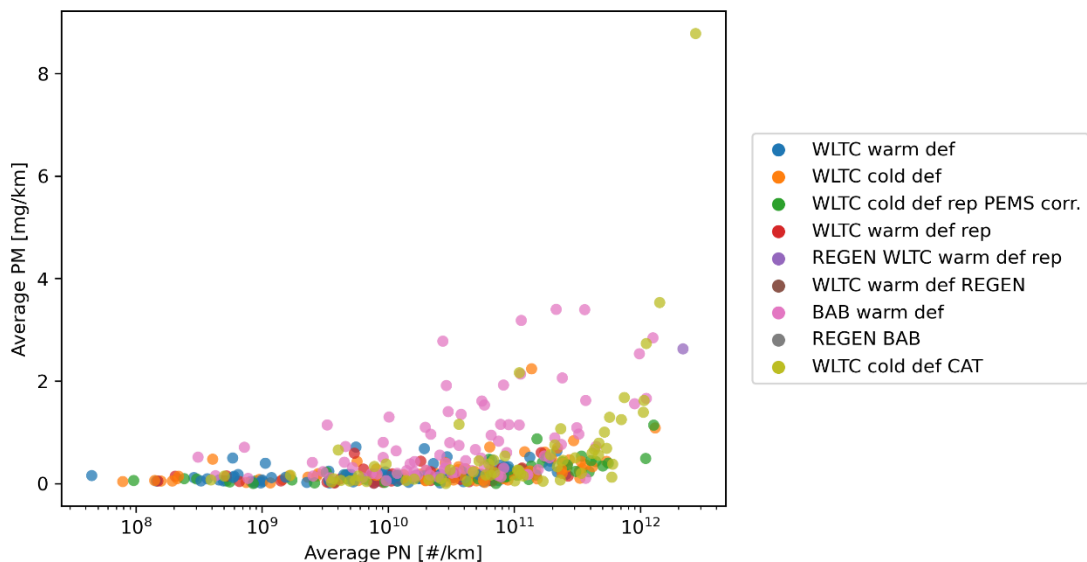
Figure 3.7: Average PM emissions as a function of the corresponding PN emissions. The colours indicate the trip type. Trips prefixed with 'REGEN' are trips during which a DPF regeneration occurred.
