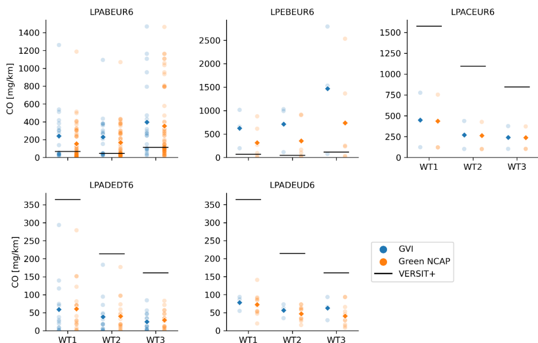
Figure A.1: Average CO emissions calculated per urban (WT1), rural (WT2) and motorway (WT3) VERSIT+ road type, as calculated per vehicle (round points) and averaged per GVI or Green NCAP data set (diamond points). Each pane shows the relevant VERSIT+ classes separately.
