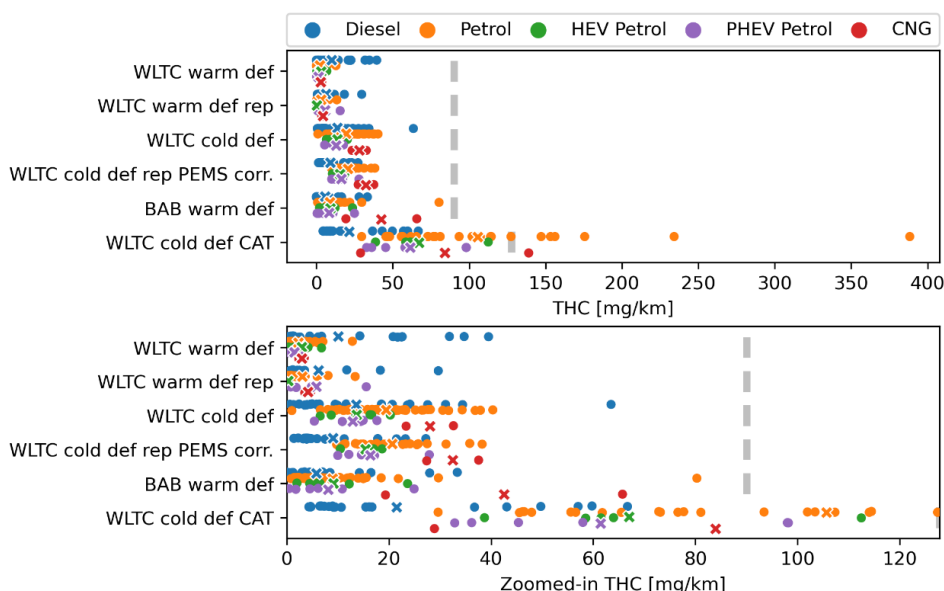
Figure 3.6: THC emissions as averaged over the entire trip. The top panel shows all data measured on the chassis dyno including the Green NCAP thresholds in grey. Averages per fuel type per test type are shown by crosses. The bottom panel shows the zoomed-in version of the top panel.
