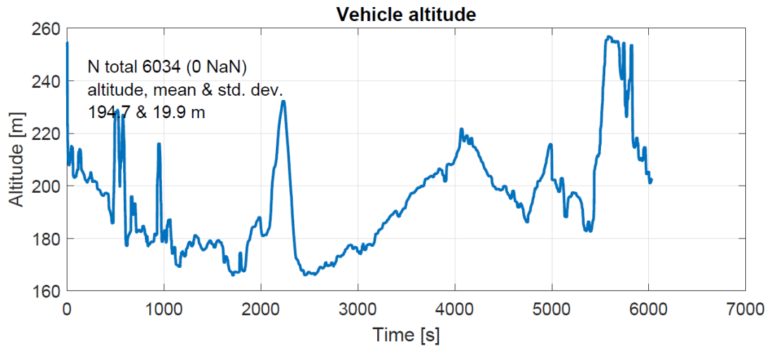
Figure 6.11: Elevation profile for the VW ID.3 in the on-road 'PEMS, regular, cold' test.
