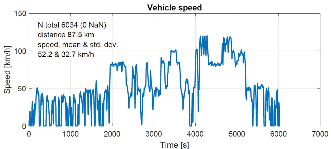
Figure 6.10: Vehicle speed for the VW ID.3 in the on-road ‘PEMS, regular, cold’ test.
