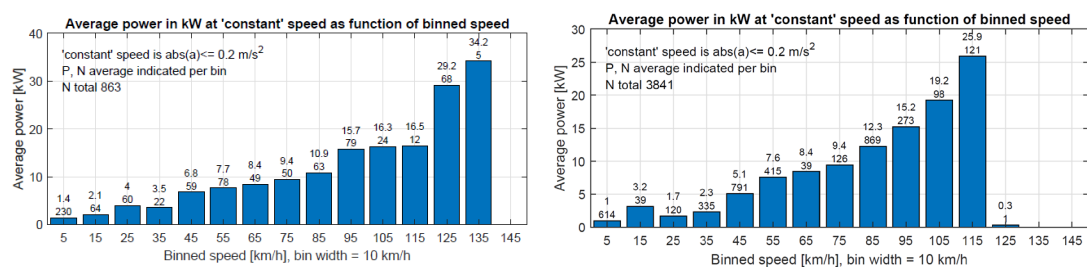
Figure 6.3: Example of average power use while driving at 'constant' speed of the VW ID.3 in a chassis dyno lab test of type 'WLTC, cold, def' (left) and an on-road PEMS test of type 'PEMS, regular, cold' (right). The two numbers above each bar are the average power and respectively the number of seconds averaged over for that bar.
