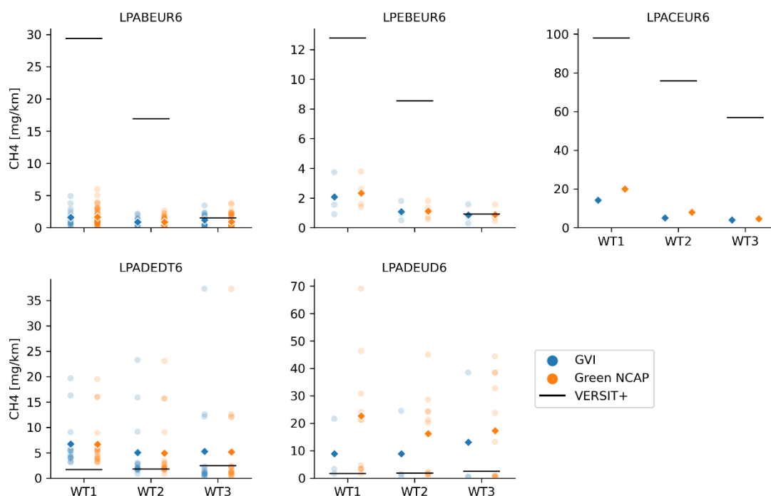
Figure A.5: Average CH 4 emissions calculated per urban (WT1), rural (WT2) and motorway (WT3) VERSIT+ road type, as calculated per vehicle (round points) and averaged per GVI or Green NCAP data set (diamond points). Each pane shows the relevant VERSIT+ classes separately. Note that CH 4 emissions were only measured for one of the CNG vehicles.
