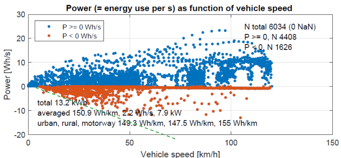
Figure 6.8: Power as function of vehicle speed for the VW ID.3 in the on-road 'PEMS, regular, cold' test.
