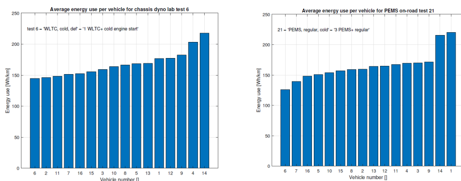
Figure 6.5: Two roughly similar tests compared: chassis dyno lab test 6 alias ‘WLTC, cold, def’ (left graph) and PEMS on-road test 21 alias ‘PEMS, regular, cold’ (right graph).
