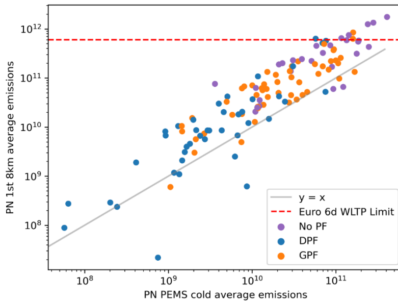
Figure 3.4: PN emissions as averaged over the first 8 km of a trip, as compared to the average over the entire trip. Blue points indicate diesel vehicles with DPF, orange petrol vehicles with GPF, and purple vehicles without a particulate filter. The dashed red line indicates the Euro 6d WLTP limit for PN.
