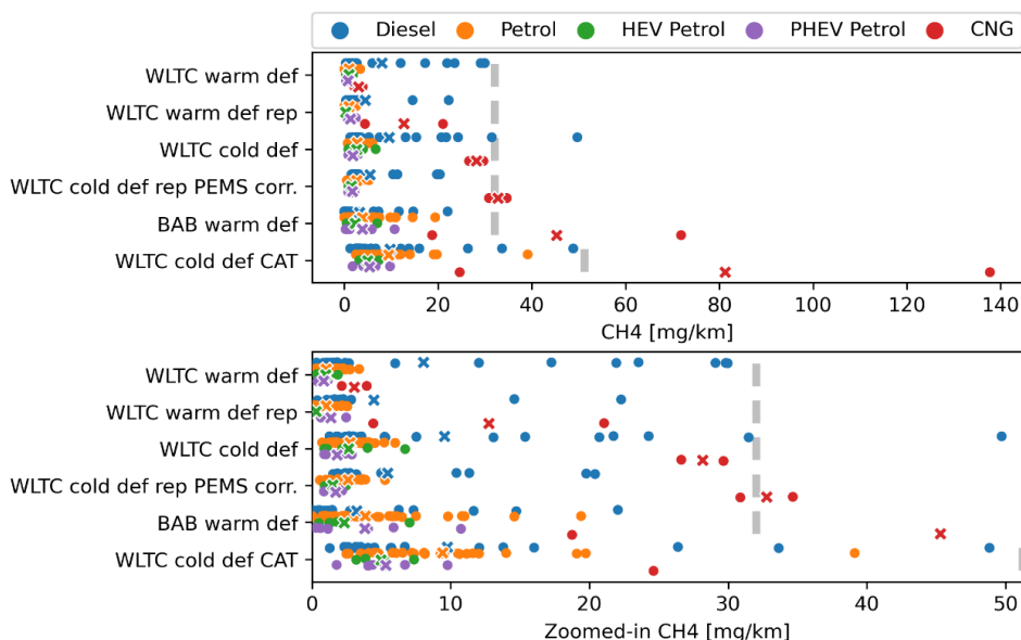
Figure 3.5: CH 4 emissions as averaged over the entire trip. The top panel shows all data measured on the chassis dyno including the Green NCAP thresholds in grey. Averages per fuel type per test type are shown by crosses. The bottom panel shows the zoomed-in version of the top panel.
