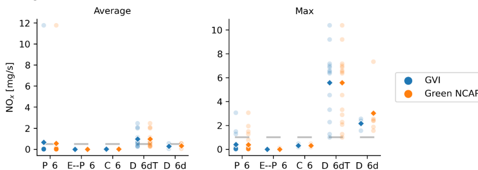
Figure 5.6: Average (left) and maximum (right) NO x emissions during the congestion test per vehicle (round points) and averaged per GVI or Green NCAP data set (diamond points). The Green NCAP thresholds are shown in grey.
