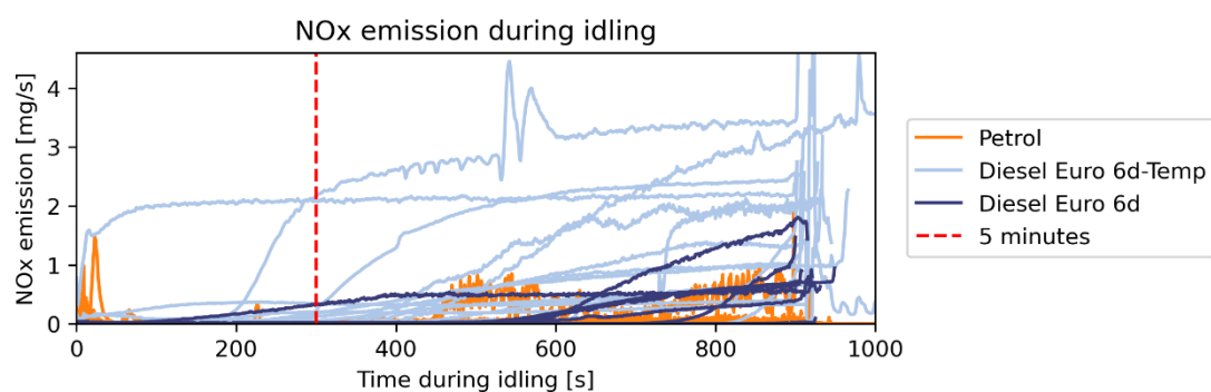
Figure 5.7: Instantaneous NO x emissions during a period of extended idling for a number of different petrol and diesel vehicles. The red line indicates five minutes, which is the maximum duration of idling allowed during an RDE test.
