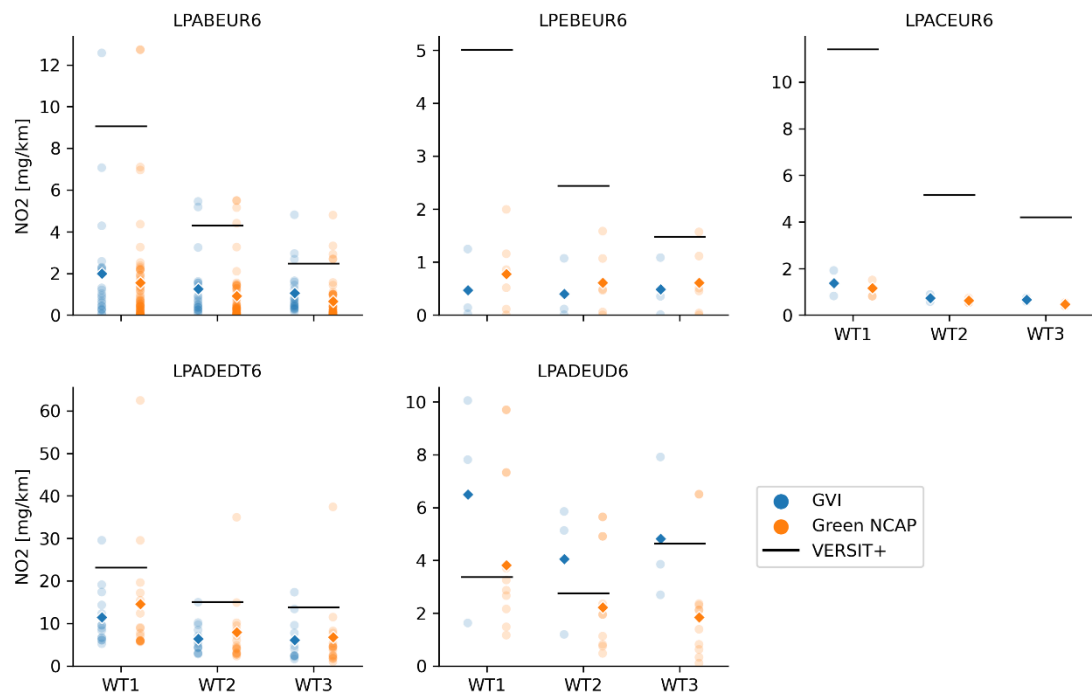
Figure A.2: Average NO 2 emissions calculated per urban (WT1), rural (WT2) and motorway (WT3) VERSIT+ road type, as calculated per vehicle (round points) and averaged per GVI or Green NCAP data set (diamond points). Each pane shows the relevant VERSIT+ classes separately.
