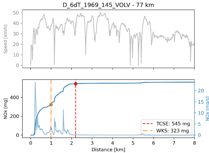
Figure 4.2: Speed (top) and NO x emissions (bottom) during the first eight kilometres of the PEMS+ cold trip shown in Figure 4.1. The red dotted line shows the distance at which the cold start is considered complete; the red dot shows the total cold start emissions (TCSE). The orange line indicates one kilometre; the sum of the emissions up to this point is used along with the average of the total trip (10 mg/km in this case) to calculate the point source representation of the cold start extra emissions (WKS, yellow dot).
