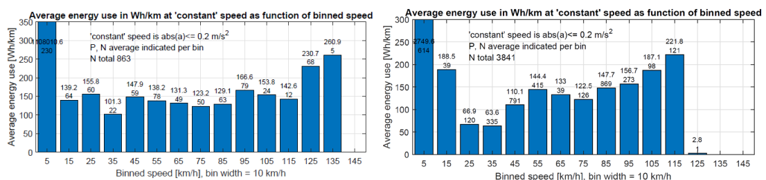
Figure 6.4: Again vehicle 5 driving at 'constant' speed but shown is now average energy per kilometre driven of the VW ID.3 in a chassis dyno lab test of type 'WLTC, cold, def' (left) and an on-road PEMS test of type 'PEMS, regular, cold' (right). The two numbers above each bar are the average power and respectively the number of seconds averaged over for that bar.
