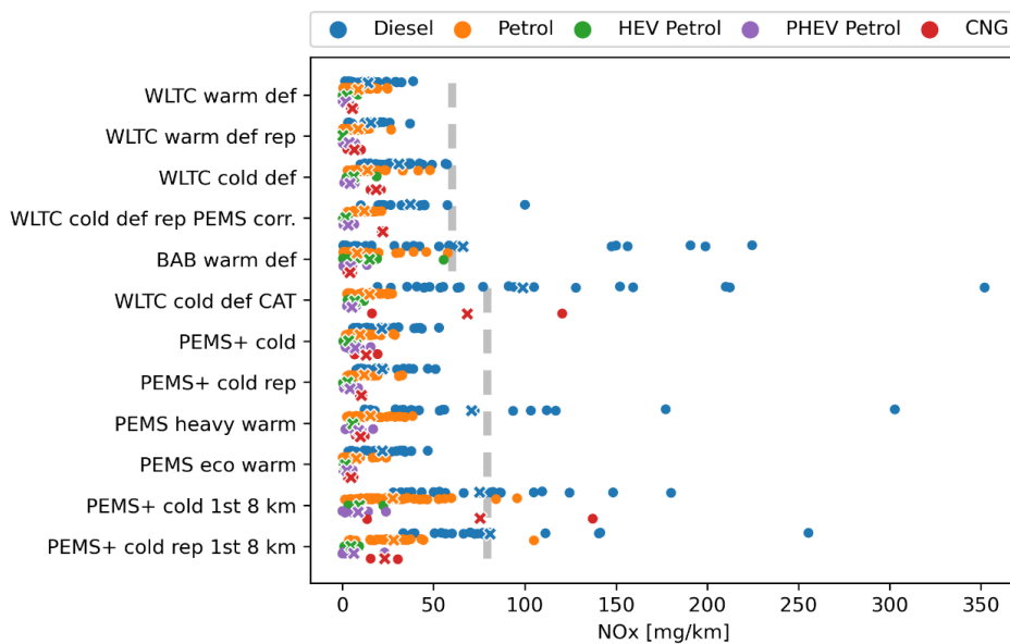
Figure 3.2: NO x emissions as averaged over the entire trip. The Green NCAP thresholds are shown in grey. Averages per fuel type per test type are shown by crosses.
