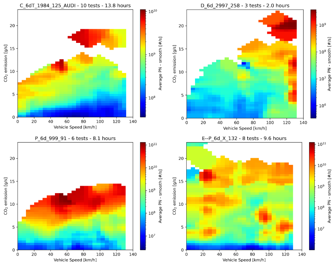
Figure 5.1: PN emissions as a function of vehicle speed and CO 2 emissions for four different vehicles as identified by their [uCARE 2021] taxonomy code. For cold trips, the data after the first kilometre is used.
