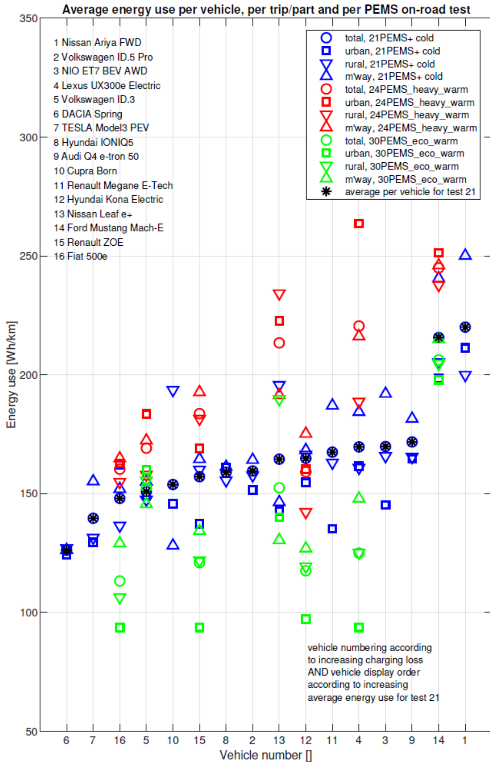
Figure 6.7: Average energy use (from battery) per vehicle per test, and per road type, for the PEMS on-road tests.
