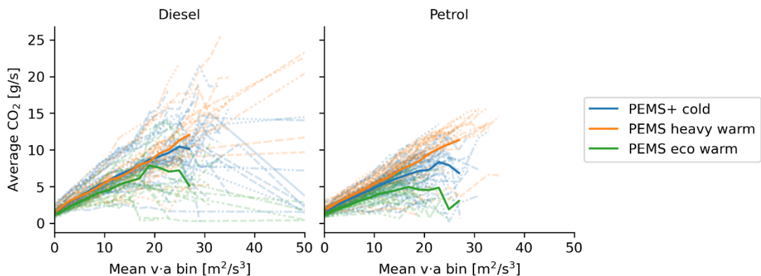
Figure 5.4: CO 2 emissions per v-a bin for diesel and petrol vehicles, as coloured by on-road test type. The bold lines show the averages of the relevant trips which are shown with the lighter dashed lines.
