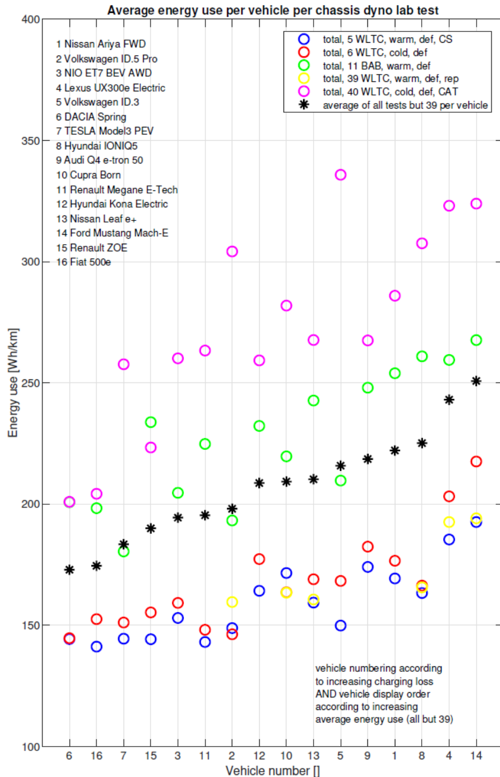
Figure 6.6: Average energy use (from battery) per vehicle per test for the chassis dyno lab tests.
