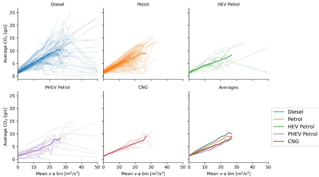
Figure 5.3: CO 2 emissions per v-a bin, per technology type. The bold lines show the averages of all the trips which are shown with the lighter dashed lines. These averages are compared in the bottom-right panel titled 'Averages'.
