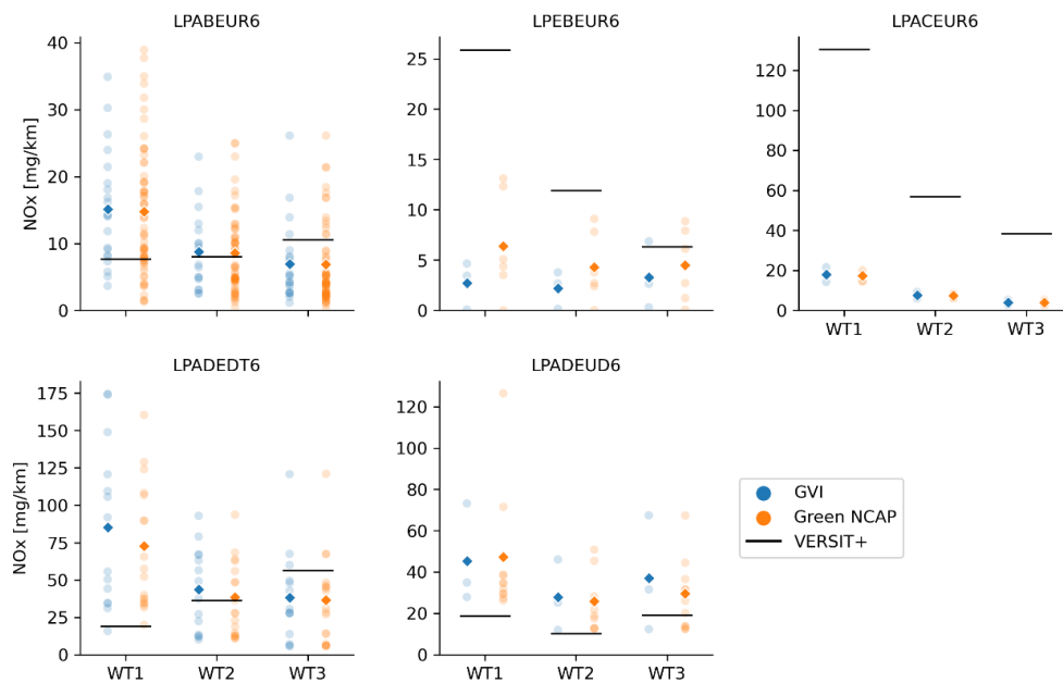
Figure 4.4: Average NO x emissions calculated per urban (WT1), rural (WT2) and motorway (WT3) VERSIT+ road type, as calculated per vehicle (round points) and averaged per GVI or Green NCAP data set (diamond points). Each pane shows the relevant VERSIT+ classes separately. Black lines indicate the corresponding VERSIT+ emission factor.
