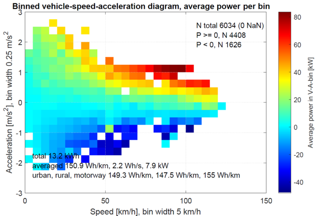
Figure 6.9: Bin-averaged power as function of vehicle speed and acceleration for the VW ID.3 in the on-road ‘PEMS, regular, cold’ test
