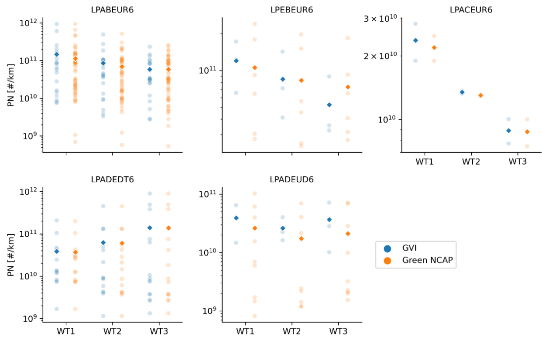
Figure 4.7: Average PN emissions calculated per urban (WT1), rural (WT2) and motorway (WT3) VERSIT+ road type, as calculated per vehicle (round points) and averaged per GVI or Green NCAP data set (diamond points). Each pane shows the relevant VERSIT+ classes separately.
