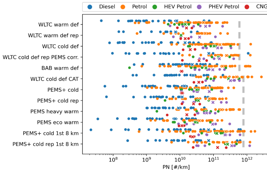
Figure 3.3: PN emissions as averaged over the entire trip. The Green NCAP thresholds are shown in grey. Averages per fuel type per test type are shown by crosses.
