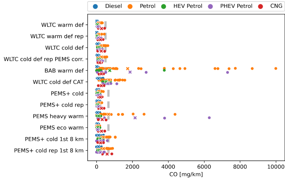
Figure 3.1: CO emissions as averaged over the entire trip. The Green NCAP thresholds are shown in grey. Averages per fuel type per test type are shown by crosses.
