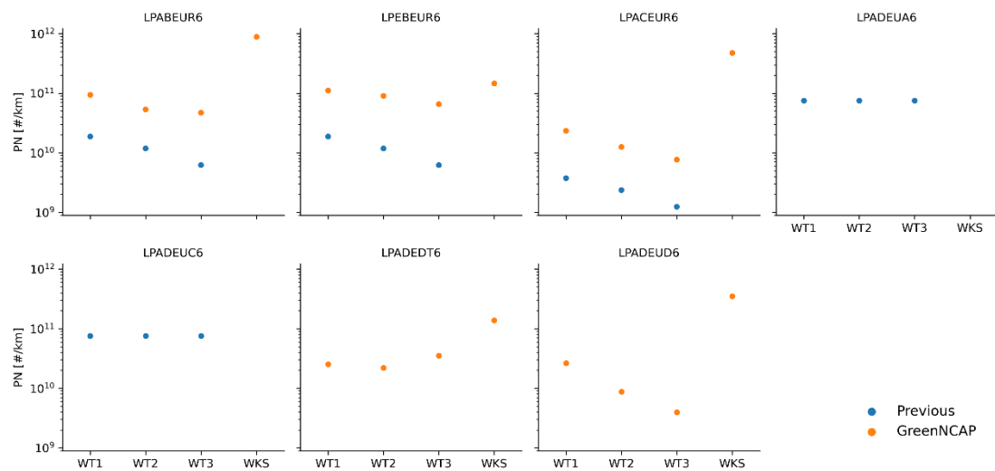
Figure 4.6: Comparison between previously used PN emission factors per road-type as determined from [EMEP/EEA et al. 2013], and those calculated using the Green NCAP data set.
