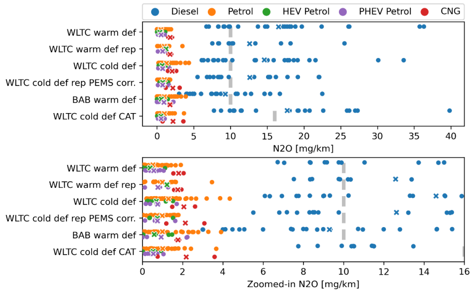
Figure 3.9: N 2 O emissions as averaged over the entire trip. The top panel shows all data measured on the chassis dyno including the Green NCAP thresholds in grey. Averages per fuel type per test type are shown by crosses. The bottom panel shows the zoomed-in version of the top panel.
