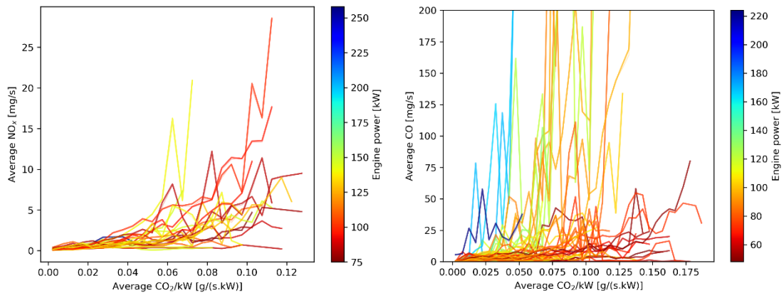
Figure 5.5: (Left) the NO x emissions per diesel vehicle, and (right) CO emissions per petrol vehicle, as a function of CO 2 normalised to the respective vehicle's engine power. Each line represents a different vehicle, and is coloured according to the respective vehicle's engine power.
