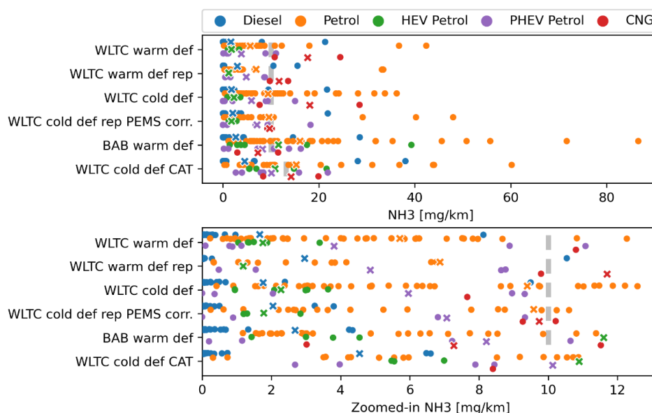
Figure 3.8: NH 3 emissions as averaged over the entire trip. The top panel shows all data measured on the chassis dyno including the Green NCAP thresholds in grey. Averages per fuel type per test type are shown by crosses. The bottom panel shows the zoomed-in version of the top panel.
