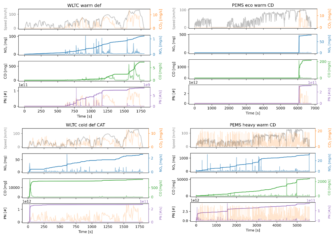
Figure 5.2: Relevant trip details for four different trips driven by E--P_6d_X_132, showing the variation in PN emissions during the trip (lower panel, purple). Per trip, the top panel shows the instantaneous speed in grey, and the CO 2 emissions in orange. The lower three panels show both the cumulative (darker line) and instantaneous (lighter line) emissions for NO x , CO, and PN respectively. The CO 2 emissions shown in the top panel are repeated in the bottom panel to show the correlation between 'engine-on' and PN peaks.
