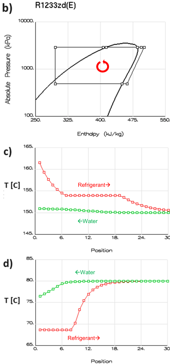
Fig. 12. (a) GUI of the “Working Cycle” feature in IMST-ART, (b) p-h diagram of the HTHP cycle under T_{src} = 80^\circ\text{C} , T_{snk} = 150^\circ\text{C} , and 25 rps, (c) temperature profiles inside the condenser, and (d) temperature profiles inside the evaporator.
