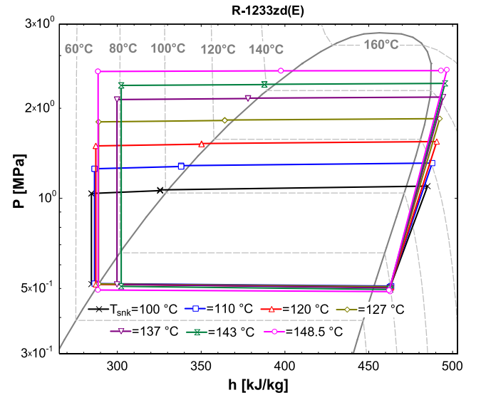
Fig. 5. P-h diagram of the proposed HTHP delivering heat at different sink temperatures under constant T_{w,in,evap} = 80 °C, T_{w,in,subc} = 60 °C, and n_{comp} = 25 rps.
