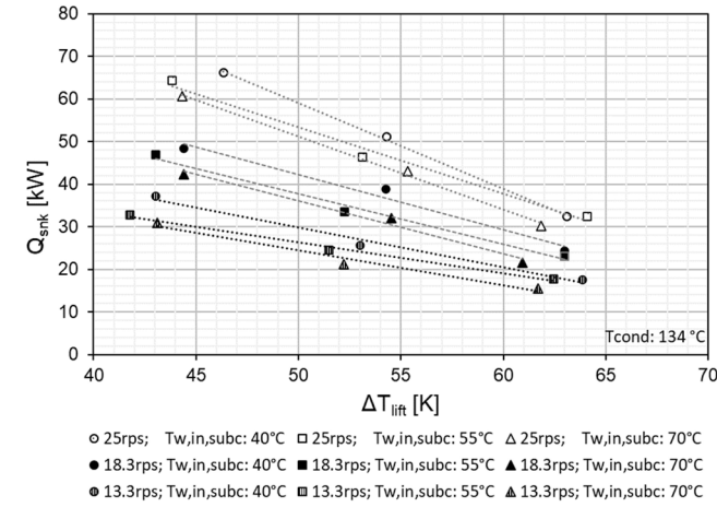
Fig. 4. Total heating capacity ( \dot{Q}_{snk} ) versus the temperature lift for stable condensation temperatures at different compressor speeds and subcooler's water inlet temperatures.
