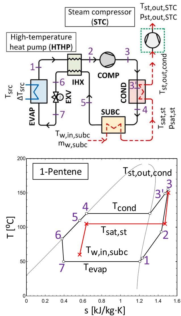
Fig. 1. (up) Proposed steam generation system (HTHP with/without steam compressor), (down) T-s diagram of the proposed HTHP using 1-Pentene.
