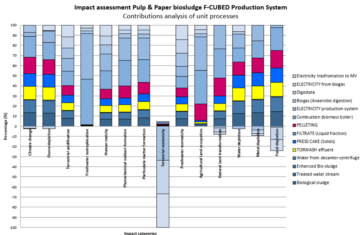
Figure 6. Impact assessment of the F-CUBED Production System for pulp and paper bio-sludge (PPB).
