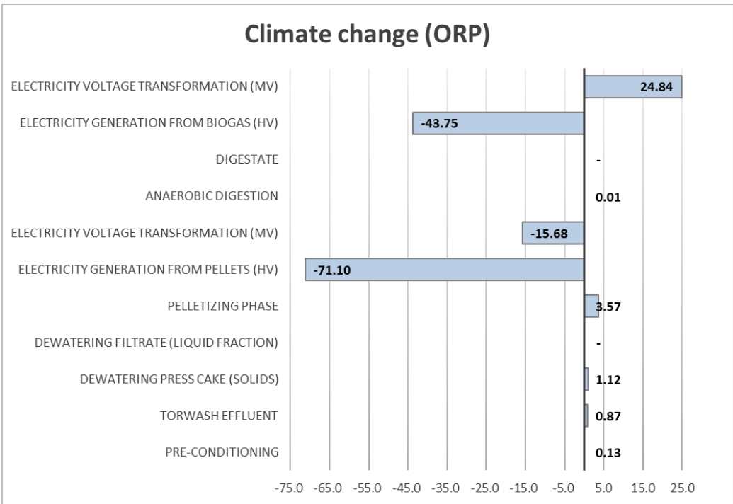
Figure 11. Climate change impact category contribution analysis of the F-CUBED production processes for the ORP case study.
