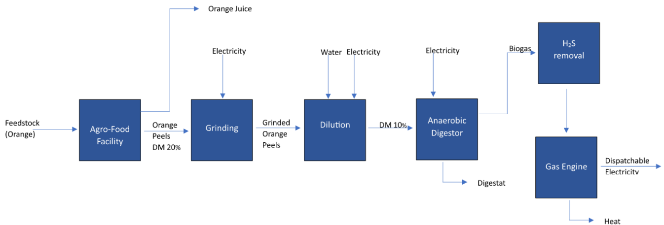
Figure 4. Representation of relevant processes considered as reference cases for fruit and vegetable (orange peel) residues.
