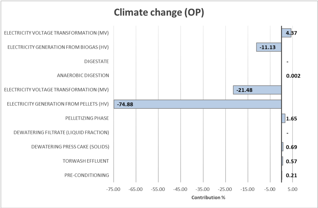
Figure 10. Climate change impact category contribution analysis of the F-CUBED production processes for the OP case study.
