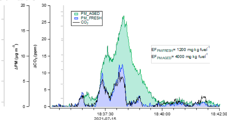
Fig. 2. Example of a ship plume measured in Marseille harbour utilising the Go:PAM OFR. \text{PM}_{\text{AGED}} and \text{PM}_{\text{FRESH}} are the particle mass concentrations measured with and without oxidation of the emissions in the OFR.
