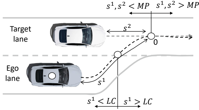
Fig. 1. Set-up of the lane-merging scenario.
