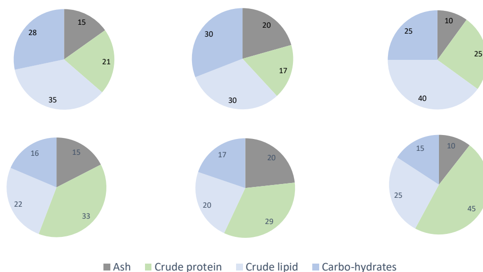
Figure 15 Haematococcus pluvialis green (top) and red (bottom) growing stages composition (ashes, proteins, lipids, and carbohydrates in %wt) at the base, pessimistic and optimistic cases at left, centre and right figure, respectively
