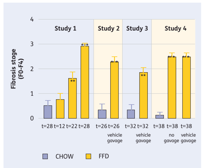
Figure C: Robust induction of fibrosis in Ldlr -/- .Leiden mice
