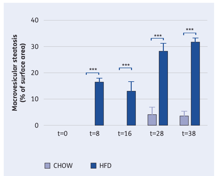
Figure A: Quantification of steatosis in Ldlr -/- .Leiden mice after different periods of HFD feeding
