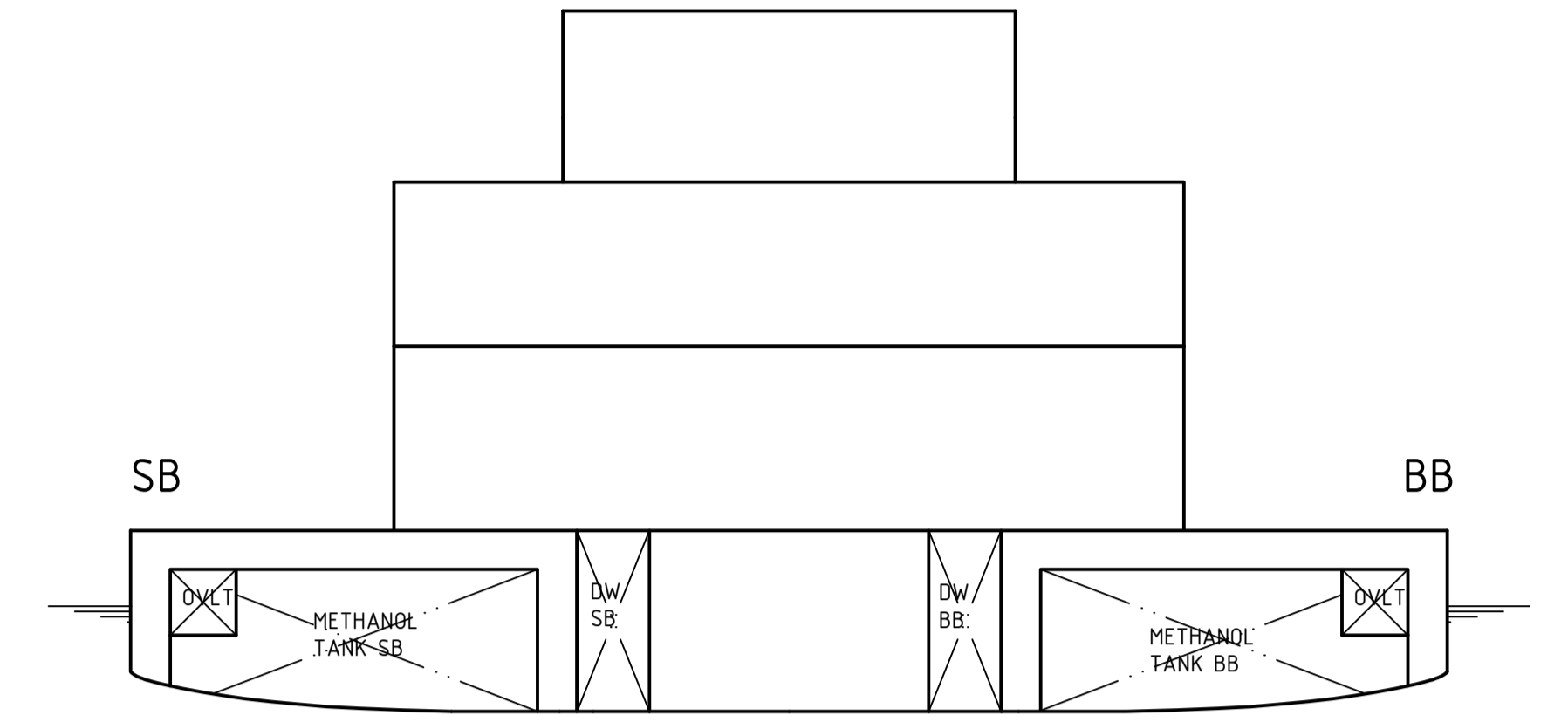
SPANT 67
