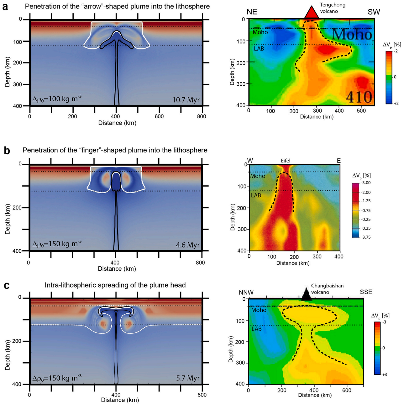
Fig. 3. Comparison of modelled plume-emplacement modes (left panels) with natural examples of seismic velocity anomalies in the upper mantle (right panels). a) Modelled "arrow"-shaped plume vs. asymmetric "arrow" beneath the Tengchong volcano. b) Modelled "finger"-shaped plume vs. columnar structure in sublithospheric and lithospheric mantle below the Eifel volcanic fields. c) Advanced stage of the "finger" scenario with intra-lithospheric spreading of the plume head vs. intra-lithospheric "mushroom" underlying the Changbaishan volcanic area. (Modified after Cloetingh et al., 2022.)
