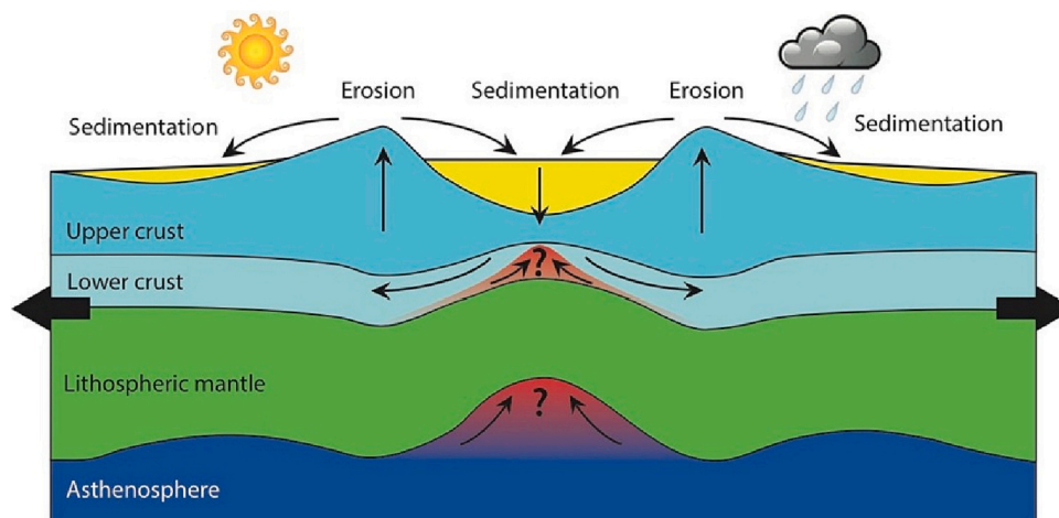
Fig. 14. Schematic representation of the interactions between surface processes and magmatism in an extensional setting (not to scale, modified after Burov and Cloetingh, 1997 ; Sternai, 2020 ). Sediments derived from erosion of rift shoulders load the rift basins. The rigid upper crust and lithospheric mantle flex and weaken, while more ductile lower-crustal material flows from the centre of the rift outward, facilitating uplift and erosion of the rift shoulders. The associated effects on extensional magmatism (reddish material) are to date poorly constrained and represent a promising emerging research field.
