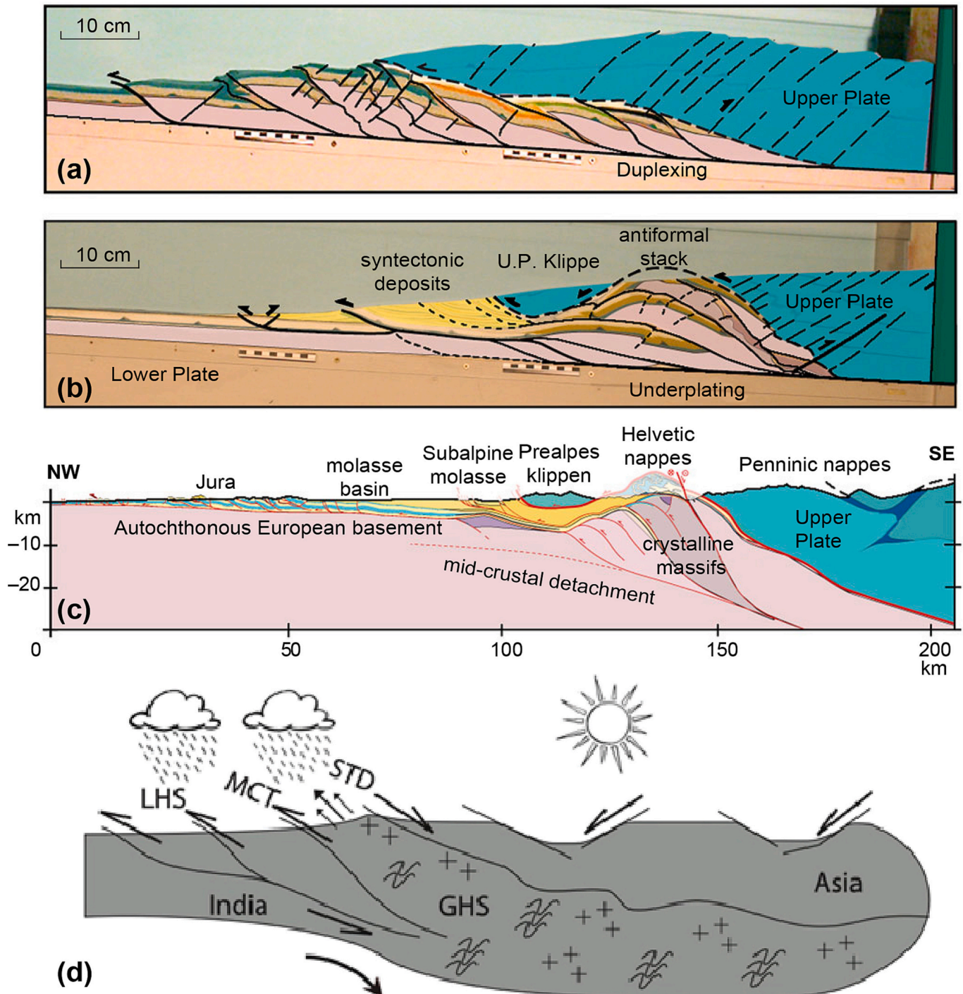
Fig. 6. (a) Analogue models of crustal convergence and orogenic wedge evolution without (a) and with (b) erosion and syntectonic sedimentation (Malavielle and Konstantinovskaya, 2010). Modelling results are compared to a classical cross section of the Swiss Alps (c) from Burkhard and Sommaruga, 1998. (d) Crustal tectonic framework of the Himalaya and Southern Tibet where erosion at the mountain front contributes to localized exhumation of weak lower crustal material (e.g., Wu et al., 1998; Burchfiel et al., 1992; Beaumont et al., 2001). LHS, Lesser Himalayan sequence; MCT, Main Central Thrust; STD, South Tibetan Detachment; GHS, Greater Himalayan Sequence.
