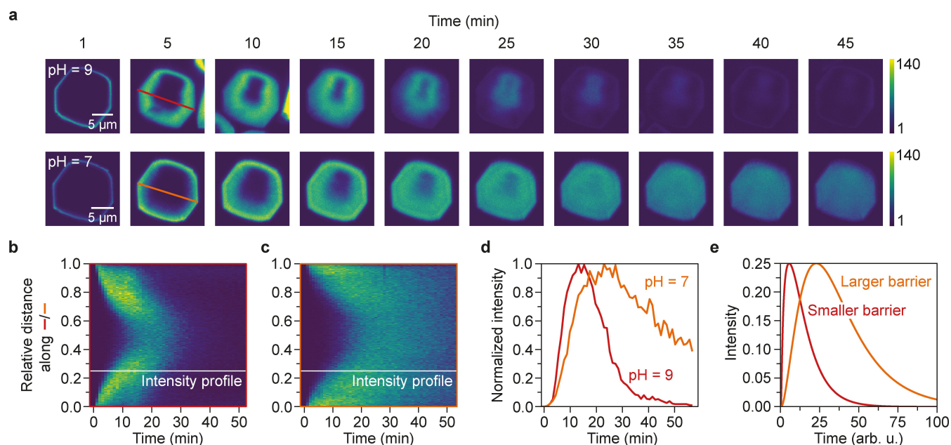
Figure 5. a) Confocal laser scanning microscopy micrographs of H-zeolite-β crystals incubated in water followed by incubation in 50 μM resorufin at two external pH values ( \lambda_{\text{ex}} = 493 nm) starting at time = 0. Kymographs along the red (b; pH 9) and orange (c; pH 7) solid lines marked in (a). d) Intensity profile at 25% of the relative position (white lines in b and c) under pH 9 and 7 conditions. e) Simulated intensity profile at 25% of the relative position of protonated resorufin corrected for J-aggregation computed with a 1D diffusion model that accounts for a diffusion barrier.
